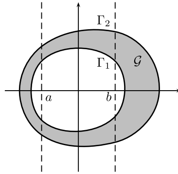
Fig. 11. Relative positions between \Gamma_1 and \Gamma_2 .
