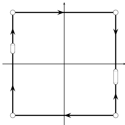
Fig. 5. An example of a phase portrait on the boundary. The rounded regions represent the set of singular points.
