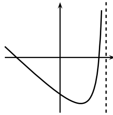
Fig. 3. A mixed function f(x) .
