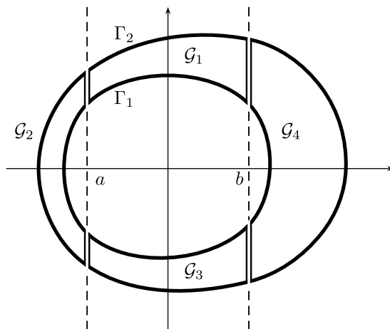
Fig. 12. Decomposition of \mathcal{G} .
