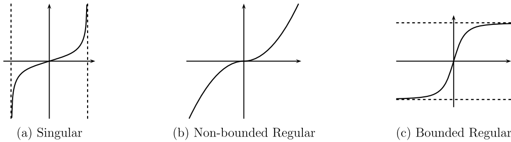
Fig. 1. Basic \varphi functions.
