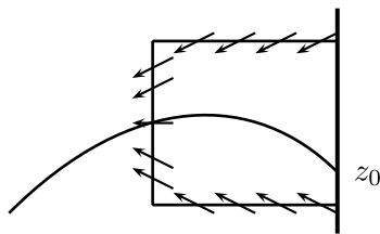
Fig. 8. Behavior of the flux near to an isolated singular point in the boundary.
