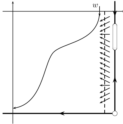
Fig. 7. Phase portrait of system (7) on the fourth quadrant.
