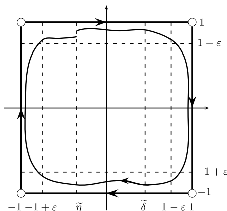
Fig. 10. Phase portrait of \Gamma_{\zeta_0} .
