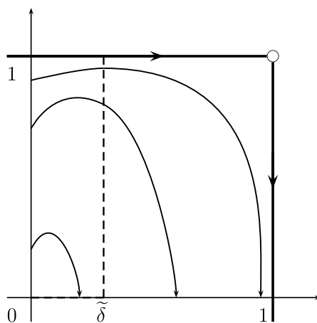
Fig. 6. Phase portrait of system (7) for the first quadrant.
