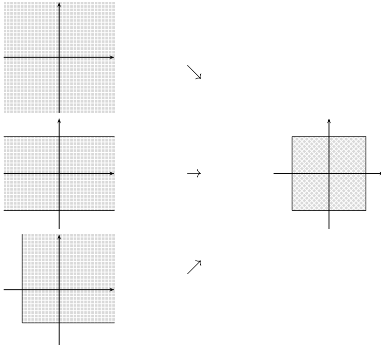
Fig. 4. Examples of compactified boundaries.
