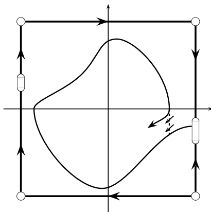
Fig. 9. Positively invariant region when the boundary has singular points different from the vertex.
