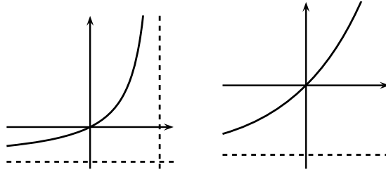
Fig. 2. Examples of mixed behavior at the boundary of the domain.
