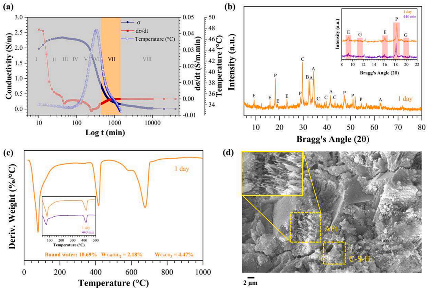
Fig. 10. Region VII at 1 day of hydration (a) Conductivity ( \sigma ), derivative ( d\sigma/dt ) and internal temperature of cement paste in function of log t; (b) XRD diffractogram (A: Alite, C_3S ; B: Belite, C_2S ; C: Calcite, CaCO_3 ; E: Ettringite, AFt; P: Calcium hydroxide; Ca(OH)_2 ); (c) DTG curve and (d) SEM image.
