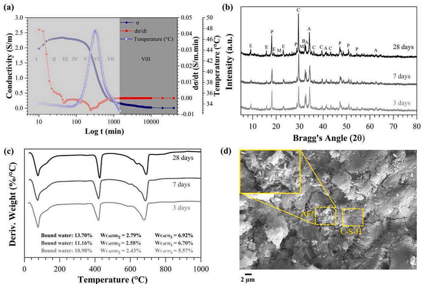
Fig. 11. Region VIII at 3, 7, and 28 days of hydration (a) Conductivity ( \sigma ), derivative ( d\sigma/dt ) and internal temperature of cement paste in function of \log t ; (b) XRD diffractogram (A: Alite, \text{C}_3\text{S} ; B: Belite, \text{C}_2\text{S} ; C: Calcite, \text{CaCO}_3 ; E: Ettringite, AFm; Monosulfate, AFm; P: Calcium hydroxide; \text{Ca}(\text{OH})_2 ); (c) DTG curve and (d) SEM image.
