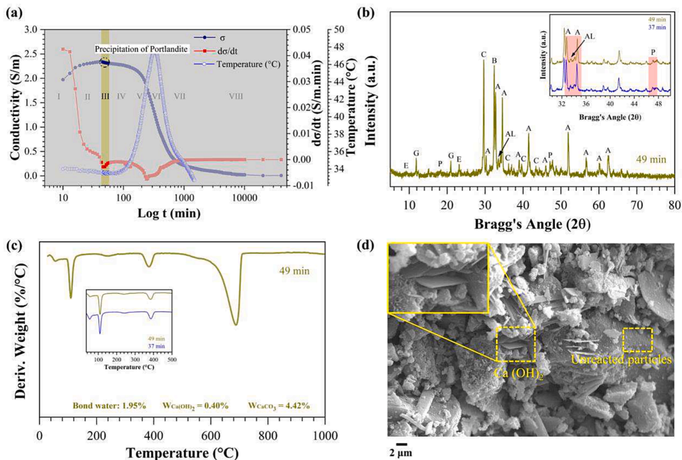
Fig. 6. Region III at 49 min of hydration (a) Conductivity ( \sigma ), derivative ( d\sigma/dt ) and internal temperature of cement paste in function of log t; (b) XRD diffractogram (A: Alite, C_3S ; AL: Tricalcium aluminate, C_3A ; B: Belite, C_2S ; C: Calcite, CaCO_3 ; E: Ettringite, Aft; G: Calcium sulfate dihydrate, CaSO_4 \cdot 2H_2O ; P: Calcium hydroxide; Ca(OH)_2 ); (c) DTG curve and (d) SEM image.
