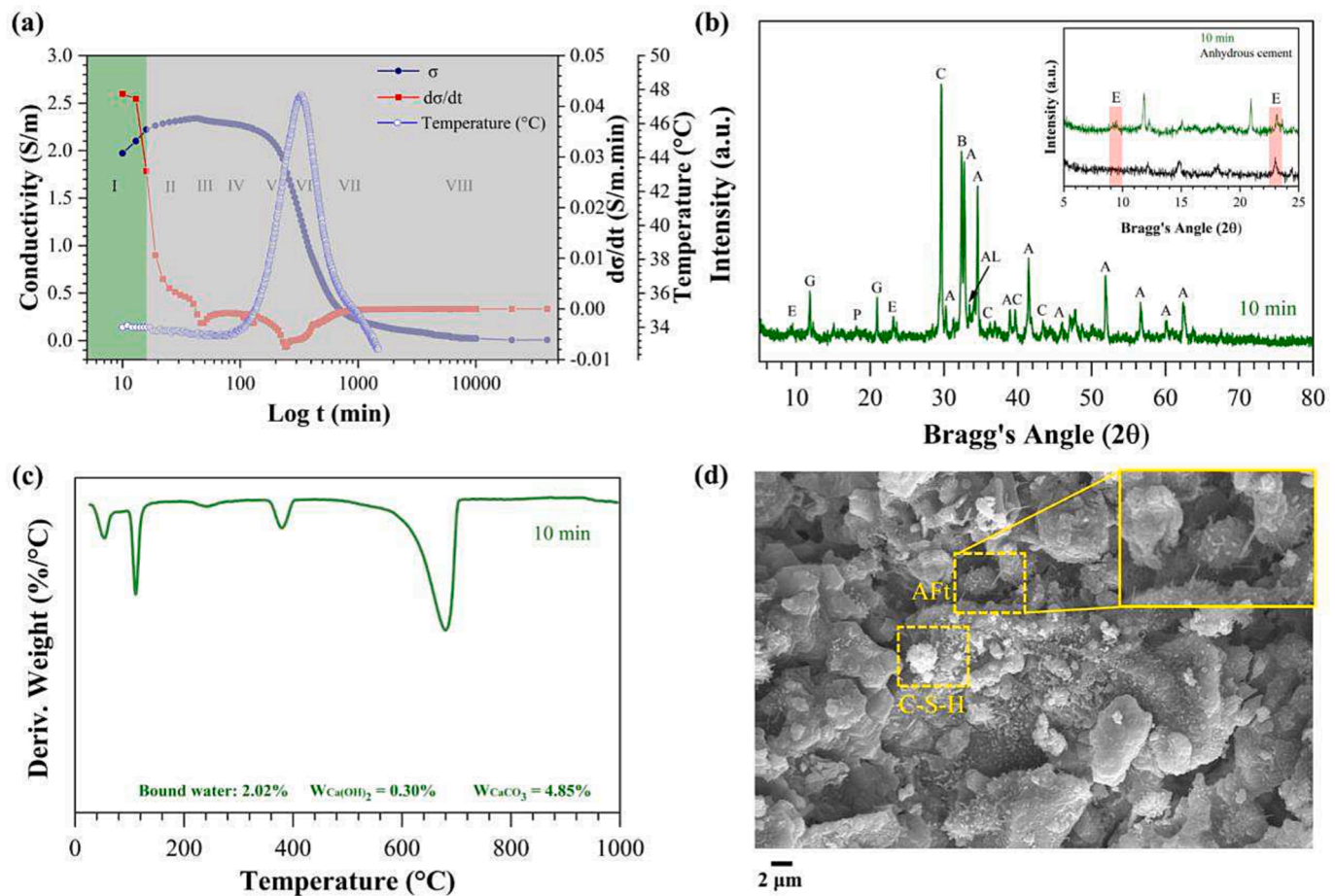
Fig. 4. Region I at 10 min of hydration (a) Conductivity ( \sigma ), derivative ( d\sigma/dt ) and internal temperature of cement paste in function of log t; (b) XRD diffractogram (A: Alite, C_3S ; AL: Tricalcium aluminate, C_3A ; B: Belite, C_2S ; C: Calcite, CaCO_3 ; E: Ettringite, Aft; G: Calcium sulfate dihydrate, CaSO_4 \cdot 2H_2O ; P: Calcium hydroxide; Ca(OH)_2 ); (c) DTG curve and (d) SEM image.
