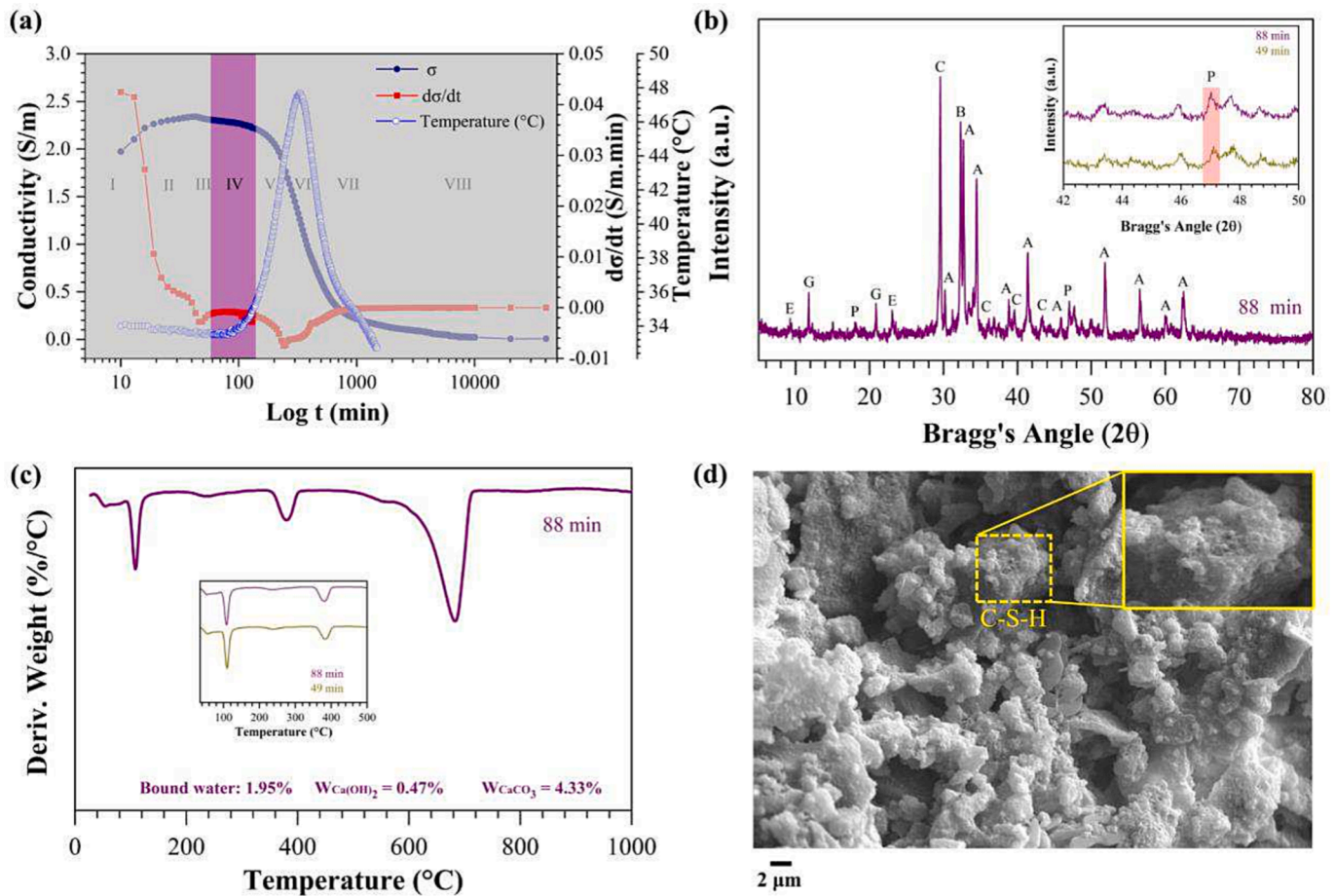
Fig. 7. Region IV at 88 min of hydration (a) Conductivity ( \sigma ), derivative ( d\sigma/dt ) and internal temperature of cement paste in function of \log t ; (b) XRD diffractogram (A: Alite, C_3S ; B: Belite, C_2S ; C: Calcite, CaCO_3 ; E: Ettringite, AfT ; G: Calcium sulfate dihydrate, CaSO_4 \cdot 2H_2O ; P: Calcium hydroxide; Ca(OH)_2 ); (c) DTG curve and (d) SEM image.
