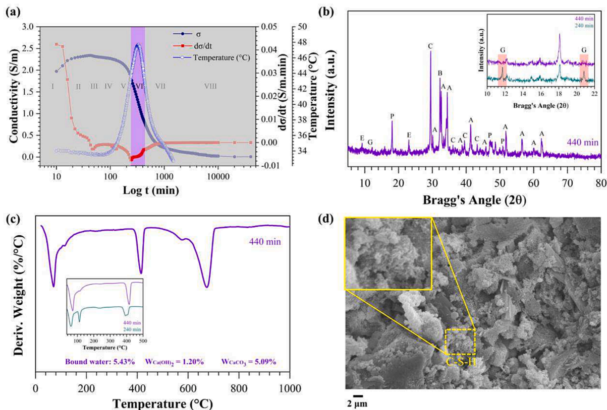
Fig. 9. Region VI at 440 min of hydration (a) Conductivity ( \sigma ), derivative ( d\sigma/dt ) and internal temperature of cement paste in function of log t; (b) XRD diffractogram (A: Alite, \text{C}_3\text{S} ; B: Belite, \text{C}_2\text{S} ; C: Calcite, \text{CaCO}_3 ; E: Ettringite, \text{AFt} ; G: Calcium sulfate dihydrate, \text{CaSO}_4 \cdot 2\text{H}_2\text{O} ; P: Calcium hydroxide, \text{Ca(OH)}_2 ); (c) DTG curve and (d) SEM image.
