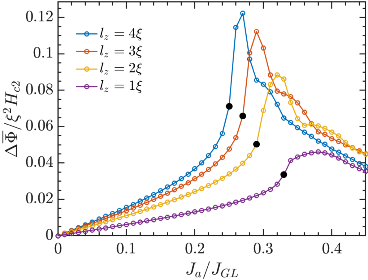
Figure 10 – Difference between the average magnetic flux on both sides of the sample through two vertical circuits positioned on the planes y = \pm(l_y/2 + \xi) . The domain of the circuits is given by \{-\xi \leq x \leq \xi, -l_z/2 \leq z \leq L_z/2\} . The value of L_z was chosen such that the area of the circuit above the z = l_z/2 surface is the same for all thicknesses l_z . The points just before the onset of the resistive state are highlighted in black.
