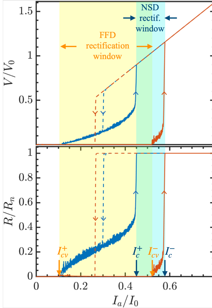
Figure 10 – Top panel shows |V(t)| as a function of |I_a(t)| . Blue and red curves represent the half period with positive and negative J_a(t) , respectively. Solid and dashed lines represent the regions where |I_a(t)| is being increased and decreased, respectively. Yellow and blue background marks the current region of vortex and diode rectification, with green background depicting the region where they coexist. Bottom panel shows R(t) as a function of |I_a(t)| , with the same definitions of the top panel following.
