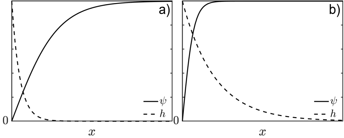
Figure 2 – Profile of the order parameter (solid line) and local magnetic field (dashed line) for \kappa \ll 1 (panel a)) and for \kappa \gg 1 (panel b)).
