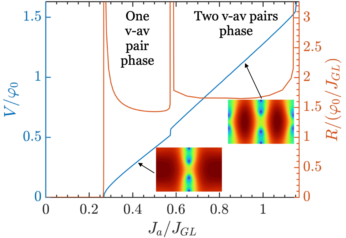
Figure 7 – IV (blue line) and IR (red line) characteristic curves, respectively, for \kappa = 1 and l_z = 3\xi . The Meissner state (full superconductivity) survives up to J_a = J_{c1} = 0.27J_{GL} . Above this current density, the resistive state sets in. The resistive state splits into two phases. In one of them the vortex and the antivortex nucleate only at the defects on the border of the superconductor. In the second phase, another set of v-av pairs nucleates at the frontiers between unit cells. The second jump in the IV characteristic is the signature of this crossover. The insets illustrate this scenario through the modulus of the order parameter in the xy plane ( z = 0 plane).
