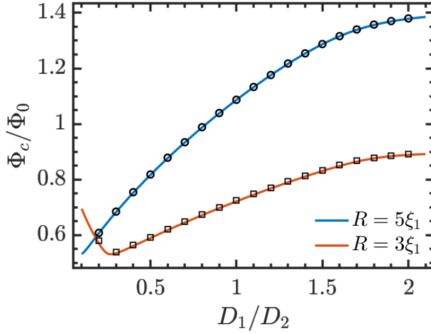
Figure 5 – Critical flux above which the Meissner state becomes unstable as a function of the ratio D_1/D_2 . The blue (red) line presents the results obtained from our method developed in Section 5.2 for a ring with radius R = 5\xi_1 ( R = 3\xi_1 ). Black circles (squares) show the values of the critical flux obtained numerically directly from the TDGL.
