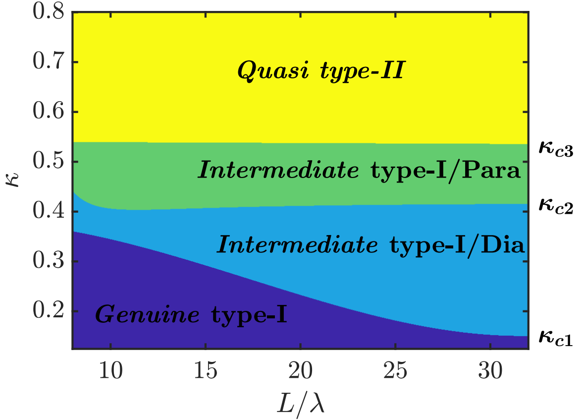
Figure 6 – \kappa - L phase diagram for the three transitions discussed above. Each color represent a different type of behavior presented by the system. The limiting curves were obtained by the adjusting the critical values of \kappa found in the simulations.
