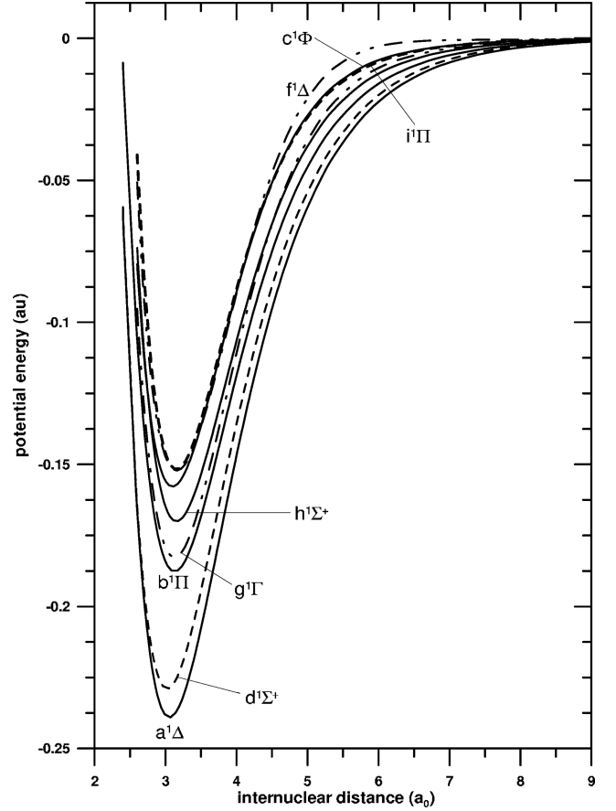
Figure 2. Potential energy curves for the lowest lying singlet states of the TiO molecule.
