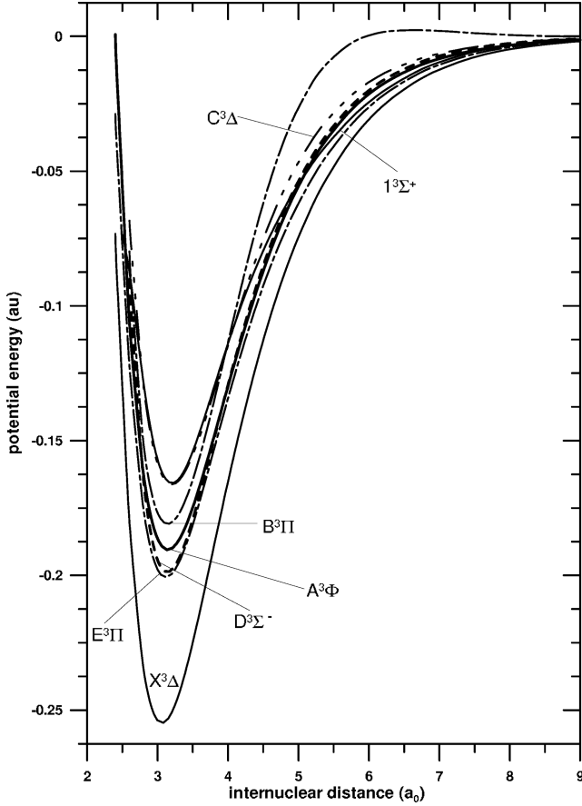
Figure 1. Potential energy curves for the lowest lying triplet states of the TiO molecule.
