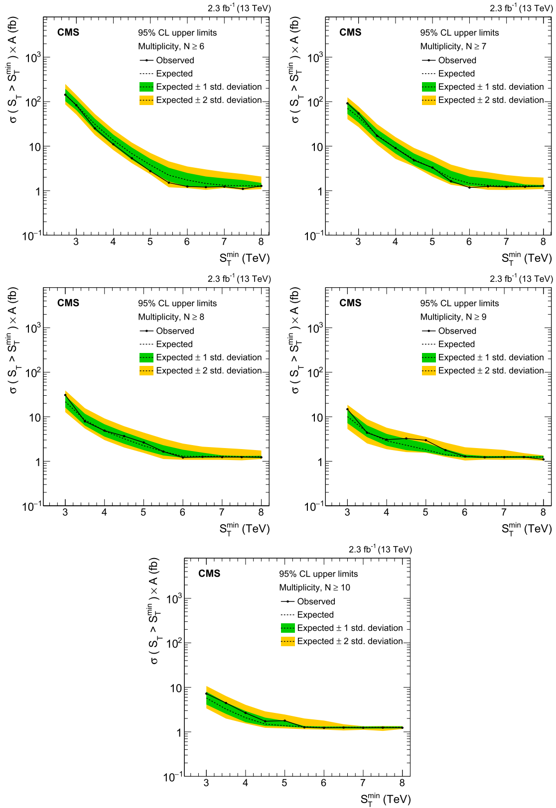
Fig. 5. Model-independent 95% CL upper limits on the cross section times acceptance for five sets of inclusive multiplicity thresholds: N \geq 6, 7, 8, 9 , and 10 . Observed (expected) limits are shown as a solid (dashed) lines, and the two bands correspond to \pm 1 and 2 standard deviations in the expected limit.
