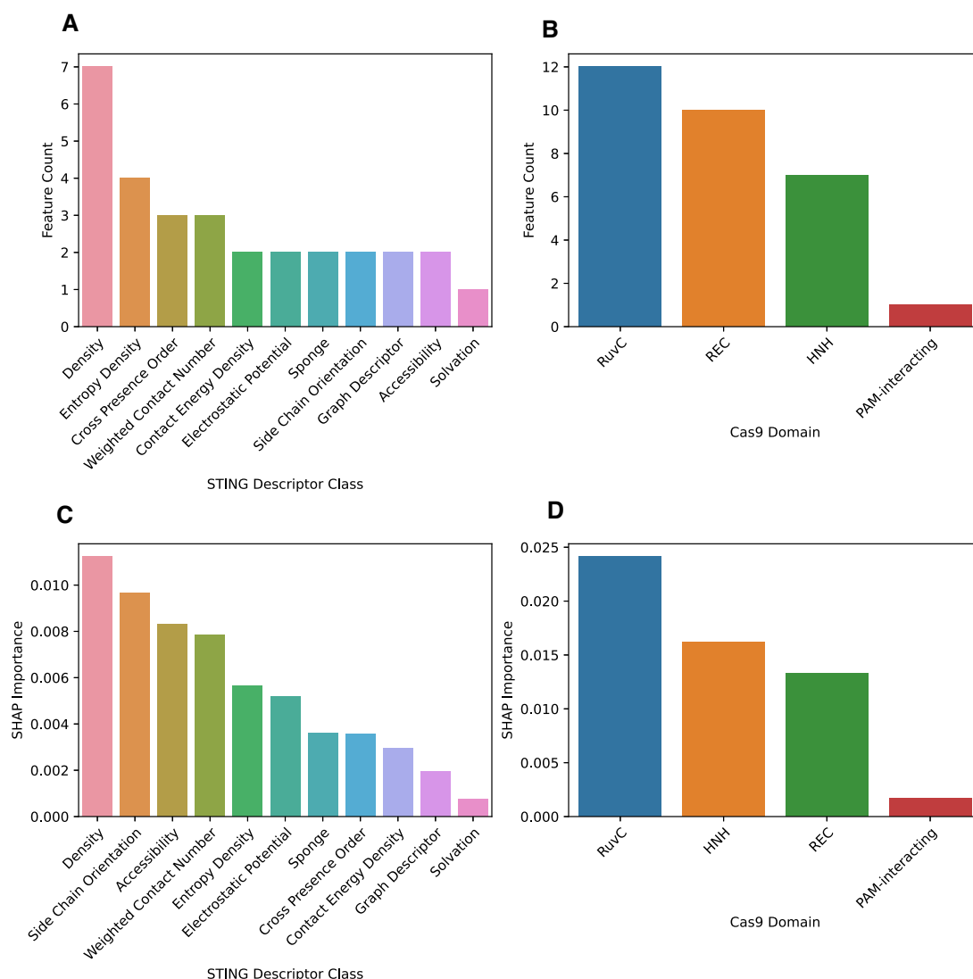
Figure 6. (Top) STING_CRISPR's feature counts categorized by STING descriptor classes (A) and CRISPR–Cas9 domains (B), respectively, sorted by decreasing count. (Bottom) STING_CRISPR's SHAP importance values for STING descriptor classes (C) and CRISPR–Cas9 domains (D), respectively, sorted by decreasing SHAP importance. Only STING descriptor classes or Cas9 domains with non-zero count or SHAP importance are shown.
