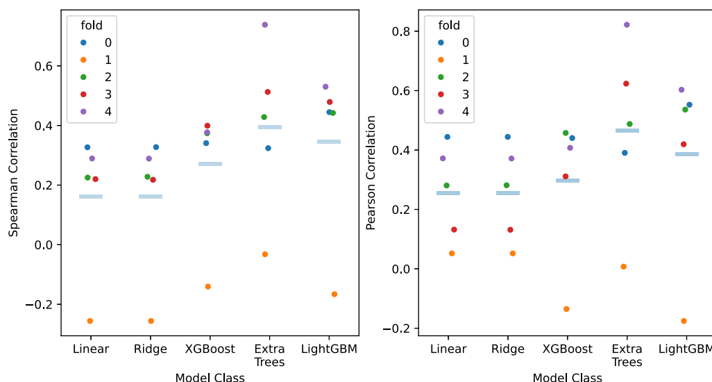
Figure 7. Five-fold cross-validation Spearman (left) and Pearson (right) correlation performance when using linear regression, ridge regression, XGBoost, extra trees, and LightGBM. Test sets for each cross-validation fold was constructed by binning snapshots associated with the trajectory with the n th lowest cleavage activity into the test partition of fold n \bmod 5 , and into the training partition in the other folds. Light blue horizontal line represents the mean correlation across the five folds.
