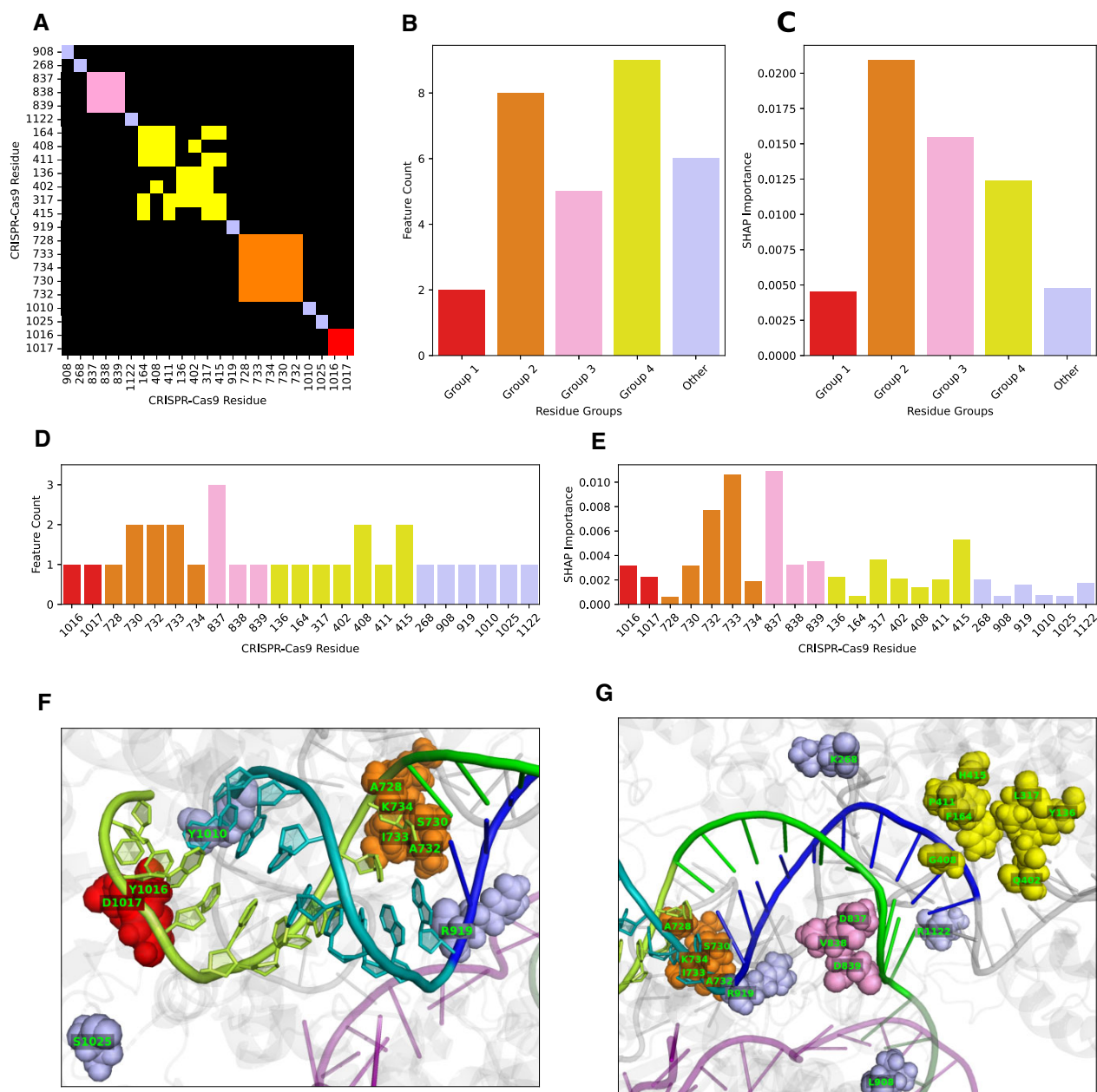
Figure 5. The ML pipeline identifies four residue clusters, namely Group 1 (residues 1016/1017, coloured red), Group 2 (residues 728/730/732–734, coloured orange), Group 3 (residues 837–839, coloured pink), and Group 4 (residues 136/164/317/402/408/411/415, coloured yellow). The fifth group ‘other’ consists of residues identified by the pipeline that do not belong to the above clusters (residues 268/908/919/1010/1015/1122, coloured light blue). (A) Binarized hierarchically clustered heatmap for the 23 Cas9 residues identified by the ML pipeline. Heatmap cells for residue pairs whose C_{\alpha} atoms are <12 Å apart are coloured according to their associated residue groups, and black otherwise. Feature counts (B) and SHAP importances (C) of the five residue groups. Feature counts (D) and SHAP importances (E) of the 23 important Cas9 residues, with residues grouped and coloured by the five residue groups. PyMOL cartoon visualization of the PAM-distal (F) and PAM-proximal (G) portions of the sgRNA–dsDNA heteroduplex taken from the last (i.e. 24th) snapshot of CMUT1’s MD trajectory. Shown as labelled spheres, the 23 CRISPR–Cas9 important residues are coloured by their residue groups. Shown as ribbons, the colour scheme of other components is as follows: other parts of Cas9 = grey, PAM-distal sgRNA = teal, PAM-proximal sgRNA = blue, PAM-distal target DNA strand = limon, PAM-proximal target DNA strand = green, and non-target DNA strand = transparent purple.
