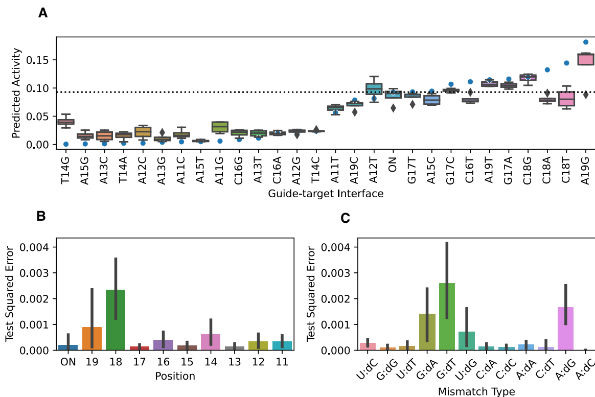
Figure 3. Test performance of STING_CRISPR. (A) STING_CRISPR's predicted cleavage activities for the hold-out test set containing the last 4 snapshots from each of the 28 MD trajectories. Blue dots indicate experimental cleavage activity labels for the 28 interfaces. Guide-target interfaces listed on the x-axis are sorted by increasing experimental activity. ON = on-target interface. (B) STING_CRISPR's squared error between predicted and actual CRISPR–Cas9 cleavage activity values for snapshots in the test set, categorized by being an on-target interface or a PAM-distal mismatch position. (C) STING_CRISPR's test squared error between predicted and actual CRISPR–Cas9 cleavage activity values for the different off-target mismatch interface types.
