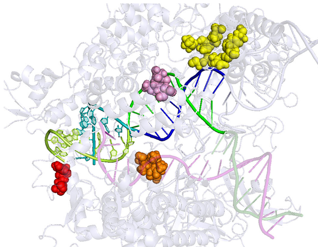
Figure 4. PyMOL cartoon visualization of the sgRNA-dsDNA-Cas9 complex, taken from the last (i.e. 24th) snapshot of CMUT1's MD trajectory. Shown as spheres, the four CRISPR-Cas9 residue clusters 136/164/317/402/408/411/415, 728/730/732-734, 837-839, and 1016/1017 are highlighted in yellow (top right), orange (center bottom), pink (center top), and red (bottom left), respectively. Other parts of the Cas9 are visualized as grey ribbons. Shown as ribbons, the colour scheme is as follows for non-Cas9 components: PAM-distal sgRNA = teal, PAM-proximal sgRNA = blue, PAM-distal target DNA strand = limon, PAM-proximal target DNA strand = green, and non-target DNA strand = transparent purple.
