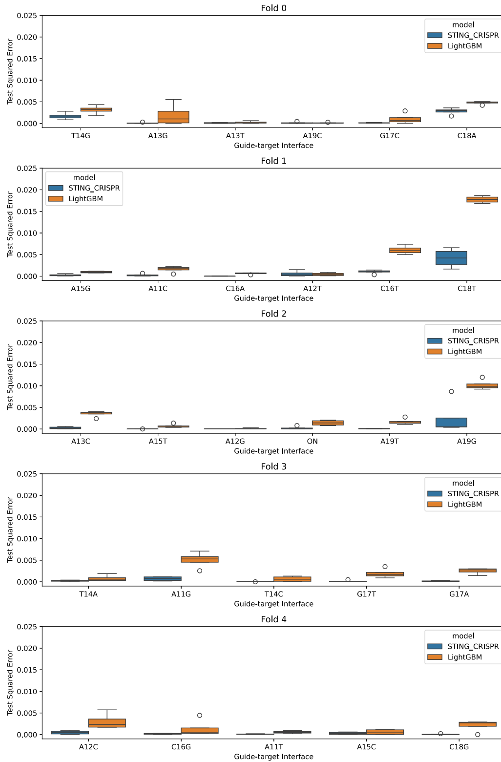
Figure 8. Box plots comparing test squared errors between STING_CRISPR and the new LightGBM model trained in Fig. 7. The x-axis lists the guide–target interfaces held-out in each of the five cross-validation folds. Circles represent outliers in the box plot.
