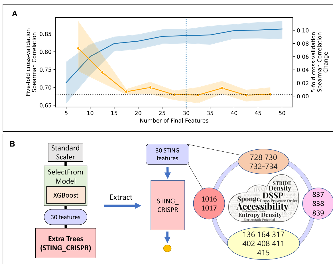
Figure 2. STING_CRISPR is an extra trees model with 30 STING features at 4 residue clusters. (A) Hyperparameter tuning of input feature set size in the ML pipeline after grid search with five-fold cross-validation. The solid rising blue line (left y-axis) indicates average five-fold Spearman test correlation, and the solid falling orange line (right y-axis) indicates average change in the average five-fold test Spearman correlation when increasing the input feature set size in increments of 5. Black dotted horizontal line indicates the Spearman change threshold \Delta\rho_S = 0.002 , and the blue dotted vertical line indicates the final input feature size selected. (B) Extraction of the second ML model (left bottom red box with bolded text) from the hyperparameter-optimized ML pipeline with m_1 = \text{XGBoost} , m_2 = \text{extra trees} , and f = 30 features yields STING_CRISPR, an extra trees model with 30 STING features. Among the 30 STING features, 17 of them form 4 residue clusters (defined below) found to be important in cleavage activity prediction for the studied sgRNA-tsDNA pairs.
