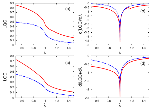
FIG. 2: Two-spin local \sigma_x -coherence for \gamma = 0.5 (a) and \gamma = 1 (c), along with its first derivative (with respect to \lambda ) for \gamma = 0.5 (b) and \gamma = 1 (d), as a function of \lambda . As the red solid line denotes the measure, the dashed blue line corresponds to its simplified version.
