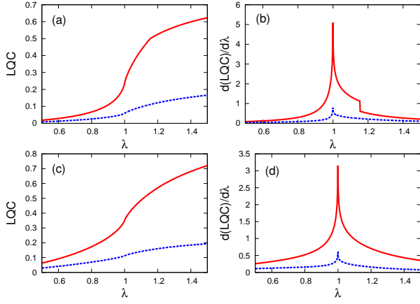
FIG. 3: Two-spin local \sigma_z -coherence for \gamma = 0.5 (a) and \gamma = 1 (c), along with its first derivative (with respect to \lambda ) for \gamma = 0.5 (b) and \gamma = 1 (d), as a function of \lambda . As the red solid line denotes the measure, the dashed blue line corresponds to its simplified version.
