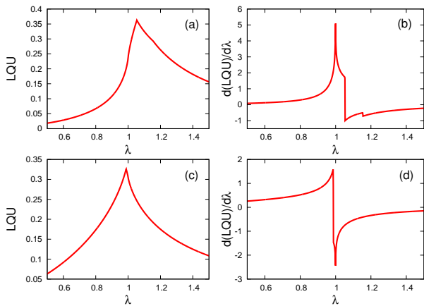
FIG. 5: Two-spin local quantum uncertainty for \gamma = 0.5 (a) and \gamma = 1 (c), along with its first derivative (with respect to \lambda ) for \gamma = 0.5 (b) and \gamma = 1 (d), as a function of \lambda .
