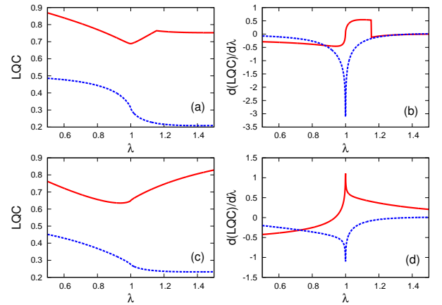
FIG. 4: Two-spin local \sigma_y -coherence for \gamma = 0.5 (a) and \gamma = 1 (c), along with its first derivative (with respect to \lambda ) for \gamma = 0.5 (b) and \gamma = 1 (d), as a function of \lambda . As the red solid line denotes the measure, the dashed blue line corresponds to its simplified version.
