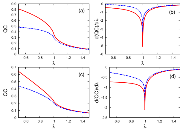
FIG. 1: Single-spin \sigma_x -coherence for \gamma = 0.5 (a) and \gamma = 1 (c), along with its first derivative (with respect to \lambda ) for \gamma = 0.5 (b) and \gamma = 1 (d), as a function of \lambda . As the red solid line denotes the measure, the dashed blue line corresponds to its simplified version.
