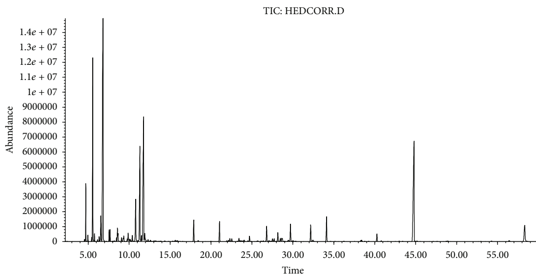
FIGURE 2: Chromatogram of Hedychium coronarium rhizomes essential oil (SBP-1 column).
