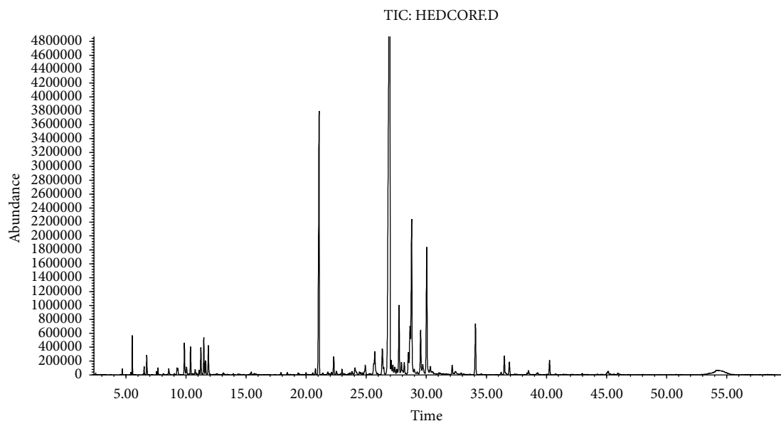
FIGURE 1: Chromatogram of Hedychium coronarium leaves essential oil (SBP-1 column).
