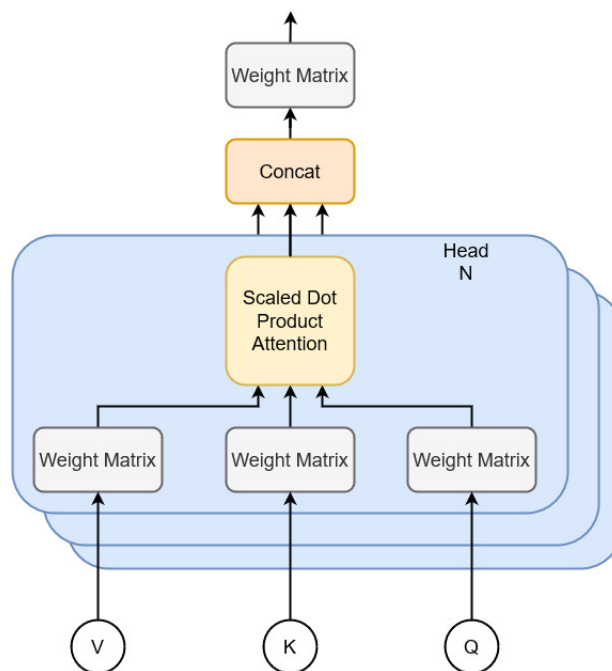
Figura 11 – Função Multi-Head Attention
