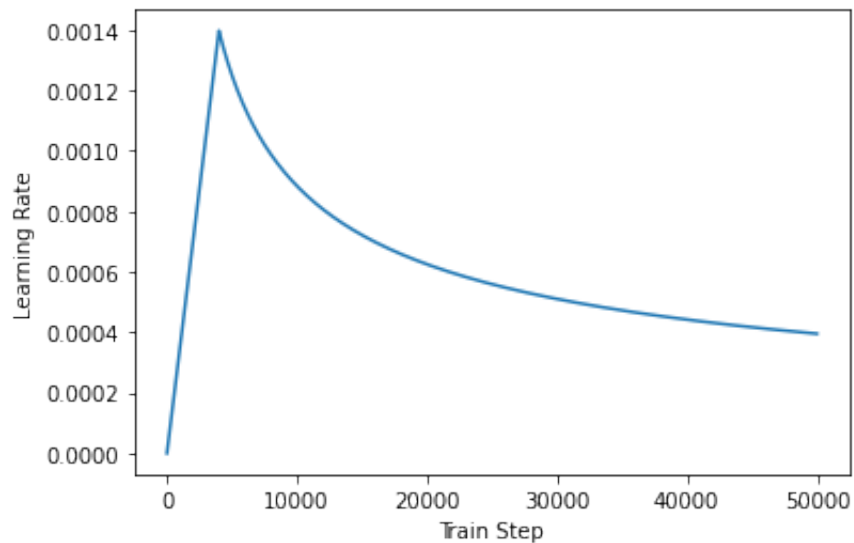
Figura 14 – Learning Rate
