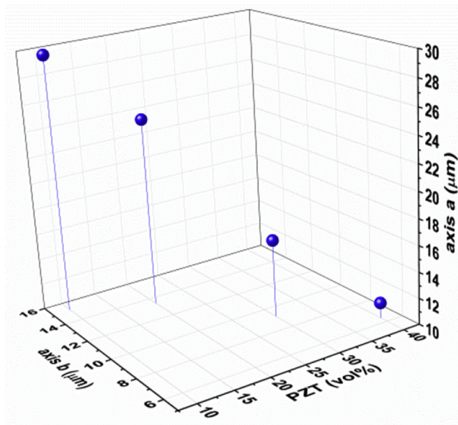
Fig. 2. Mean values of CB agglomerate size as a function of the PZT vol% for 25%vol CB.
