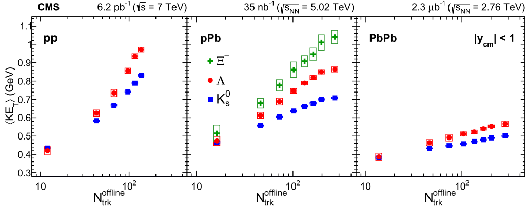
Fig. 6. The average transverse kinetic energy, \langle KE_T \rangle , at |y_{cm}| < 1 for K_S^0 , \Lambda , and \Xi^- particles as a function of multiplicity in pp, pPb, and PbPb collisions. The inclusion of the charge-conjugate states is implied for \Lambda and \Xi^- particles. For the \Xi^- , only results from pPb collisions are shown. The error bars represent the statistical uncertainties, while the boxes indicate the systematic uncertainties.
