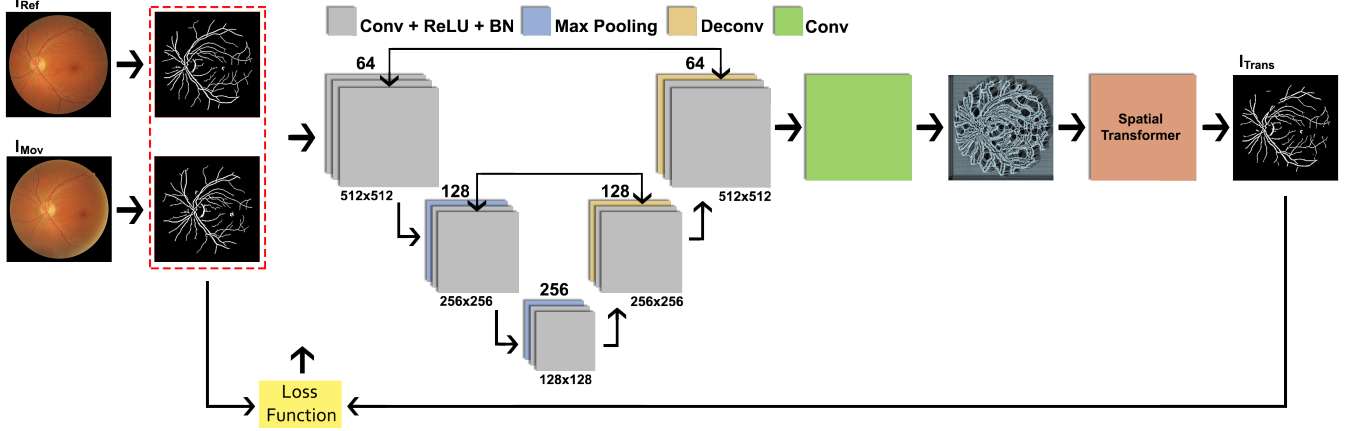
Fig. 1. Pipeline overview of the proposed unsupervised learning framework.
