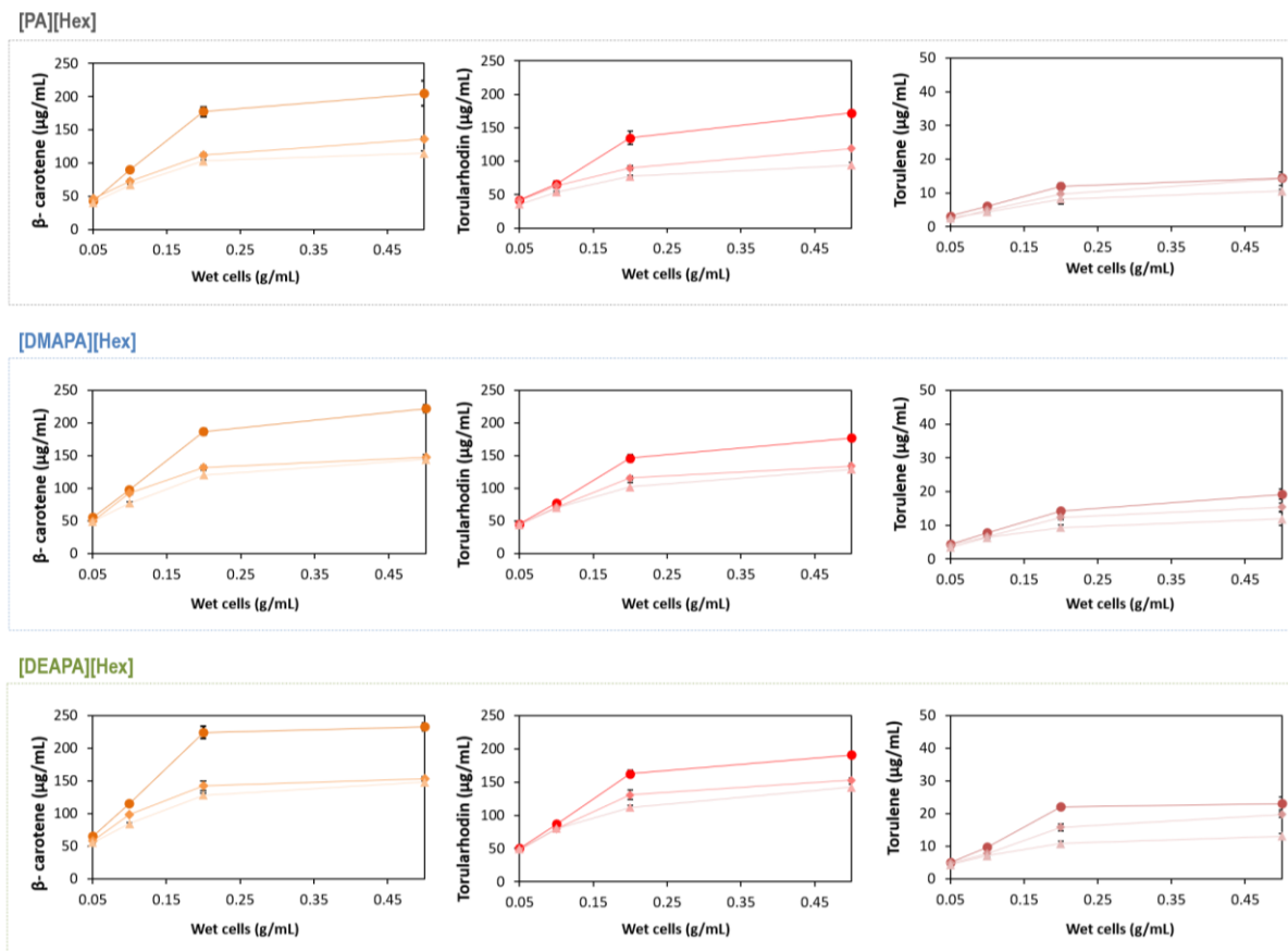
Figure 4.6. Effect of the temperature [(triangle) 25 °C, (diamond) 45 °C, and (circle) 65 °C] as a function of solid-liquid ratio, SLR (0.05, 0.1, 0.2, and 0.5 g/mL wet cells), on the release of β-carotene, torularhodin, and torulene using different solutions of PILs at 90% (v/v) after 1 h of stirring (30 rpm). The error bars represent 95% confidence levels for the mean of three independent assays, but in some cases, they are smaller than the markers.
