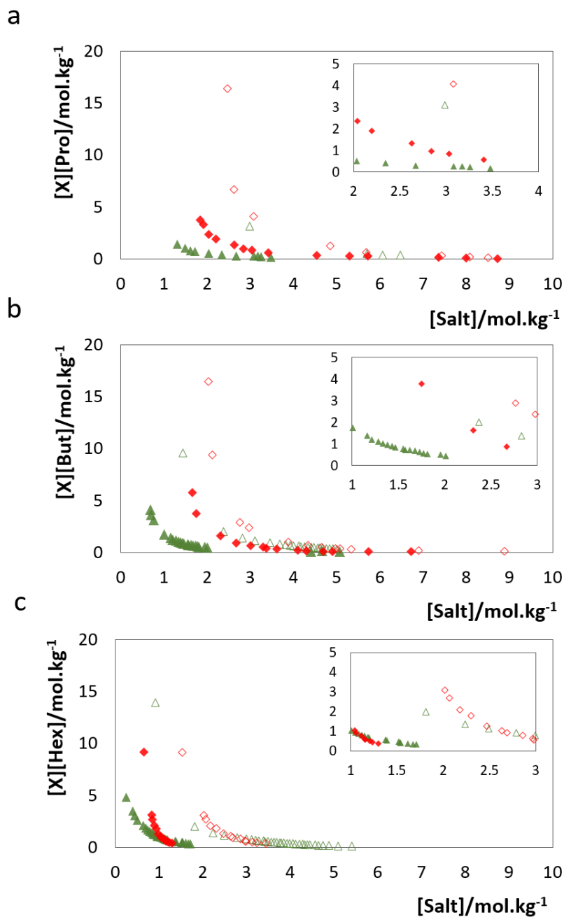
Figure 5.3. Ternary phase diagrams of the systems a) [X][\text{Pro}] + \text{salt} + \text{H}_2\text{O} , b): [X][\text{But}] + \text{salt} + \text{H}_2\text{O} and c) [X][\text{Hex}] + \text{salt} + \text{H}_2\text{O} determined at 298 (\pm 1) \text{ K} and atmospheric pressure. The experimental binodal curves of the systems composed of \text{K}_3\text{PO}_4 are represented by full symbols, and \text{K}_2\text{HPO}_4 by open symbols. [X] corresponds to [\text{DEAPA}]^+ (green triangle) or [\text{DMAPA}]^+ (red diamond) cation.
