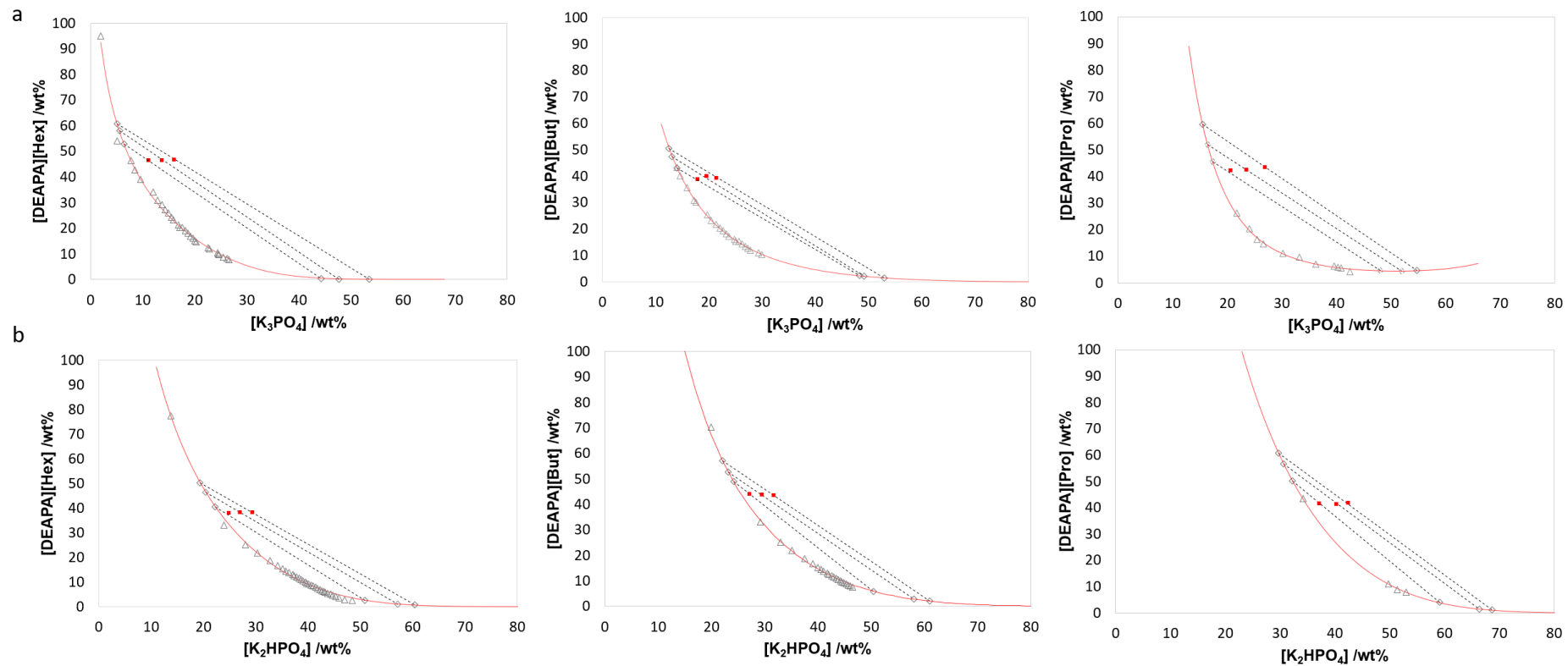
Figure C.1. Ternary phase diagrams for ABS composed of [DEAPA][X] + Salt ( a : K_3PO_4 and b : K_2HPO_4 ) + H_2O , at T = 298 K and atmospheric pressure. binodal curve data ( \Delta ); tie line experimental data ( \diamond ); total composition ( \blacksquare ); fitted binodal curve using Equation (5.1) (—).
