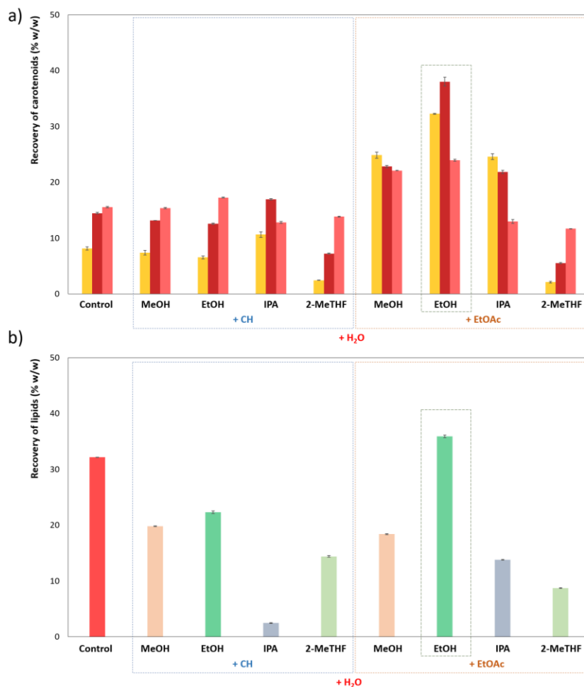
Figure 6.2. Recovery yields (% w/w) of (a) carotenoids (β-carotene [yellow], torularhodin [red], and torulene [pink]) and (b) lipids using aqueous (25% w/w of H 2 O) mixtures of CH (25% w/w) (+ MeOH, EtOH, IPA and 2-Me-THF) (50% w/w) and EtOAc (25% w/w) (+ MeOH, EtOH, IPA and 2-Me-THF) (50% w/w) at R. glutinis wet cell concentration of 0.2 g/mL after 1 h stirring (300 rpm) at 65 °C. The conventional Bligh and Dyer mixture of chloroform (25% w/w) + MeOH (50% w/w) +
