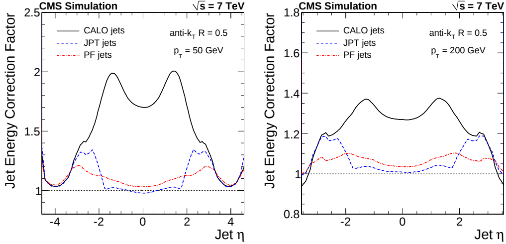
Figure 6. Monte Carlo jet-energy-correction factors for the different jet types, as a function of jet \eta . Left: correction factor required to get a corrected jet p_T = 50 \text{ GeV} . Right: correction factor required to get a corrected jet p_T = 200 \text{ GeV} .
