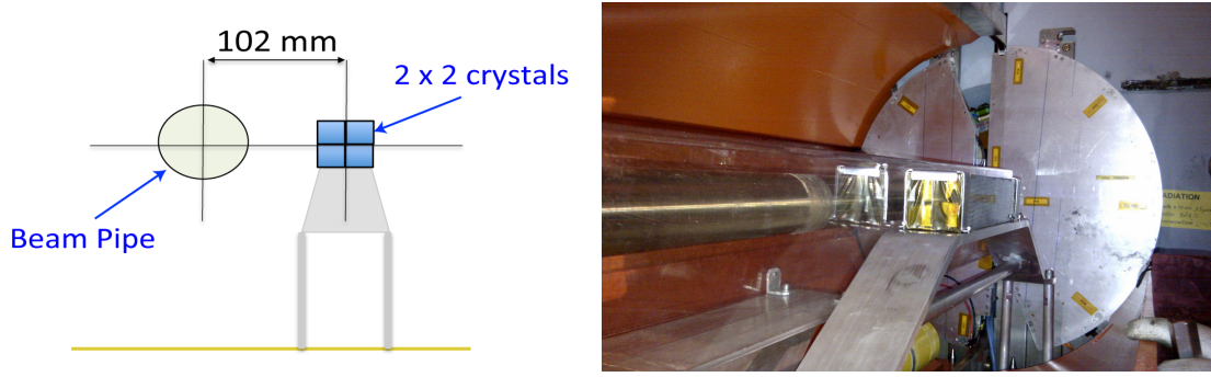
Figure 4. Schematic and photo of the 2 \times 2 EE-sized crystals irradiated close to the CMS beam pipe in 2012.
