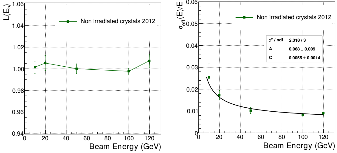
Figure 15. Average linearity (left), defined as \frac{E_{3 \times 3}}{E_{\text{beam}}} , and energy resolution (right) for the 3×3 clusters of non-irradiated crystals centered on the nine central crystals of 2012 matrix 1.
