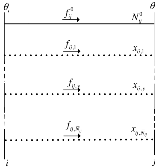
Figure 2 - Transmission lines model between two buses in the disjunctive model of TEP problem
