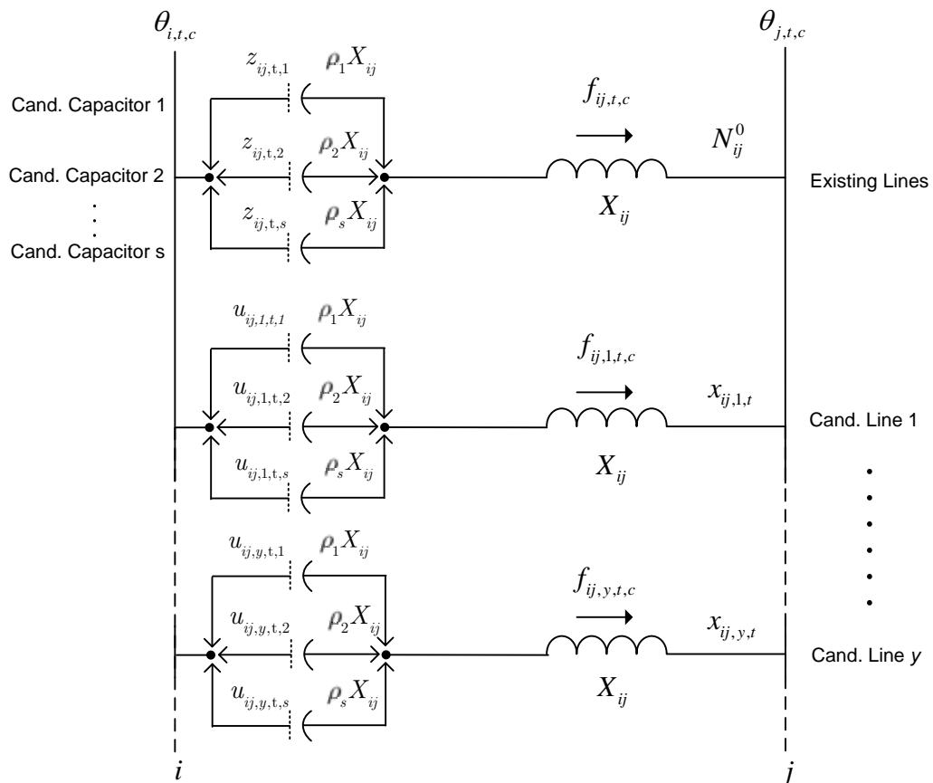
Figure 12 - General model for a transmission corridor with existing lines, candidate lines and FSCs
