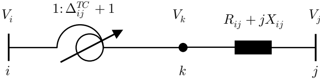
Fig. 1 Equivalent circuit of a VR/SS's OLTC.
