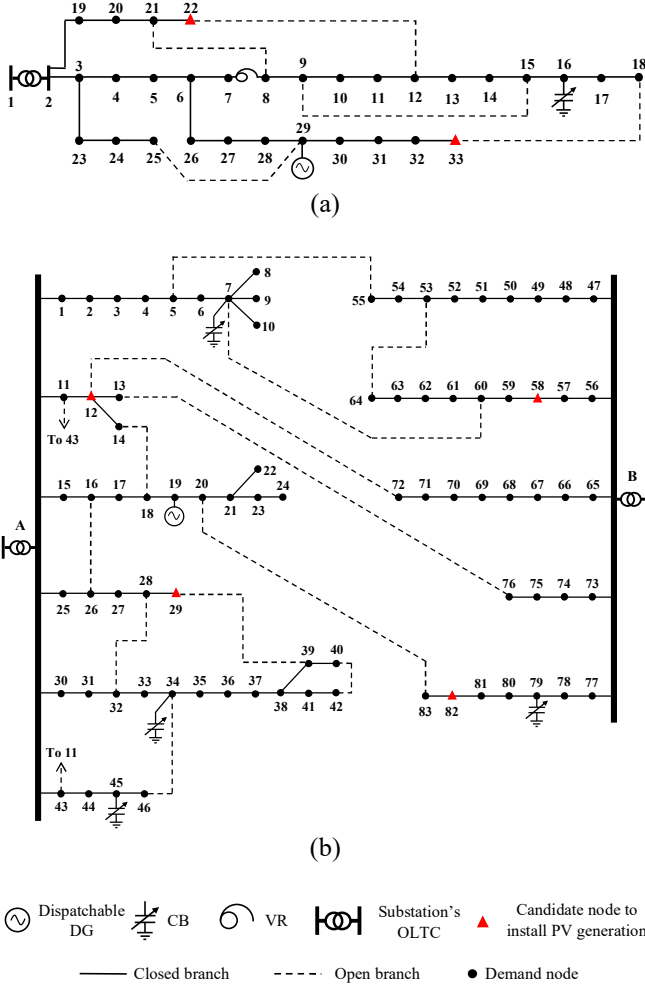
Fig. 5 Initial configuration of the (a) 33-node and (b) 85-node networks.
