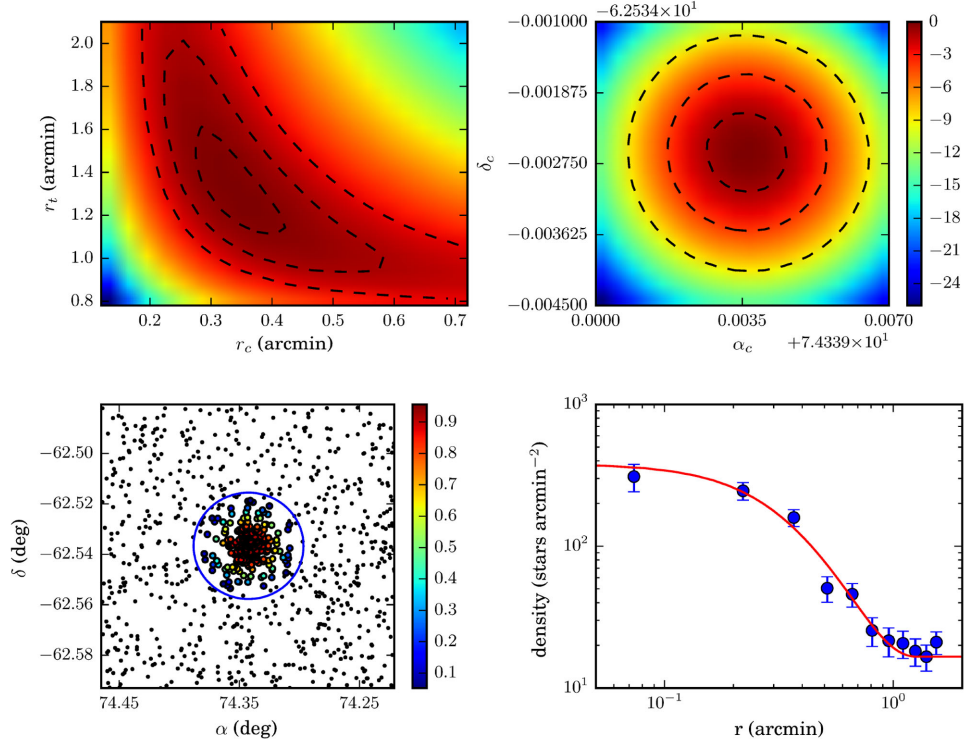
Figure 10. Maximum likelihood method applied to the cluster SL126. The most likely parameters for this cluster are r_c = 19 arcsec, r_t = 79 arcsec, \alpha_c = 74^\circ 34' 24'' , \delta = -62^\circ 53' 56'' , k = 0.14 stars arcsec ^{-2} . Top panels: likelihood distribution (normalized by maximum) over r_c and r_t (left) and over cluster centre coordinates (right). Lower left: field stars ( P^{kp} < 0.05 , black dots) and likelihood (colour bar) that each star belongs to the cluster. Lower right: density profile binned in 11 rings (blue dots) and the fitted density profile (solid red line).
