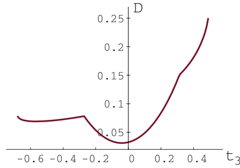
Figure 1. Quantum discord D = \mathcal{Q}(\rho_X) for x_3 = 0.1 , y_3 = 0.2 , t_1 = 0.2 , t_2 = 0.3 . Here the results in 24 , our numerical results and our upper bound in Eq. (10) agree with high precision.
