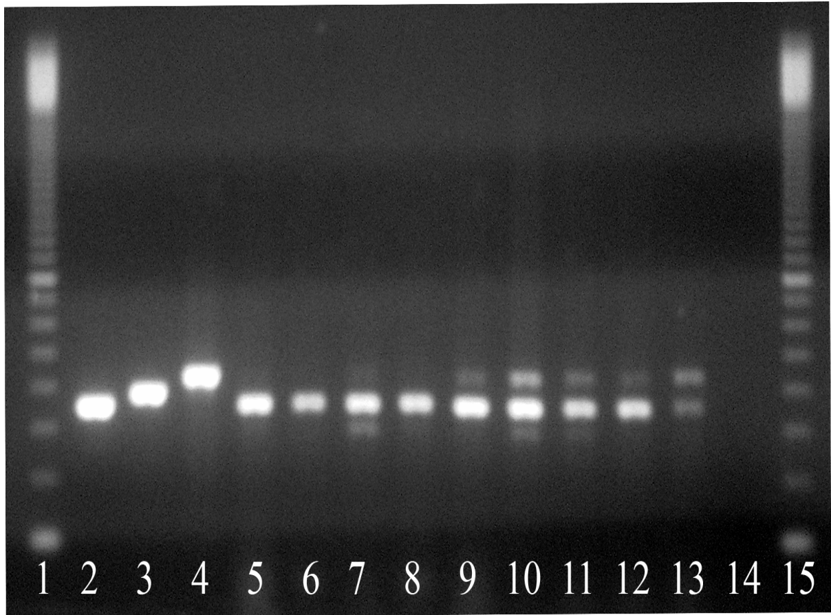
Figure 6 - Agarose gel electrophoresis (2%) showing PCR amplification bands with the genus oligonucleotide primer pair using DNA extracted from fecal samples of Lewis rats infected with 400 L3. Lanes 1 and 15 – 100 bp ladder (GE Healthcare). Lane 2 – 340 bp ( S. venezuelensis DNA). Lane 3 – 380 bp ( Syphacia muris DNA). Lane 4 – 420 bp ( Rattus norvegicus DNA). Lanes 5 to 13 – DNA from fecal samples - 340 bp S. venezuelensis DNA. Lanes 9 to 13 – 420 bp R. norvegicus DNA. Lanes 7, 10 and 11 – 300 bp -unspecific band. Lane 14 - without DNA.
