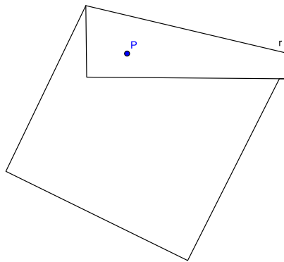
Figura 2.17: Reta perpendicular, P \notin r - passo 2
