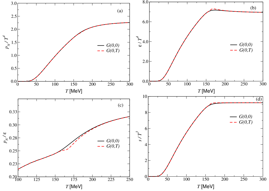
Figure 4. Panel (a): Scaled pressure p_N/T^4 . Panel (b): Scaled energy density \epsilon/T^4 . Panel (c): Equation of state p_N/\epsilon . Panel (d): Scaled entropy density s/T^3 ( s = dP/dT ).
