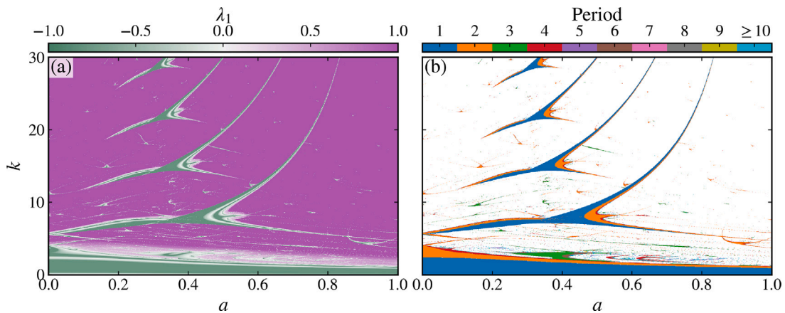
Fig. 3. Demonstration of the use of the (a) lyapunov method and (b) period method from the DiscreteDynamicalSystem class of dynamicalsys for the dissipative kicked rotor map [Eq. (24)] with parameter \gamma = 0.8 . Execution times: (a) 25 min 31 s and (b) 7 min 56 s. (For interpretation of the references to color in this figure legend, the reader is referred to the web version of this article.)
