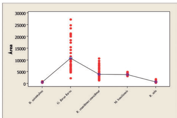
Fig. 6. Distribution of cell area ( \mu\text{m}^2 ) in prophase I of the five species of Heteroptera analyzed.
