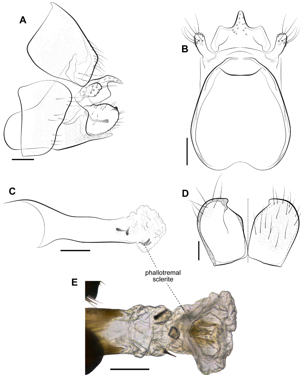
Figure 5. Chimarra (Curgia) prata sp. nov., male genitalia (holotype): (A) Segments VIII, IX, tergum X, and inferior appendage, left lateral view; (B) Segment IX and tergum X, dorsal view; (C) Phallic apparatus, left lateral view; (D) Left inferior appendage, dorsal view (left) and ventral view (right); (E) Phallic apparatus, dorsal view (photograph). Scale bars in mm: 0.1.
