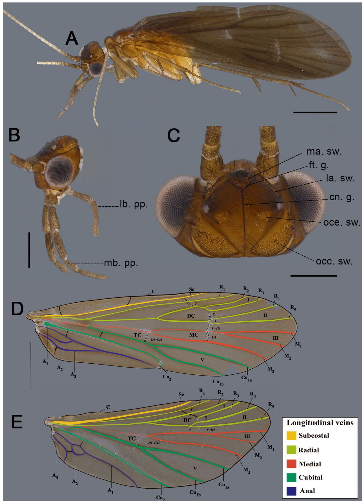
Figure 2. Chimarra (Curgia) opala sp. nov., holotype male: (A) Left lateral habitus; (B) Head, left lateral view; (C) Head, dorsal view; (D) Venation of the right forewing, dorsal view (longitudinal veins highlighted in colors); (E) Venation of the right hindwing, dorsal view (longitudinal veins highlighted in colors). Scale bars in mm: (A,D,E) = 1; (B) = 0.2; (C) = 0.5.
