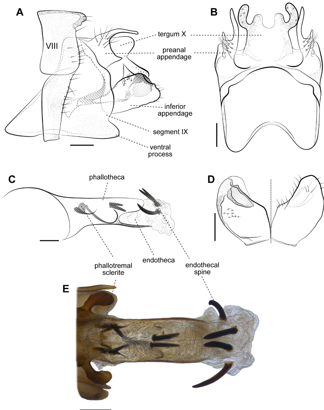
Figure 3. Chimarra (Curgia) opala sp. nov., male genitalia (holotype): (A) Segments VIII, IX, tergum X, and inferior appendage, left lateral view; (B) Segment IX and tergum X, dorsal view; (C) Phallic apparatus, left lateral view; (D) Left inferior appendage, dorsal view (left) and ventral view (right); (E) Phallic apparatus, dorsal view (photograph). Scale bars in mm: 0.1.
