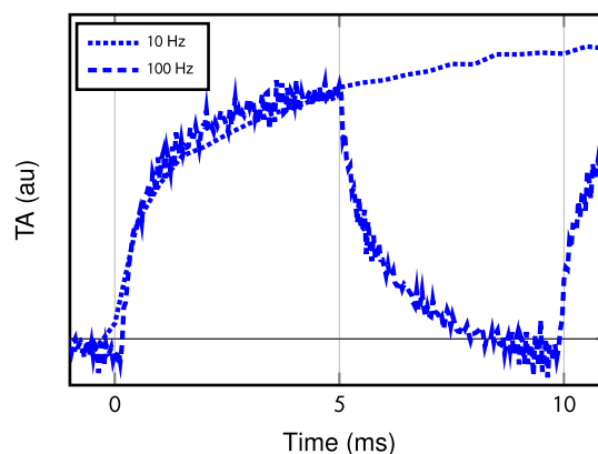
Figure 8. Comparison of transient absorption measurements for external load resistor of 90 kΩ with pump intensity of 25 mW at frequency modulation of 10 and 100 Hz.
