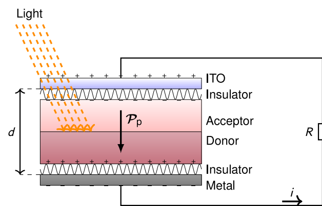
Figure 1. Photoinduced polarization \mathcal{P}_p on an LHC. The waved lines between the active layer (acceptor/donor) and the contacts represent the insulating layers.
