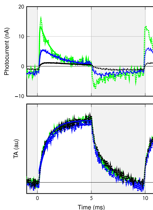
Figure 7. Photocurrent (top) and transient absorption (bottom) for external load resistors of 30 kΩ (green), 90 kΩ (blue), and 342 kΩ (black). Dotted lines represent the measured data, and solid lines result from theoretical fitting with eq 14 to the photocurrent or from monoexponential fitting to the transient absorption.
