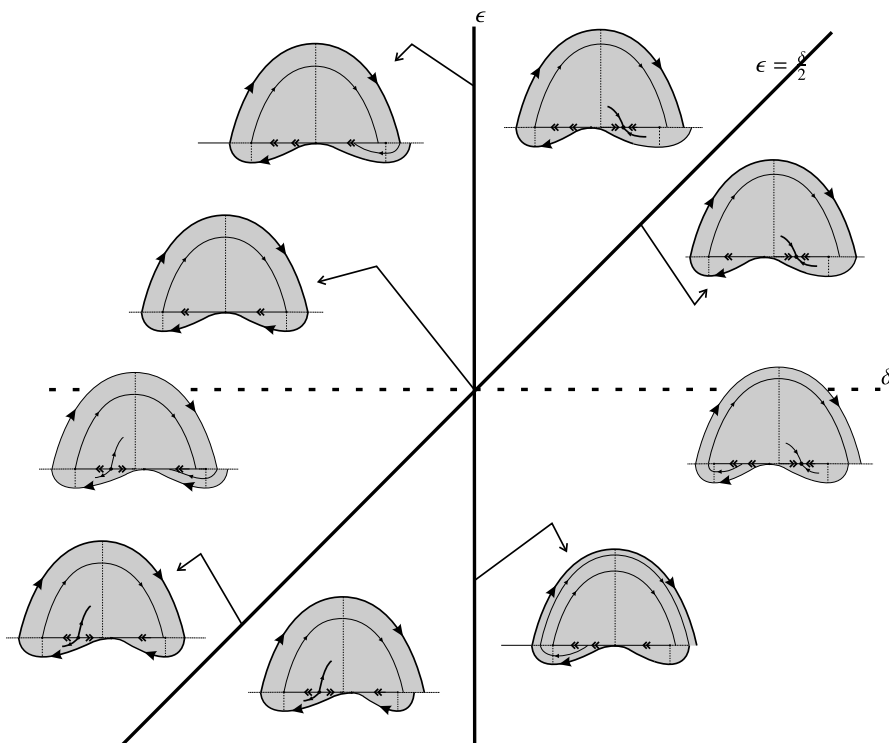
Fig. 11. Bifurcation diagram.
