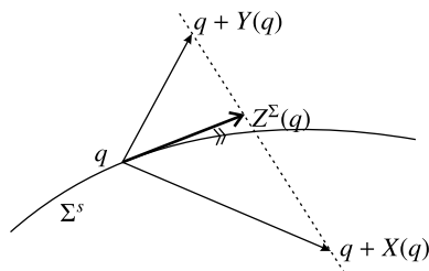
Fig. 1. Filippov's convention.
