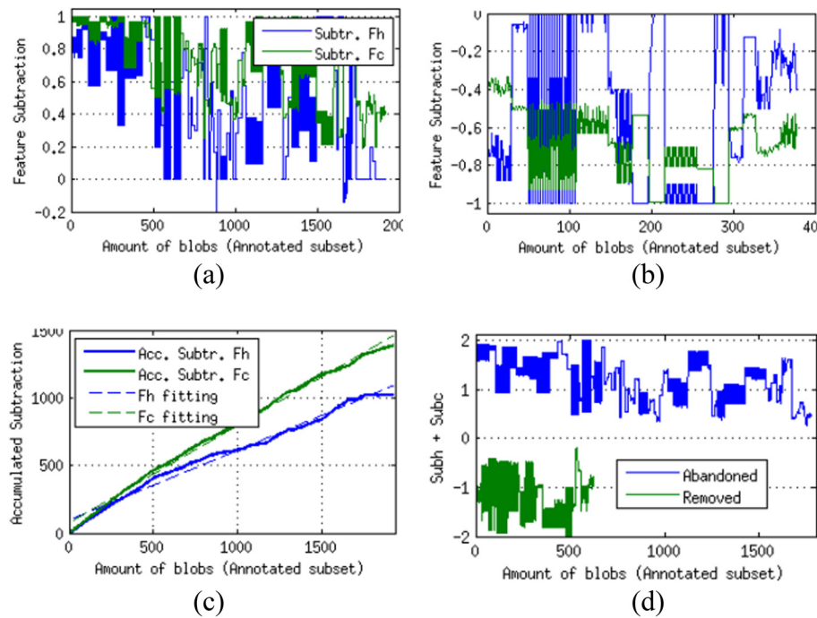
Figure 7 Plots of the annotated subset. (a) Feature subtraction of abandoned blobs. (b) Feature subtraction of removed blob. (c) Accumulated subtraction of abandoned blobs. (d) Plot of Sub_h + Sub_c .
