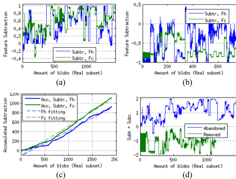
Figure 8 Plots of the real subset. (a) Feature subtraction of abandoned blobs. (b) Feature subtraction of removed blob. (c) Accumulated subtraction of abandoned blobs. (d) Plot of Sub_h + Sub_c .
