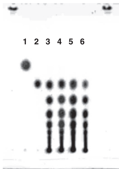
Fig. 7. Thin-layer chromatography of the hydrolysis products of oat spelts xylan by Xyl I from T. inhamatum . Row: 1 xylose. Row 2: xylobiose. Rows 3, 4, 5 and 6: 10 min, 30 min, 2 h and 17 h of hydrolysis, respectively.
