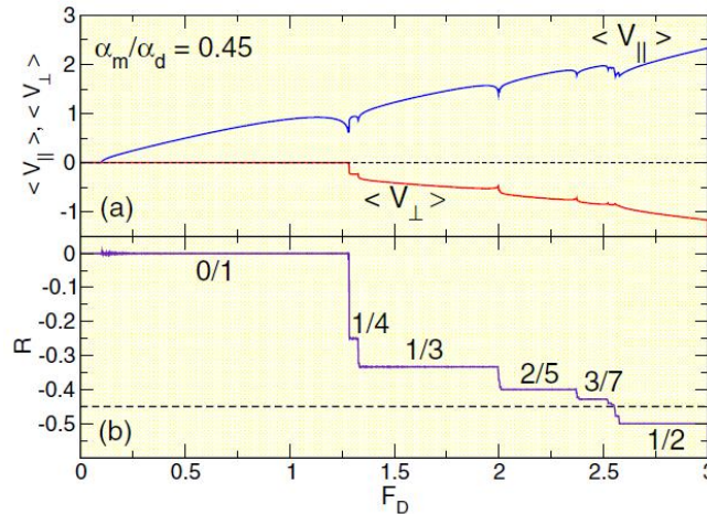
Figure 3.5 – (a) The average velocity curves, \langle V_{\parallel} \rangle and \langle V_{\perp} \rangle , as a function of the applied driving force F_D for a system using \alpha_m/\alpha_d = 0.45 . \langle V_{\parallel} \rangle is the velocity parallel to the applied drive and \langle V_{\perp} \rangle is perpendicular. (b) The R curve as a function of the applied drive F_D . The velocity dips are related to a change in the skyrmion direction of motion. The dashed line in (a) represents null velocities and in (b) it represents the intrinsic skyrmion Hall angle. (From Reichhardt et. al. (2015), pg 104426-4 [39]).
