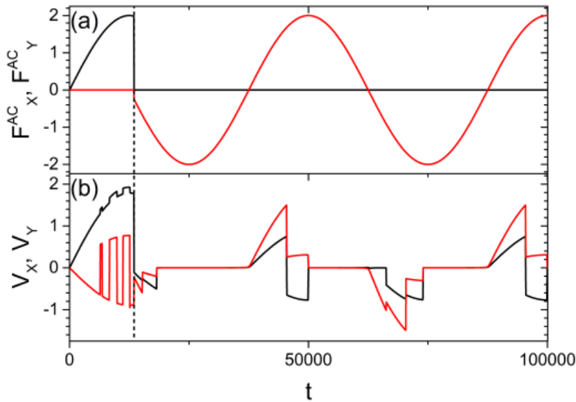
Figure 12.6 – The applied ac drive forces F_x^{AC} (black) and F_y^{AC} (red), versus time t for the guided motion shown in Fig. 12.5. Note that the time axis is truncated at t = 100,000 , but the same ac driving is applied at later times to achieve the results shown in Fig. 12.5. (b) The instantaneous skyrmion velocities V_x (black) and V_y (red) versus t under the driving shown in (a). The dashed vertical line indicates the transition at which the ac drive direction is switched. (From Bellizotti Souza et. al. [204], pg. 8).
