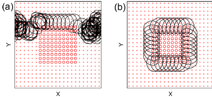
Figure 9.8 - The obstacles (open circles) and the skyrmion trajectory (black lines) for the system using \alpha_m/\alpha_d = 0.45 , circular ac driving where A = B and \omega = 2 \times 10^{-5} . (a) A = 0.886 a partially motion along the interface, where the skyrmion cannot turn corners. (b) A = 0.894 a translating orbit where the skyrmion follows the interface turning all four corners. (From Vizir et. al. [198], pg. 6).
