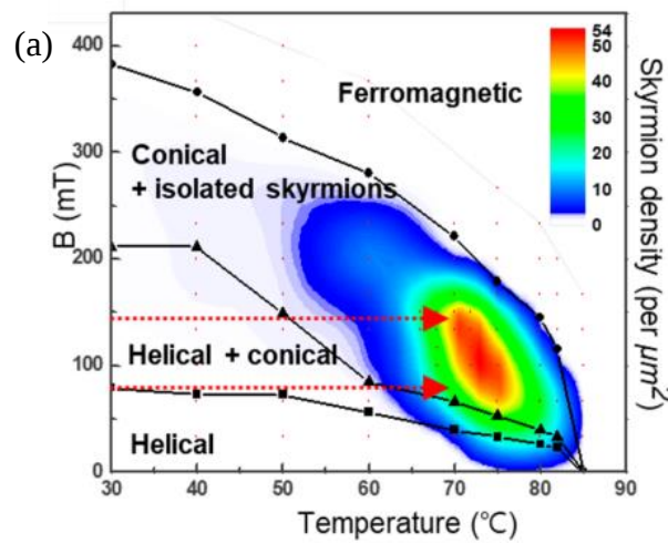
Figure 13.1 – (a) Phase diagram of the skyrmion density in the magnetic field ( B ) vs. temperature ( T ) plane deduced from LTEM observations for a \text{Co}_8\text{Zn}_{10}\text{Mn}_2 thin plate. (From Kim et. al. [212], pg. 5548). [(b), (c), (d)] Simulation results for spin configurations at a transversal section of a thin plate in the xz plane for varied applied magnetic field values in the z direction. (b) The spin configuration in the absence of field, the Helical phase. (c) For intermediate fields, the Conical phase. (d) For high fields, the saturated ferromagnetic phase, where all spins align with the applied field (Figs. (b), (c) and (d) are elaborated by the author).
