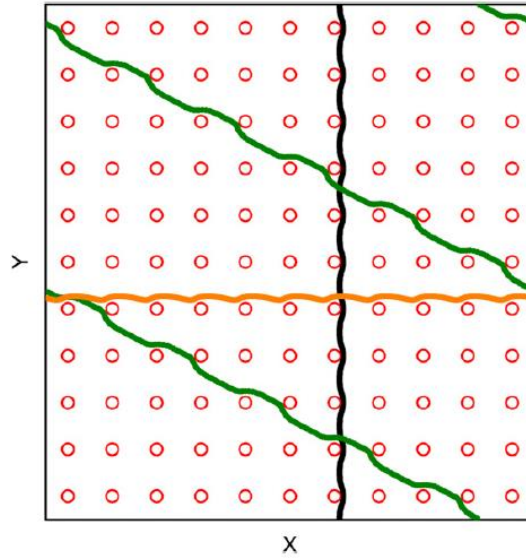
Figure 5.11 - The obstacles (open circles) and the skyrmion trajectory (lines) for a system with a_0 = 0.65 at \alpha_d = 0 (black), 2.0 (green) and 5.0 (orange). (From Vizir et. al. [137], pg. 9).
