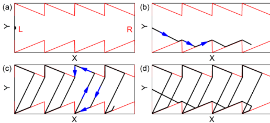
Figure 12.5 – Funnel walls (red lines) and the skyrmion trajectory (black lines) for the system where the skyrmion starts in funnel L and must travel to R and return back to L . The blue arrows indicate the direction of the skyrmion motion. (a) skyrmion starting position in funnel L for t = 0 . (b) First stage of operation with A = 2.0 and B = 0 , where the skyrmion moves from L to R . (c) Second stage of operation with A = 0 and B = 2.0 , where the skyrmion moves from R to L . (d) The complete trajectory, adding operations 1 and 2 together. (From Bellizotti Souza et al. [204], pg. 8).
