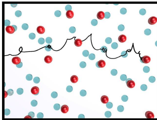
Figure 3.1 –Illustration of skyrmion (red circles) and the pinning centers randomly placed (blue circles). The black line is a selected skyrmion trajectory as it moves through the sample and interact with pinning centers. (From Reichhardt et. al. (2015), pg 217202-2 [26]).
