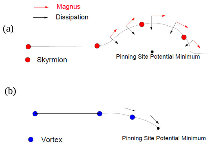
Figure 1.5 – Schematic illustrations of a (a) skyrmion and a (b) superconducting vortex interacting with an attractive point-like pinning site. The velocity component induced by the dissipation is indicated by black arrows, and that produced by the Magnus force is red. The Magnus force is always perpendicular to the attractive force of the pinning center, resulting in a deflection. (adapted from C. Reichhardt et al. [74], 2022, page 14).
