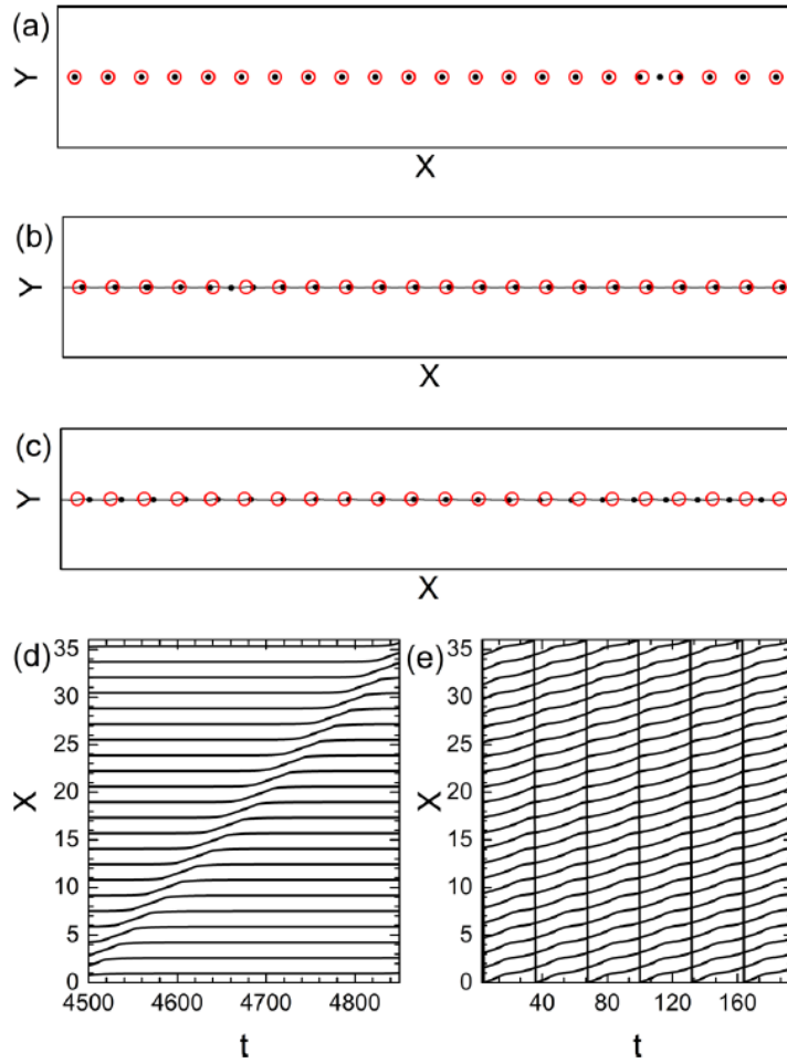
Figure 11.3 – In [(a), (b), (c)] the representation of the pinning site positions (red circles) and the skyrmion trajectories (black lines) for a sample with N_{sk}/N_p = 1.044 , \alpha_m/\alpha_d = 0.5 , C_p = 0.15 and n_p = 0.093/\xi^2 . (a) At F^D = 0.01 , the skyrmions are static in the pinned phase. The interstitial skyrmion is present due to the incommensuration between the skyrmion and the pinning site number. (b) For F^D = 0.3 , the interstitial skyrmion moves as a soliton by hopping from site to site with slow average velocity. (c) At F^D = 1.0 all skyrmions flow simultaneously at higher velocities. [(d) and (e)] Skyrmion positions as a function of time. (d) For F^D = 0.3 , as shown in panel (b), the soliton pulse propagates through the sample. (e) For F^D = 1.0 , all skyrmions flow through the sample, as shown in panel (c). (From Vizir et. al. [207], pg. 224409-4).
