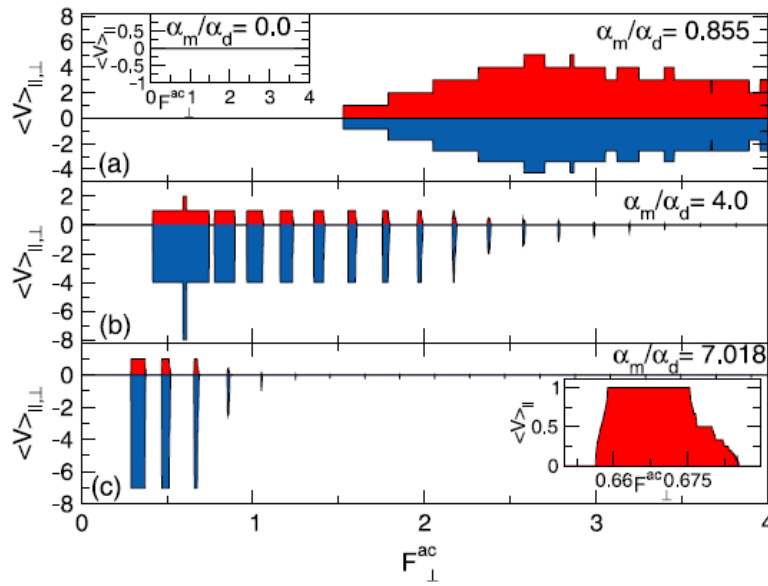
Figure 3.16 – The skyrmion average velocity parallel, \langle V_{\parallel} \rangle and perpendicular \langle V_{\perp} \rangle to the substrate asymmetry versus F_{\perp}^{ac} . (a) for \alpha_m/\alpha_d = 0.855 , in the inset is shown the overdamped case where the ratchet is absent, (b) \alpha_m/\alpha_d = 4.0 and (c) \alpha_m/\alpha_d = 7.018 , the inset shows a blowup of \langle V_{\parallel} \rangle . (From Reichhardt et. al. (2015), pg 5 [32]).
