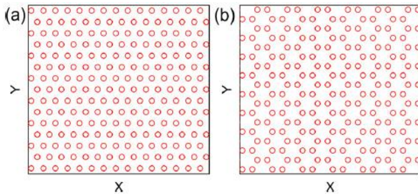
Figure 10.1 – An illustration of the obstacle lattices used in this work. (a) Triangular obstacle array and (b) the honeycomb lattice. (From Vizir et. al. [200], pg. 2)
