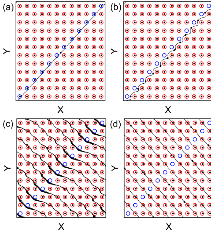
Figure 11.14 – Pinning site positions (red circles) and the skyrmion trajectories (black lines) for the sample of Fig. 11.13 with N_{sk}/N_p = 1.01 , \alpha_m/\alpha_d = 1.0 , weak pins C_p = 0.15 , strong pins C_p = 1.0 and n_p = 0.373/\xi^2 . (a) At F^D = 0.25 where the soliton flows following the weak line of pins, at \theta_{sk} = +45^\circ . (b) At F^D = 0.5 , the skyrmions trapped in the weak line of pins depin and flow along \theta_{sk} = +45^\circ . (c) For F^D = 1.0 the transient phase, where \theta_{sk} gradually reverses. In this case, \theta_{sk} \approx -35^\circ . (d) For F^D = 1.8 , the skyrmion Hall angle reversal is complete, the flow is locked at \theta_{sk} = -45^\circ . (From Vizir et. al. [204], pg. 224409-9).
