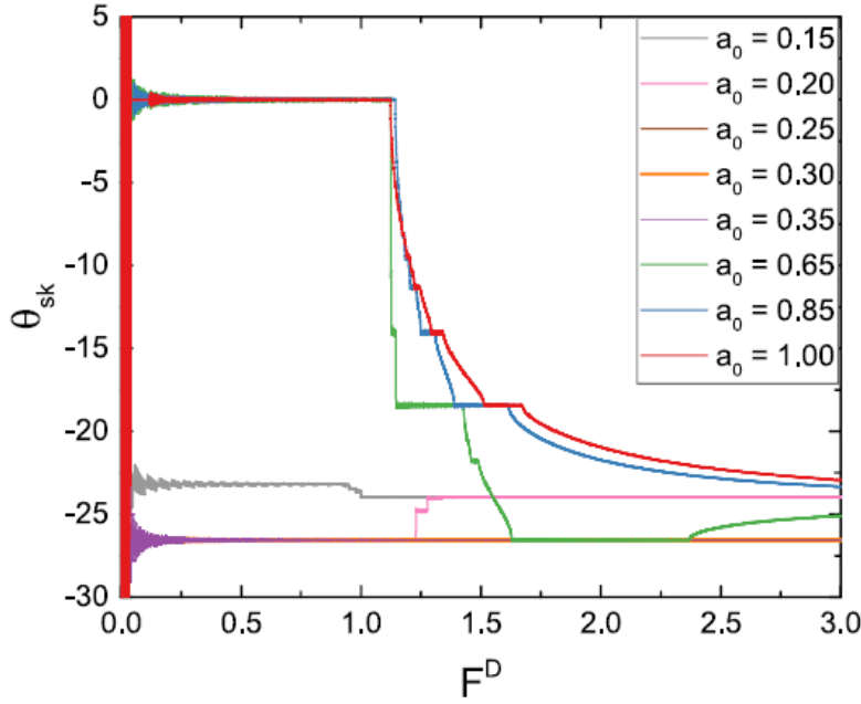
Figure 5.3 – The skyrmion Hall angle, \theta_{sk} = \arctan R vs. F^D , where R = \langle V_{\perp} \rangle / \langle V_{\parallel} \rangle , in samples with \alpha_m/\alpha_d = 0.45 at varied a_0 (From Vizir et. al. [137], pg. 5).
