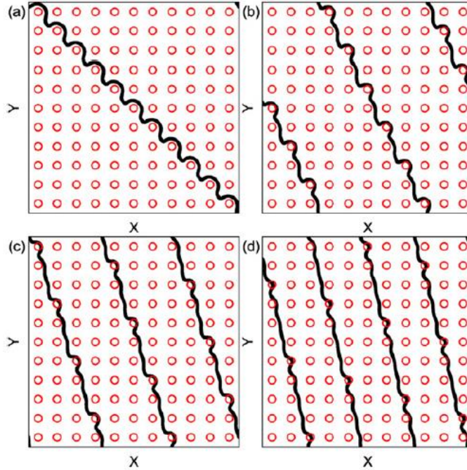
Figure 5.8 – The obstacles (open circles) and the skyrmion trajectory (black lines) for the system in Fig. 5.7 (a) with \alpha_m/\alpha_d = 4.925 and a_o = 1.0 . (a) The R = -1.0 state, (b) the R = -2.0 , (c) the R = -3.0 state and (d) R = -4.0 state. (From Vizir et al. [137], pg. 8).
