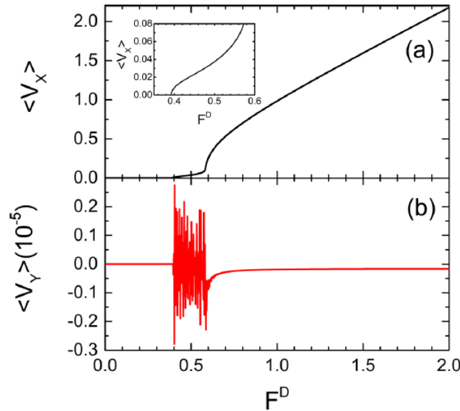
Figure 11.4 – The skyrmion average velocities (a) \langle V_x \rangle and (b) \langle V_y \rangle as a function of the applied drive, F^D , for the sample illustrated in Fig. 11.1 (a) with N_{sk}/N_p = 0.96 , \alpha_m/\alpha_d = 0.5 and n_p = 0.093/\xi^2 . The inset shows a blowup of panel (a) over the range 0.35 < F^D < 0.6 . (From Vizir et. al. [207], pg. 224409-4).
