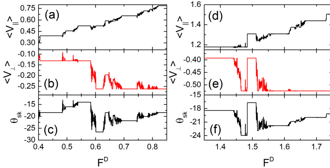
Figure 6.9 - The average velocities (a) \langle V_{\parallel} \rangle (black) and (b) \langle V_{\perp} \rangle (red) and (c) \theta_{sk} as a function of the applied dc force F^D under a finite ac driving force with amplitude B = 0.5 for the interval 0.4 < F^D < 0.85 . The average velocities (a) \langle V_{\parallel} \rangle (black) and (b) \langle V_{\perp} \rangle (red) and (c) \theta_{sk} as a function of the applied dc force F^D under a finite ac driving force with amplitude B = 0.5 for the interval 1.35 < F^D < 1.75 using \alpha_m/\alpha_d = 0.45 and a_o = 0.65 (From Vizir et. al. [161], pg. 104413-6).
