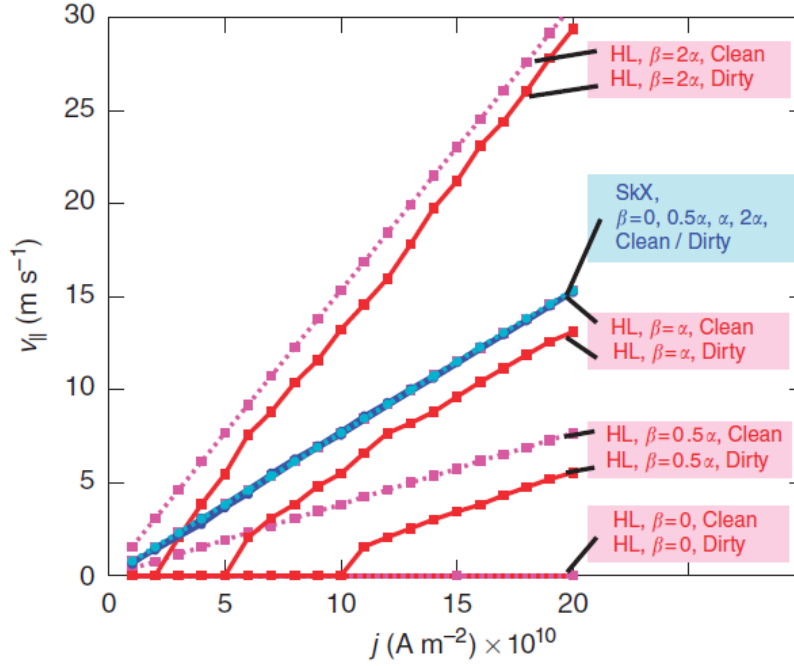
Figure 2.13 – Current-velocity curves, v_{\parallel} vs. j , for the helical (HL) and skyrmion crystal (SkX) phases. The clean case is when x = 0 , where x is the impurity concentration. The dirty case when x = 0.1\% . Lines for the SkX phase are all the same, while for HL phase it greatly depends on the parameters (From Iwasaki et. al. (2013), pg 3).
