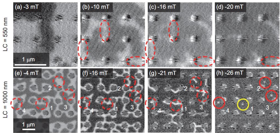
Figure 3.14 – XMCD-STXM images of the magnetic evolution as the applied magnetic field is varied in the antidot array. From (a) – (d) using LC = 550 nm and from (e) – (h) using LC = 1000 nm. Dark and bright contrasts represents the magnetization domains point up or down, respectively. Skyrmion are highlighted with solid circles and magnetic domains with red dashed circles and ellipses. (From Saha et. al. (2019), pg 144435-6 [64]).
