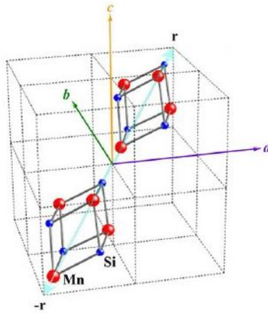
Figure 2.2 –Crystal structure of MnSi with B20 cubic symmetry, which is noncentrosymmetric, as revealed by the fact that inversion operation ( \mathbf{r} \rightarrow -\mathbf{r} ) does not produce identical unit (adapted from T. Y. Ou-Yang et. al. , J. Phys. Condens. Matter 28, 026004 (2015) [87]).
