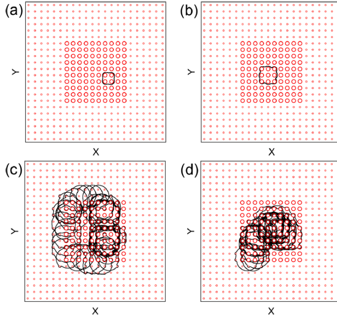
Figure 9.10 - The obstacles (open circles) and the skyrmion trajectory (black lines) for the system using \alpha_m/\alpha_d = 9.962 , circular ac driving where A = B and \omega = 1 \times 10^{-5} . (a) A = 0.03 a localized orbit encircling four obstacles. (b) A = 0.1 a localized orbit encircling nine obstacles. (c) A = 0.324 , the skyrmion jumps between clockwise motion through the interface and disordered motion in the bulk. (d) A = 0.34 a disordered motion. (From Vizir et. al. [198], pg. 8).
