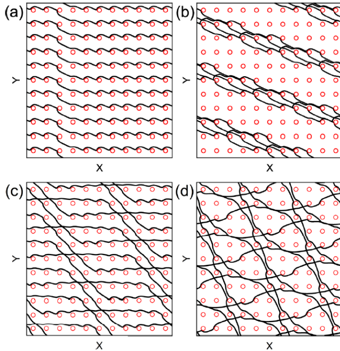
Figure 6.17 – The obstacles (open circles) and the skyrmion trajectory (black lines) for the system in Fig. 6.16 with \alpha_m/\alpha_d = 1.0 and fixed dc drive F^D = 1.0 . (a) At A = 0.2 where the skyrmion moves 10 lattice constants in x and one lattice constant in y . (b) A R = 1/3 step at A = 1.0 . (c) Skyrmion motion at B = 0.34 and (d) for B = 1.0 . (From Vizir et. al. [161], pg. 104413-9).
