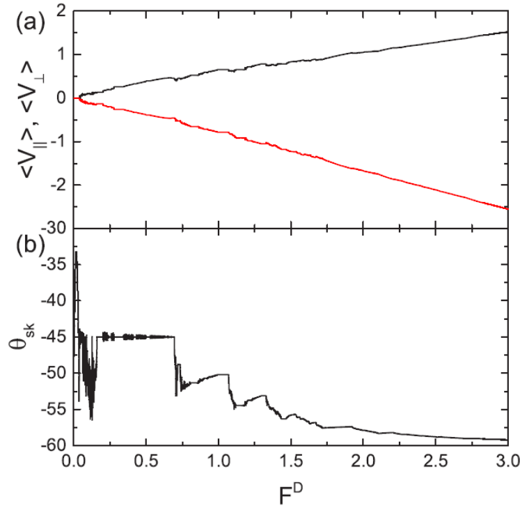
Figure 6.5 - (a) The average velocities \langle V_{\parallel} \rangle (black) and \langle V_{\perp} \rangle (red) as a function of the applied dc force F^D under a finite ac driving force with amplitude A = 0.5 . (b) The corresponding \theta_{sk} curve as function of the applied dc drive F^D for a single skyrmion in the square obstacle array using \alpha_m/\alpha_d = 1.732 and a_o = 0.65 (From Vizir et. al. [161], pg. 104413-5).
