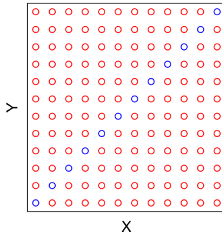
Figure 11.12 – Pinning site positions (red circles: strong pins; blue circles: weak pins) for a sample with a diagonal line of weak pinning sites oriented at +45^\circ respective to the x direction. The weak pins have C_p = 0.15 , strong pins C_p = 1.0 and we set n_p = 0.373/\xi^2 . (From Vizari et. al. [207], pg. 224409-8).
