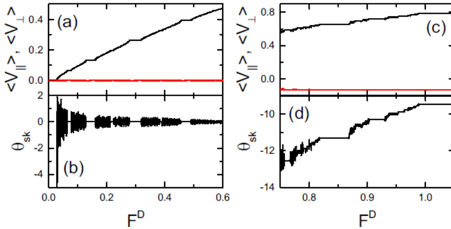
Figure 6.2 – (a) The zoom in the range of 0 < F^D < 0.6 from Fig. 6.1, showing the average velocities \langle V_{\parallel} \rangle (black) and \langle V_{\perp} \rangle (red) as a function of the applied dc force F^D . (b) The corresponding \theta_{sk} curve as function of the applied dc drive F^D . (c) The zoom in the range of 0.7 < F^D < 1.2 from Fig. 6.1. (d) The corresponding \theta_{sk} curve showing the decrease in magnitude of \theta_{sk} with increasing F^D for a single skyrmion in the square obstacle array using \alpha_m/\alpha_d = 0.45 , \alpha_o = 0.65 and the ac drive with A = 0.5 (From Vizir et. al. [161], pg. 104413-3).
