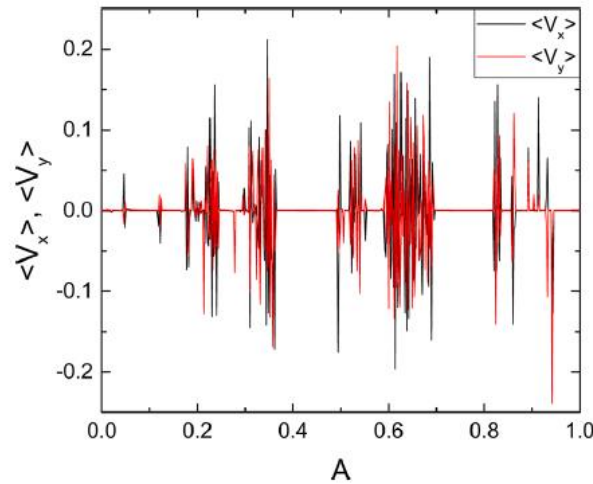
Figure 9.11 – The average velocities \langle V_x \rangle and \langle V_y \rangle as a function of the ac drive amplitude A for the system in Fig. 9.10 using \alpha_m/\alpha_d = 9.962 . (From Vizir et. al. [198], pg. 8).
