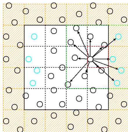
Figure 4.5 – Periodic boundary conditions being applied to a cell on the edge of the main simulation box. Particles inside the cell in red interact with particles from the opposite side of the main simulation box.
