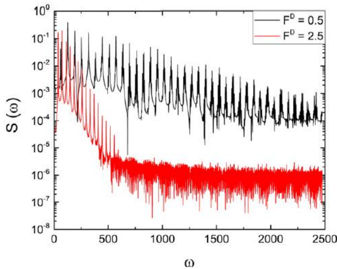
Figure 10.5 – The Fourier transform S(\omega) of the V_{\parallel} data exhibited in Fig. 10.4. for the triangular array with \rho_t = 0.128 and \alpha_m/\alpha_d = 1.0 in the locking regime (black) and the non-locking regime (red). The peaks are much stronger in the locking regime. (From Vizirim et. al. [200], pg. 4).
