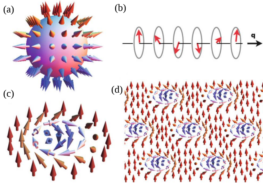
Figure 1.1 – In (a) the Skyrmion illustration as proposed by Tony Skyrme in the 60s. In (b) an illustration of the helical state present in chiral magnets as a consequence of the competition between the Dzyaloshinskii-Moriya and the ferromagnetic exchange interactions. In (c) the skyrmion representation recently discovered in chiral magnets. In (d) an illustration of a skyrmion array in chiral magnets under the influence of a applied magnetic field. Note that they arrange themselves in a regular triangular lattice (adapted from S. Seki and M. Mochizuki, 2016, page 2).
