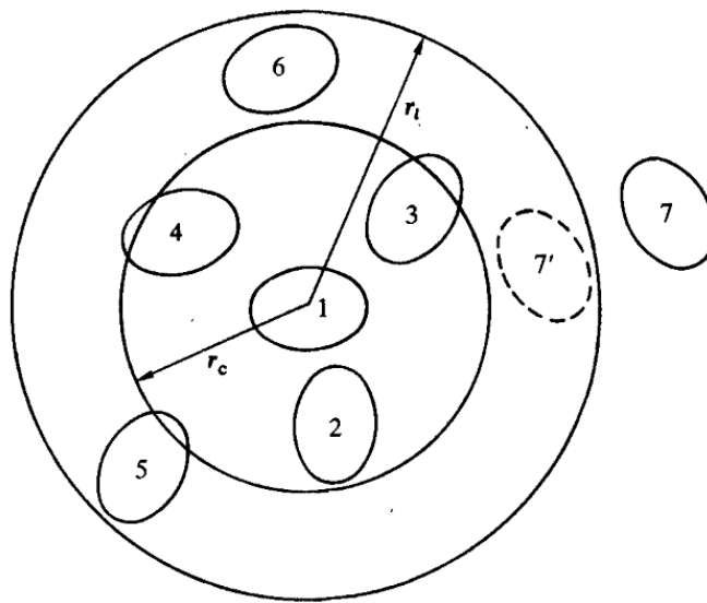
Figure 4.3 – The cutoff and skin spheres around the particle 1. The particles 2, 3, 4, 5 and 6 are on the list of particle 1, but particle 7 is not on the list. Only particles 2, 3 and 4 are within the range of the potential cutoff at the time the list is constructed (From M. P. Allen, D. J. Tildesley, and L. Allen [153]).
