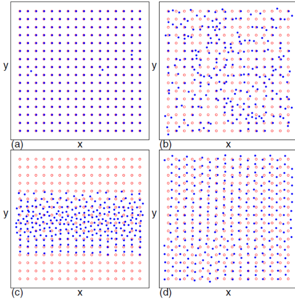
Figure 3.11 – Skyrmion positions (blue dots) and pinning center positions (red circles) for the system of Fig. 3.10. (a) The pinned Phase I, (b) the disordered flow os skyrmions Phase III, (c) the segregated skyrmion phase PS, and (d) the moving crystal MC phase. (From Reichhardt et. al. (2018), pg 134418-4 [40]).
