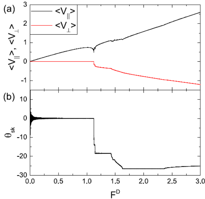
Figure 5.1 - (a) the average velocity curves \langle V_{\parallel} \rangle, \langle V_{\perp} \rangle as a function of the transport force F^D containing a single skyrmion where a_0 = 0.65 and \alpha_m/\alpha_d = 0.45 . For F^D < 1.0 the motion is strictly in the x direction, parallel to the driving force. (b) the corresponding skyrmion Hall angle \theta_{sk} = \arctan(R) vs F^D curve (From Vizari et al. [137], pg. 4).
