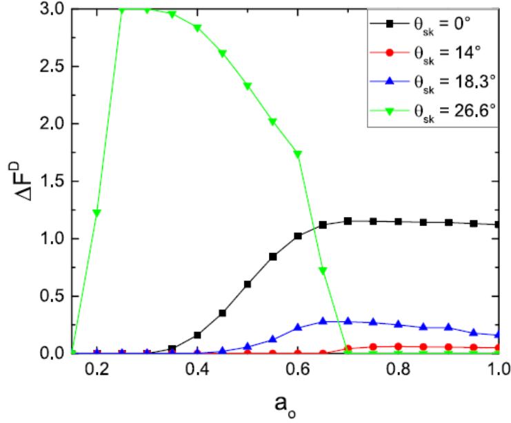
Figure 5.4 - Range of forces \Delta F^D as a function of the obstacle radius a_o for a single skyrmion in the square obstacle array using \alpha_m/\alpha_d = 0.45 (From Vizir et. al. [137], pg. 6).
