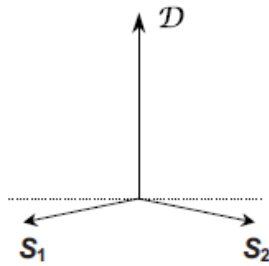
Figure 2.3 – Vector representation of the Dzyaloshinskii-Moriya interaction. Here, \mathbf{D} is always perpendicular to the plane formed by \mathbf{S}_1 and \mathbf{S}_2 (Adapted from Coey, 2009, page 139).
