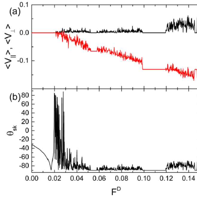
Figure 7.7 – Blowup of Fig. 7.6 for the interval 0 < F^D < 0.15 . (a) The average velocities \langle V_{\parallel} \rangle (black) and \langle V_{\perp} \rangle (red) as a function of the applied dc force F^D . (b) The corresponding \theta_{sk} curve. (From Vizir et. al. [180], pg. 6).
