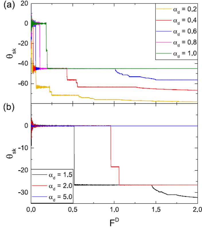
Figure 5.10 - In (a) and (b) the \theta_{sk} vs F^D curve for the system of Fig. 5.9 with fixed \alpha_m = 1.0 and a_0 = 0.65 (From Vizir et. al. [137], pg. 9).
