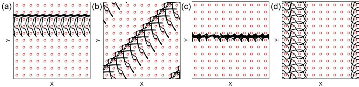
Figure 8.22 - The obstacles (open circles) and the skyrmion trajectory (black lines) for the system with \alpha_m/\alpha_d = 0.577 and circular ac driving where A = B and a_0 = 0.65 . (a) and (b) Sample with \omega_2/\omega_1 = 0.5 . (a) A = 0.4 a translating orbit along +x direction. (b) A = 0.58 a translating orbit along 45^\circ . (c) and (d) Sample with \omega_2/\omega_1 = 2.0 . (c) A = 0.2 a disordered translating orbit along -x direction. (d) A = 1.0 a translating orbit along +y direction. (From Vizir et. al. [189], pg. 16).
