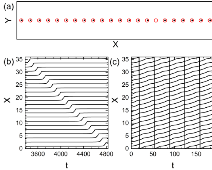
Figure 11.5 – In (a) the representation of the pinning site positions (red circles) and the skyrmion trajectories (black lines) for a sample with N_{sk}/N_p = 0.96 , \alpha_m/\alpha_d = 0.5 , C_p = 0.15 and n_p = 0.093/\xi^2 . (a) At F^D = 0.3 , the skyrmions are static in the pinned phase. The vacant pinning site is present due to the incommensuration between the skyrmion and the pinning site number. [(b) and (c)] Skyrmion positions as a function of time. (b) For F^D = 0.45 the soliton pulse propagates through the sample along -x direction. (c) For F^D = 1.0 , all skyrmions are flowing as a moving crystal. (From Vizir et. al. [207], pg. 224409-5).
