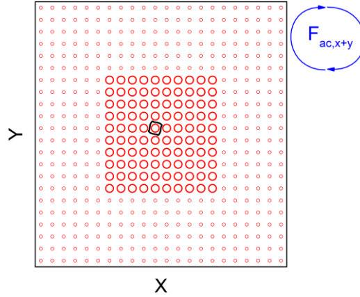
Figure 9.1 - A schematic of the system, which consists of regions of a square array of obstacles (red circles) with different sizes. The larger obstacles have R_0^L = 0.85 and the small ones R_0^S = 0.45 . The black lines correspond to the skyrmion trajectories under the influence of both damping, Magnus term, and circular ac drive (From Vizir et. al. [198], pg. 2)
