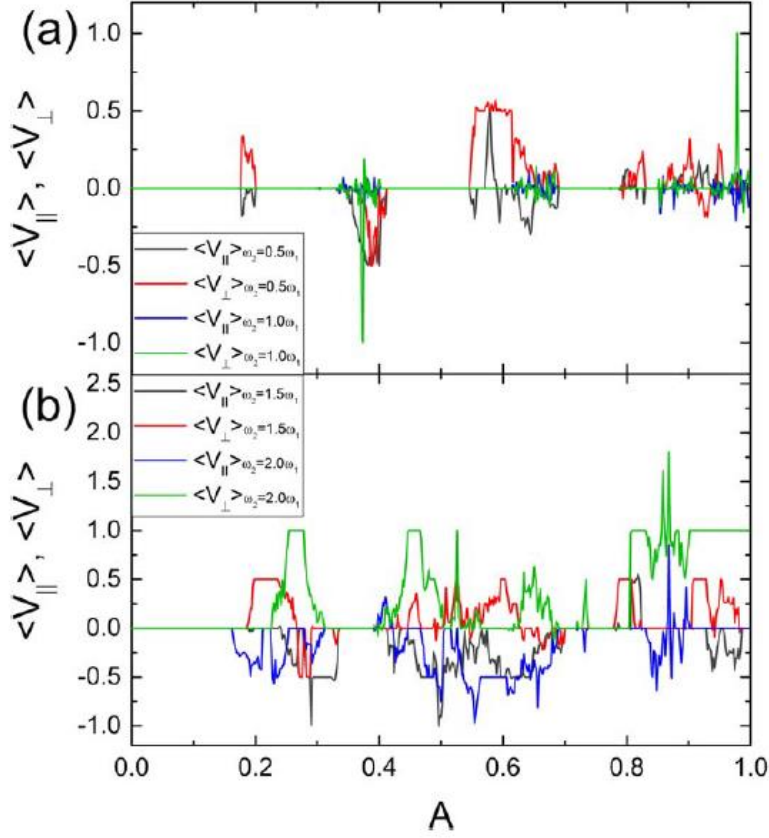
Figure 8.21 The velocities \langle V_{\parallel} \rangle and \langle V_{\perp} \rangle as a function of the ac drive amplitude, A = B , for a single skyrmion in the square obstacle array using \alpha_m/\alpha_d = 0.577 and obstacle sizes of a_0 = 0.65 . In (a) curves for \omega_2/\omega_1 = 0.5 and 1.0, in (b) for \omega_2/\omega_1 = 1.5 and 2.0 (From Vizir et. al. [189], pg. 16).
