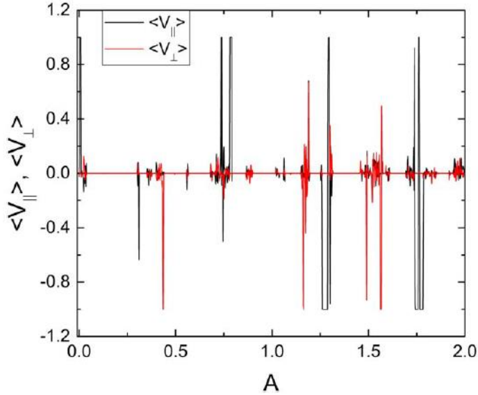
Figure 8.14 – The average velocities \langle V_{\parallel} \rangle and \langle V_{\perp} \rangle as a function of the ac drive amplitude A and fixed B = 1.0 , using \alpha_m/\alpha_d = 1.732 and a_o = 0.65 . (From Vizarim et. al. [189], pg. 12).
