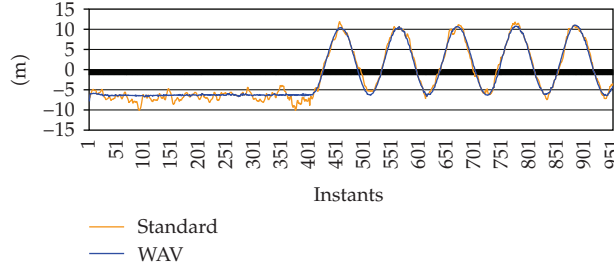
Figure 8: Pseudorange DD 14-01 observations in the Standard and WAV strategies.
