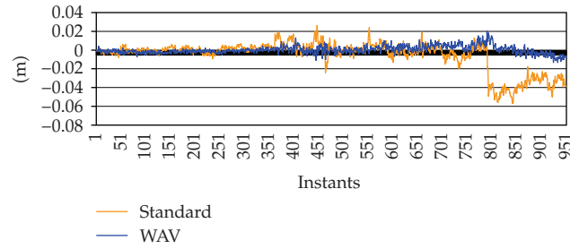
Figure 24: CP DD 14-03 residuals in the Standard and WAV strategies.
