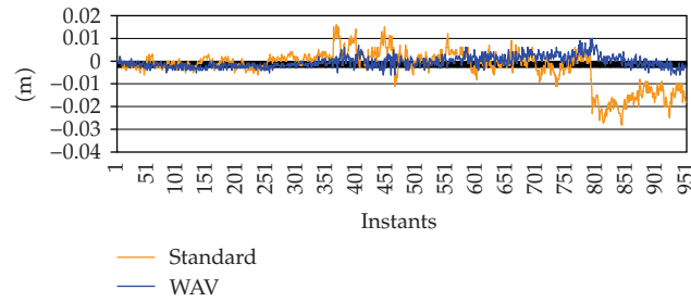
Figure 25: CP DD 14-18 residuals in the Standard and WAV strategies.
