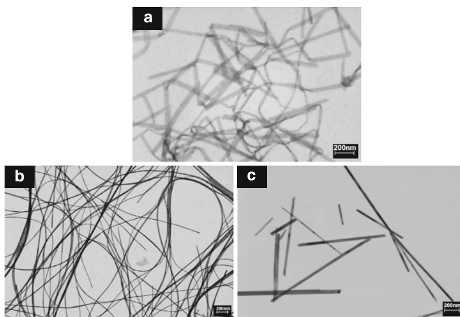
Figure 3 FE-STEM images of a 1D V_2O_5 \cdot nH_2O nanostructures synthesized. (a) 160°C, (b) 180°C and (c) 200°C.
