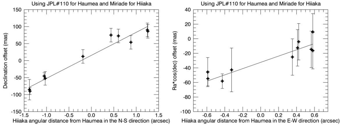
Figure 4: Residuals of the astrometric data to Haumea's orbit versus the angular separation of Hi'iaka with respect to Haumea obtained from the Miriade service. Each point corresponds to the median of the residuals obtained per night per telescope. The line depicts a linear fit to the data points.
