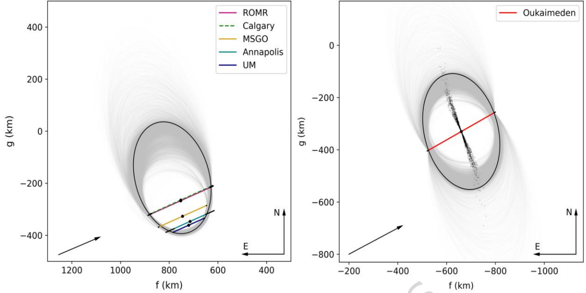
Figure 3 Chords and projected ellipses from the ellipsoidal fits to Hi'iaka's shape as observed during the two stellar occultations, shown with respect to the offsets between Hi'iaka's observed positions and its predicted positions from the Miriade ephemeris combined with Haumea's JPL#110 orbit. Left panel: The black ellipse represents the best fit to the positive chords from the stellar occultation on April 16 th using least-squares minimization. The gray shaded region represents the solutions from the Monte Carlo simulations. The black arrow at the bottom shows the direction of the body motion. The segments of different colors correspond to the chords from the observing sites indicated in the legend (using the nomenclature of Table 2). Right panel: The single positive chord from the occultation on April 6 th is shown (red line) fitted to the ellipses obtained after projecting the 3D model to the corresponding rotational phase at the moment of the April 6 th occultation. The small black dots indicate the center of the ellipses. In both panels the errors of the chords are present but may be too small to see.
