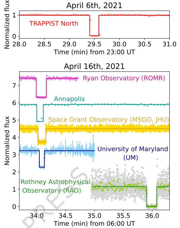
Figure 2 Light curves of the positive detections from April 6 th (top panel) and April 16 th (bottom panel), 2021. Observational data are represented by colored points with their corresponding uncertainties in the same color, with the exception of RAO for which the standard deviation of the data was used as the uncertainty. The error bars for the Annapolis data are smaller than the symbol size and therefore not visible in the figure. The square-well fit models for each light curve describing the occultation of the star are depicted by the solid, colored lines. In the bottom panel, offsets have been applied in the y-axis for clarity. Light curves are plotted in time as seen from each observatory. No residual flux is seen during the occultation.
