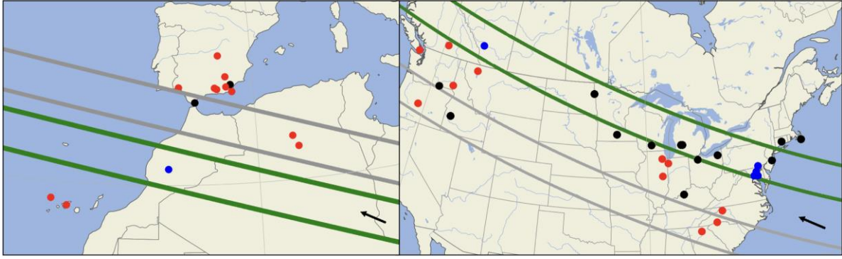
Figure 1 Maps showing the locations of the observatories involved in the observing campaigns on April 6 th (left) and 16 th (right). Blue dots indicate positive detections of the stellar occultation, red dots indicate no detection of the stellar occultation, and black dots indicate no observations due to bad weather or technical problems. Green lines indicate the final shadow path of Hi'iaka considering the respective projected diameter for each event (370 and 360 km for the left and right plots, respectively) while the gray lines show the predicted path. The black arrows located at the bottom right corner of the maps depict the sense of motion of the shadow path. These maps were generated using the SORA package ( https://sora.readthedocs.io/latest/ ).
