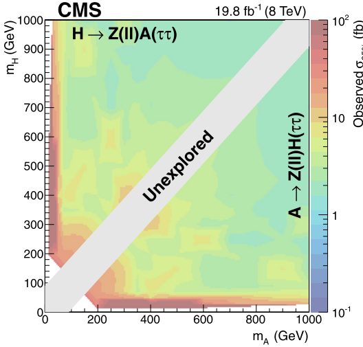
Fig. 4. Observed 95% CL upper limits on \sigma_{H/A \rightarrow Z A/H \rightarrow \ell\ell\tau\tau} as a function of m_A and m_H .
