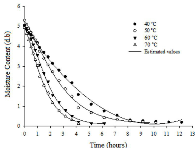
Figure 1. Foam-layer drying curves of cagaita pulp ( Eugenia dysenterica DC) at different temperatures.
