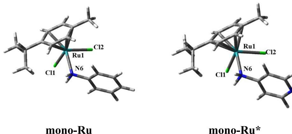
FIGURE 3 | DFT-optimized structures of the mono-Ru and mono-Ru* complexes.
