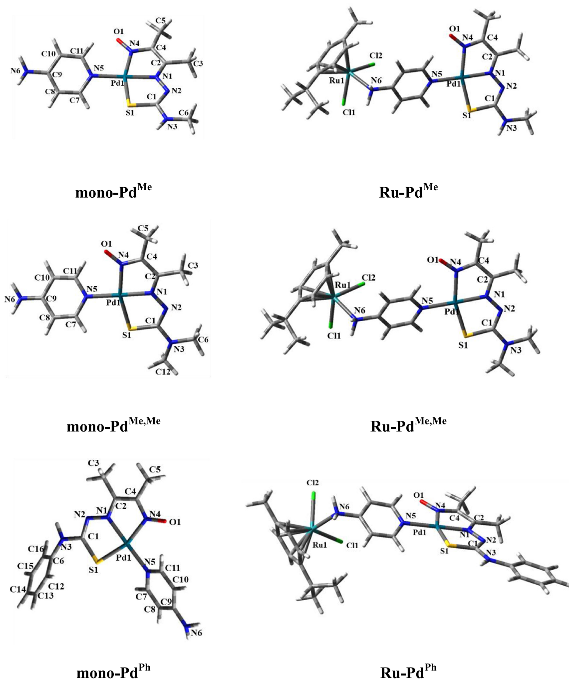
FIGURE 2 | DFT-optimized structures of mono-Pd L and Ru-Pd L complexes.
