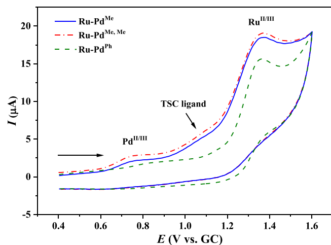
FIGURE 4 | Cyclic voltammograms of the Ru-Pd Me , Ru-Pd Me,Me , and Ru-Pd Ph complexes in DMSO at 25 \pm 0.1^\circ\text{C} vs. glassy carbon at a scan rate of 50 \text{ mV s}^{-1} ( [\text{Ru-Pd}^{\text{L}}] = 1 \text{ mM} , [\text{n-Bu}_4\text{NPF}_6] = 0.1 \text{ M} ).
