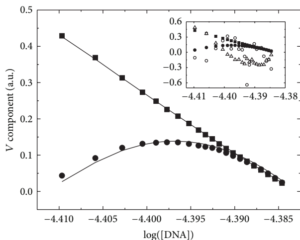
FIGURE 3: V component amplitude as a function of the total DNA concentration. Data were generated from the SVD matrix of the ActD-DNA titration data. The squares show the first V component values, and circles represent the second-component amplitudes. The first four V component amplitudes are shown in the inset, and the results generated from the F matrix were adjusted to the experimental data using our SVD analysis routine and are shown by the solid lines.
