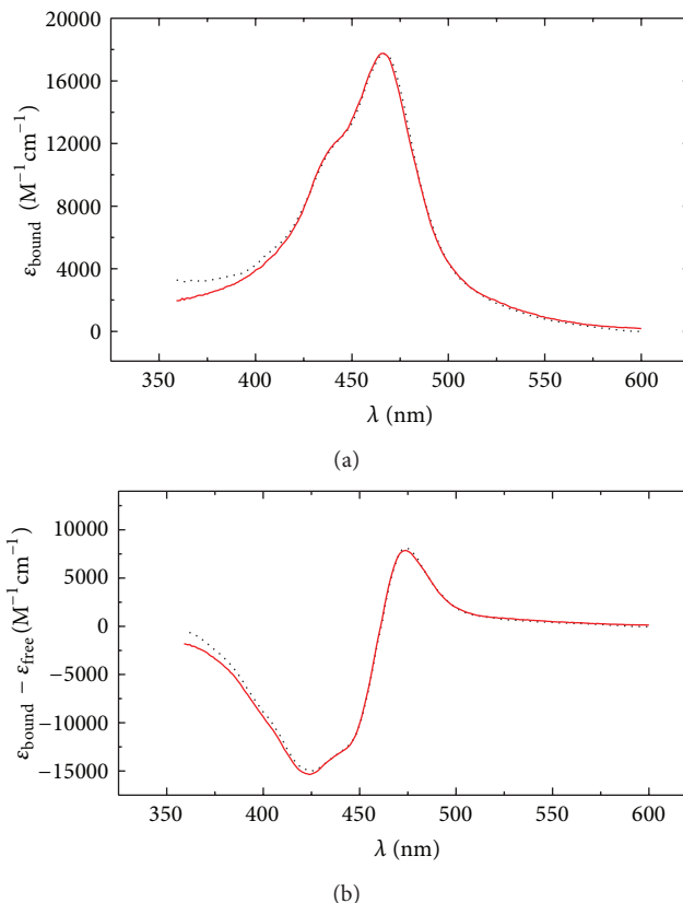
FIGURE 10: The (\epsilon_B - \epsilon_F) and \epsilon_B spectra determined using SVD-based binding analysis compared with directly measured coefficients. The solid lines represent the measured data, and the dash lines represent the results for extinctions coefficients determined by SVD and model fitting.
