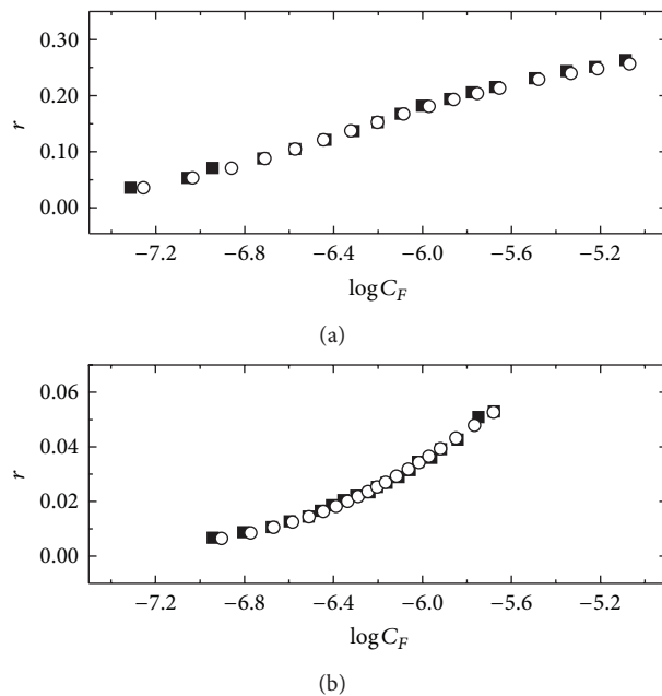
FIGURE 4: The rate number r (ratio of bound ligand concentration to DNA concentration) as a function of the free ligand concentration for ActD-DNA titration. The squares and circles represent the classical and SVD model fitting procedures, respectively.
