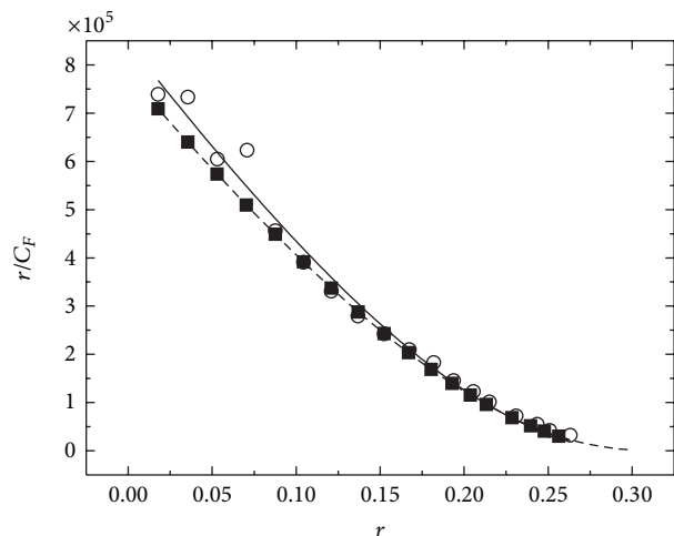
FIGURE 9: Scatchard plot of Daun-DNA binding. The squares and circles show SVD-based fitting and a traditional Scatchard plot, respectively. The standard noncooperative McGee and von Hippel model fitting parameters are K = 8.5 \pm 0.2 \times 10^5 \text{ M}^{-1} and n = 3.14 \pm 0.06 \text{ bp}/(\text{bound drug molecule}) while the SVD-based parameters for fitting are K = 7.79 \pm 0.05 \times 10^5 \text{ M}^{-1} and n = 3.0 \text{ bp}/(\text{bound drug molecule}) .
