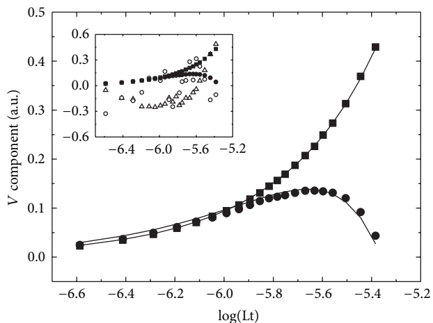
FIGURE 2: V component amplitude as a function of the total ActD concentration. The symbols represent values, of the SVD matrix for the ActD-DNA titration. The squares represent the first V component values and the circles represent the amplitudes of the second component. The first four V component amplitudes are shown in the inset, and the results generated from F matrix were adjusted to the experimental data according to SVD analysis routine (solid lines).
