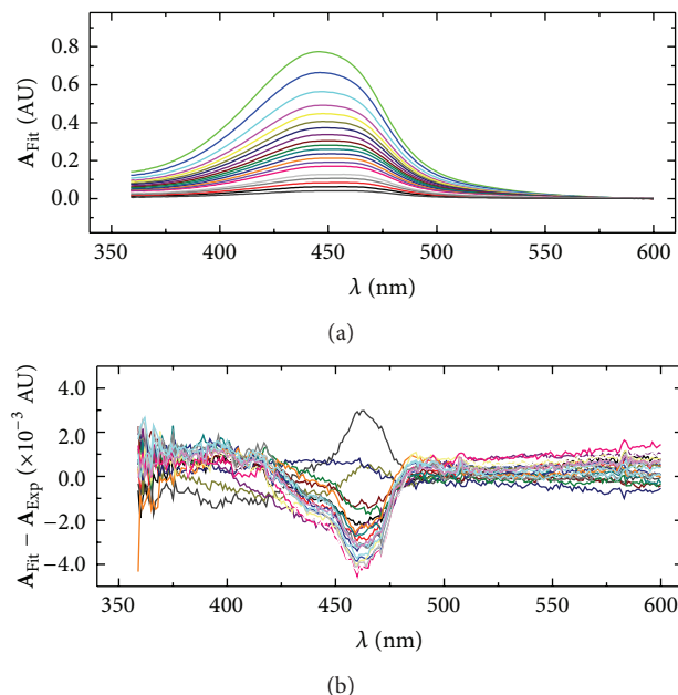
FIGURE 7: (a) Absorbance spectra recalculated using A_{\text{Fit}} = \mathbf{D}\mathbf{F}^T , where \mathbf{F} is given by the fitted model. (b) The residual absorbance spectra ( A_{\text{Fit}} - A_{\text{Exp}} ) of the difference between the recalculated and experimental spectra.
