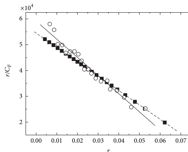
FIGURE 8: Scatchard plot of ActD-DNA binding. The squares and circles represent the SVD binding and standard procedures, respectively. The one-site model fitting using the Scatchard plot gives K = 7.0 \pm 0.5 \times 10^5 \text{ M}^{-1} and n = 12 \pm 1 \text{ bp}/(\text{bound drug}) , while the SVD binding analysis gives K = 5.57 \pm 0.07 \times 10^5 \text{ M}^{-1} and n = 10 \text{ bp}/(\text{bound drug}) .
