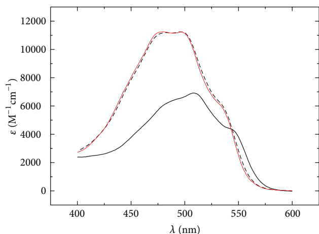
FIGURE 6: Free (dashed line) and bound (solid line) molar extinction coefficient spectra determined by the SVD fitting model for Daun compared with free DNA-Daun sample extinction coefficient spectra (soft solid line).
