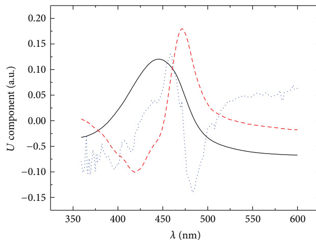
FIGURE 1: The first three U component spectra in sequence: solid, dashed, and dotted lines for the SVD of binding of Act-D-DNA spectrophotometric titration data.
