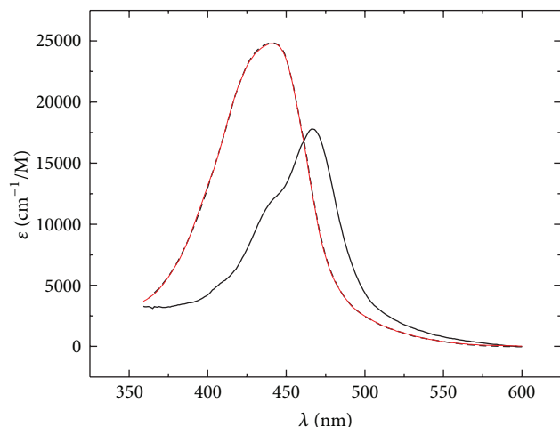
FIGURE 5: Free (dashed line) and bound (solid line) molar extinction coefficient spectra determined by the SVD fitting model for ActD compared with the free DNA-ActD sample extinction coefficient spectra (thin solid line).
