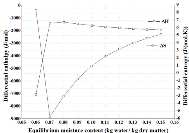
Fig. 4. - Calculated differential enthalpy and differential entropy of ora-pro-nóbis leaves as function of the equilibrium moisture content.
