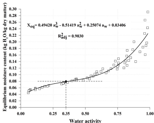
Fig. 2. - Determination of the optimal water activity for preservation of ora-pro-nóbis leaves.
