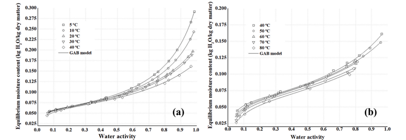
Fig. 1. Desorption isotherms of ora-pro-nóbis leaves at storage (a) and drying (b) temperatures.
