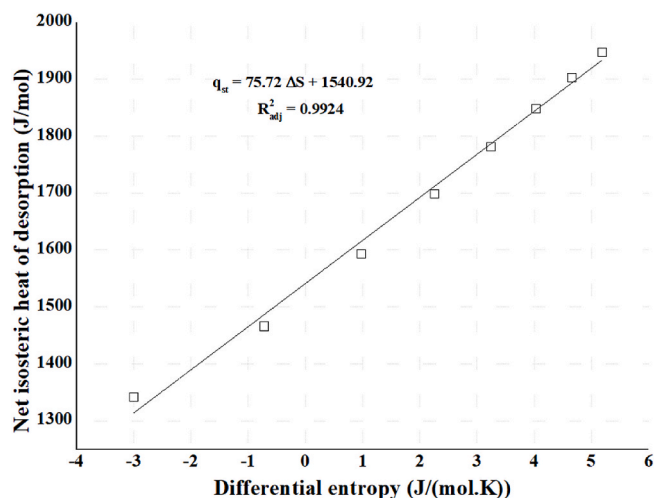
Fig. 5. - Linear relationship between net isosteric heat of desorption and entropy.
