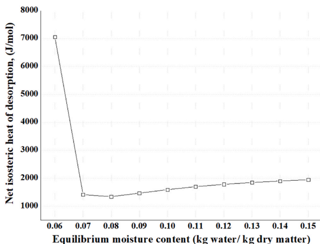
Fig. 3. - Calculated net isosteric heat of desorption of ora-pro-nóbis leaves as function of the equilibrium moisture content.
