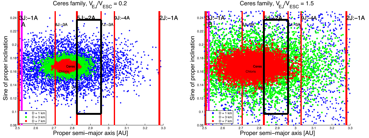
Figure 4. An (a, \sin(i)) distribution of D = 1, 3 , and 7 km members of Ceres families obtained using V_{EJ} = 0.2V_{ESC} (panel A) and V_{EJ} = 1.5V_{ESC} (panel B). The black box identify the orbital regions in which most of the D = 3 km fragments for V_{EJ} = 1.5 \cdot V_{ESC} and most of the D = 1 km for V_{EJ} = 0.2 \cdot V_{ESC} could be found in the pristine region of the main belt.
