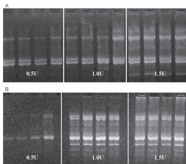
Figure 3. RAPD banding patterns obtained with Citrulus lanatus (A) and Sesamum indicum (B) in three different Taq polymerase enzyme concentrations (0.5, 1.0 and 1.5 U) using 40 ng DNA and 8 and 12 pmol of primer, respectively in 1.5% agarose gel stained with ethidium bromide for both tested DNA samples
