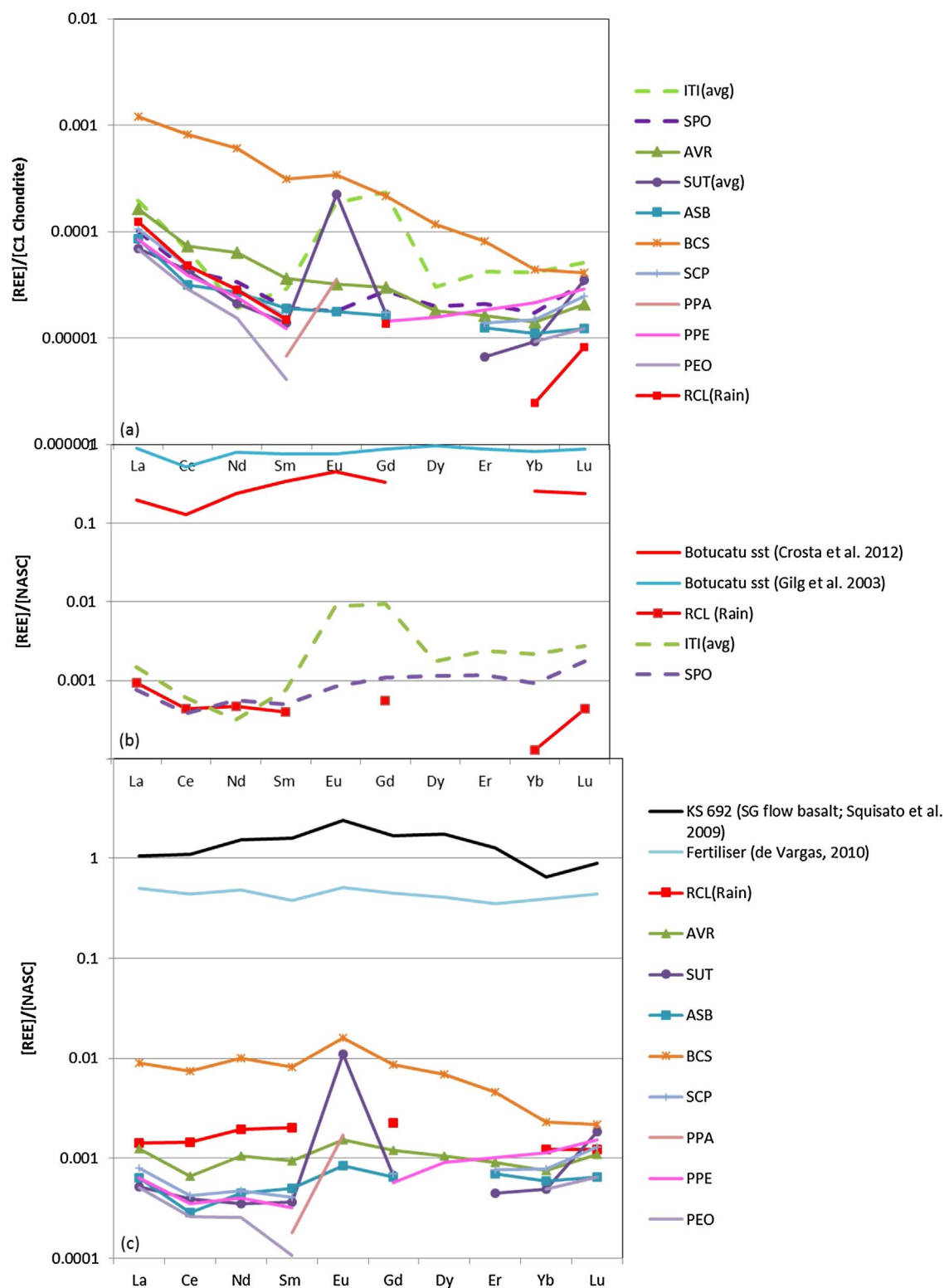
Fig. 5. Dissolved REE concentrations in sampled GAS waters normalised to (a) C1 chondrite (Anders and Grevesse, 1989), (b) and (c) North American Shale Composite (NASC) standard (Gromet et al., 1984). Additional data for comparison shows in (b) REE-signature attributed to the Botucatu Sandstone (sst) (Gilg et al., 2003; Crósta et al., 2012) and in (c) a Serra Geral flow basalt representative of the region (Squisato et al., 2009). Additionally, an NPK- fertiliser sample (de Vargas, 2010) has been included.
