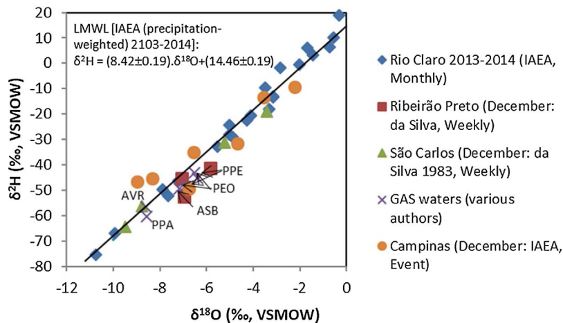
Fig. 3. Stable isotopes of water (‰ \delta^2\text{H} , \delta^{18}\text{O} with respect to Vienna Standard Mean Ocean Water, VSMOW) for monthly rainfall samples (diamonds) at Rio Claro (2013–2014) and event waters for December 1997 from Campinas station (circles) in São Paulo State. Data are taken from the Global Network of Isotopes in Precipitation (GNIP) database of the International Atomic Energy Agency (IAEA). The Rio Claro data define the precipitation-weighted Local Meteoric Water Line (LMWL). Relevant weekly rainfall samples from Ribeirão Preto (squares) and São Carlos (triangles) (da Silva, 1983) also have been included. Additionally, GAS groundwater signatures (crossed symbol) for sites Avaré (AVR), Águas de Santa Bárbara (ASB), Paraguaçu Paulista (PPA), Presidente Epitácio, Presidente Prudente have been included (da Silva, 1983; Kimmelman et al., 1994; Gastmans et al., 2010a) for comparison.
