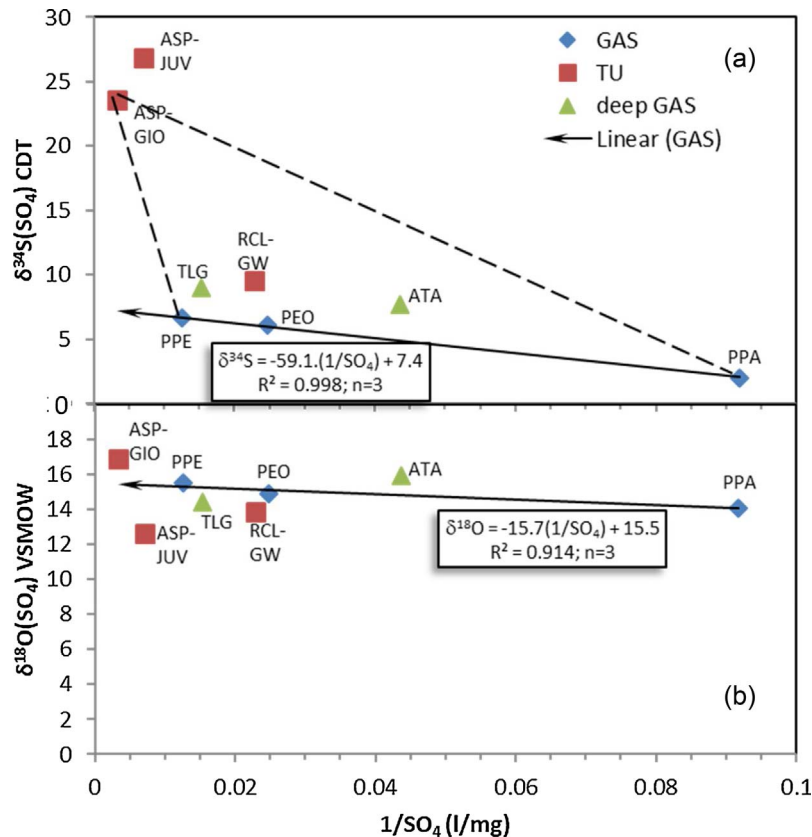
Fig. 9. Two-component mixing diagram (cross-plot) for sulfur isotope systematics ( \delta^{34}\text{S} , \delta^{18}\text{O} ) of dissolved sulfate in the GAS of São Paulo State. (a) \delta^{34}\text{S} (‰ with reference to the standard Canyon Diablo Troilite, CDT) versus reciprocal sulfate concentration (weight); (b) \delta^{18}\text{O} (‰ with reference to VSMOW) versus reciprocal sulfate concentration (weight). The relevant GAS sites (diamonds) have been identified alongside other deep GAS (triangles) and TU (squares) sites. Data are taken from Soler i Gil and Bonotto (2015) . Borehole construction details for other relevant GAS sites are: ASP-JUV: unlined in Sao Bento (0–45 m), PD (45–240 m), TU (240–469) Groups; ASP-GIO: details unknown; TLG lining details are unknown; ATA: unlined through SG (22–957 m), BO (957–1214 m); Rio Claro-GW: unlined through SG (0–62.4 m), PD (62.4–112.0 m), TU (112.0–198.5 m).
