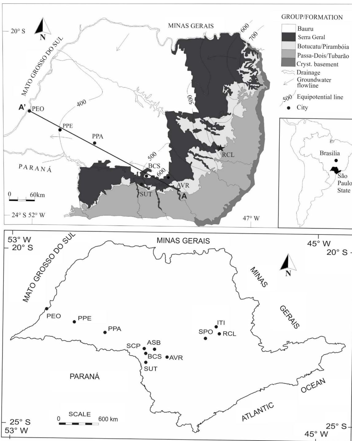
Fig. 1. (top) Simplified map modified from da Silva (1983) showing the outcrop and groundwater flow direction in the GAS, São Paulo State, Brazil, as well the transect AA' from Avaré up to Presidente Epitácio (SE-NW direction); the star symbol indicates the location of the rainwater sampling point (Rio Claro). (bottom) Location in São Paulo State of all sampling sites.
