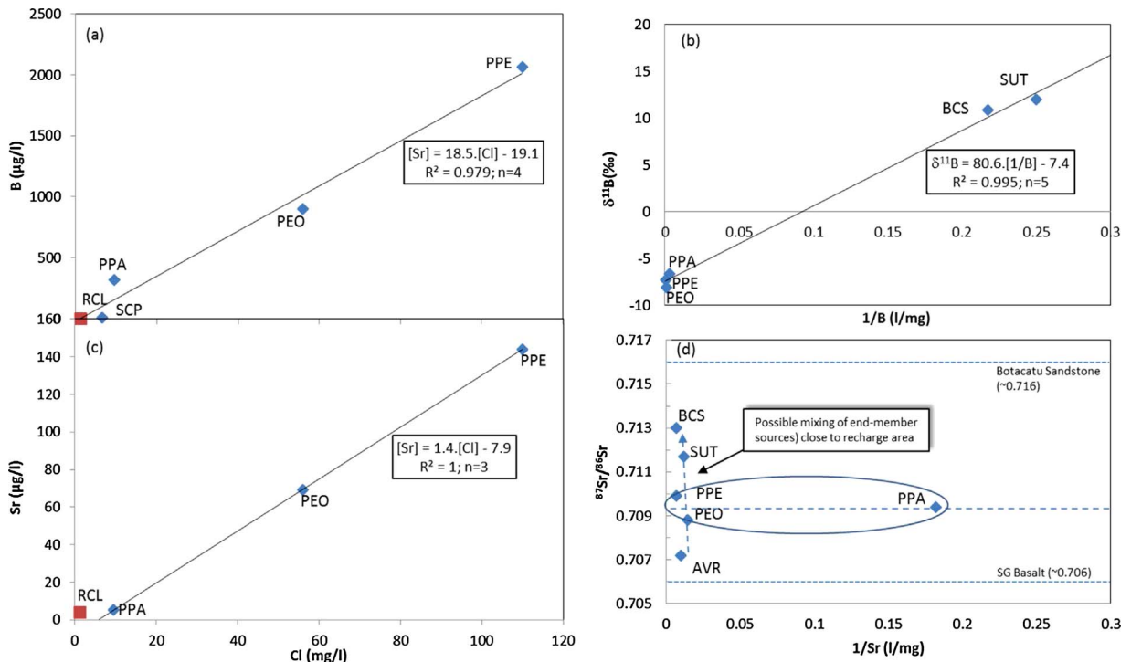
Fig. 7. Cross-plot mixing diagrams: (a) B versus Cl (weight); (b) \delta^{11}B versus reciprocal boron concentration (weight); The boron isotope values are with respect to NIST standard SRM 951; (c) Sr versus Cl (weight); (d) ^{87}Sr/^{86}Sr versus reciprocal strontium (weight). Particular GAS groundwater and rainfall (Rio Claro) sites are identified.
