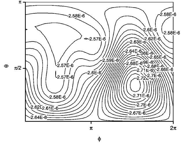
FIG. 2. Renormalized value of the vacuum 00 component of a conformally coupled massive scalar field \phi ( E = T_{\mu\nu} u^\mu u^\nu = T_{00} ) with a mass m = 0.5 in the static R \times \mathcal{M} space-time with R_{\text{CURV}} = 10 . The T_{00} is on a sphere of radius r = 0.6 , inside the fundamental polyhedron, Fig. 1, where r is given in Eq. (5).
