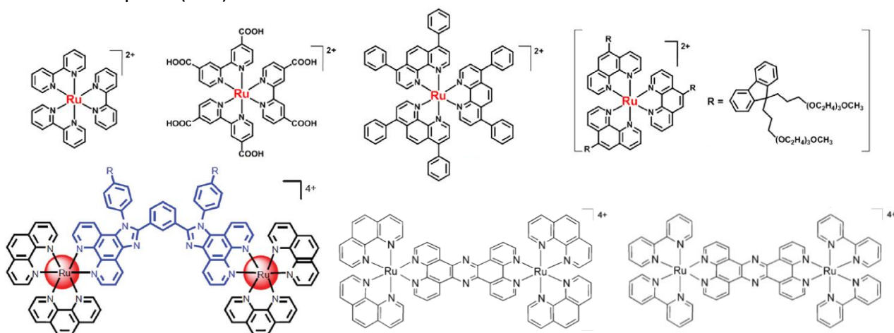
Figure 4. Chemical structures of some Ru(II) and dinuclear Ru(II)—Ru(II) complexes with Two-Photon Absorption (TPA). 40–42
