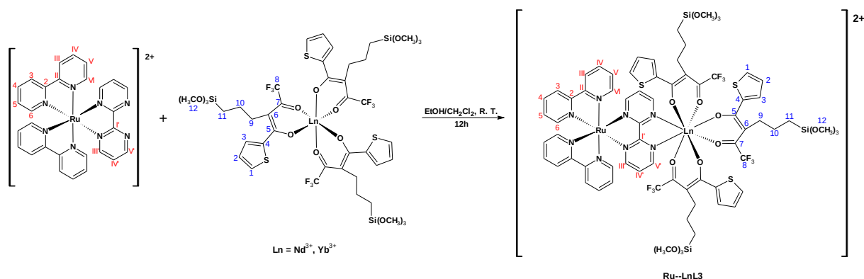
Figure 16. Synthetic route of the [Ru(bpy) 2 (bpmd)Ln(TTA-Si) 3 ]Cl 2 complex (Ru—LnL3).
