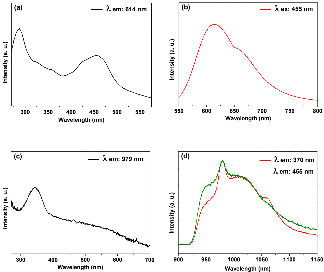
Figure 100. Room temperature excitation ((a), \lambda_{\text{emission}} : 614 nm and (c), \lambda_{\text{emission}} : 979 nm) and emission ((b), \lambda_{\text{excitation}} : 455 nm; and (d), \lambda_{\text{excitation}} : 370 and 455 nm) spectra from the SiO 2 d-YbRuL in solid state.
