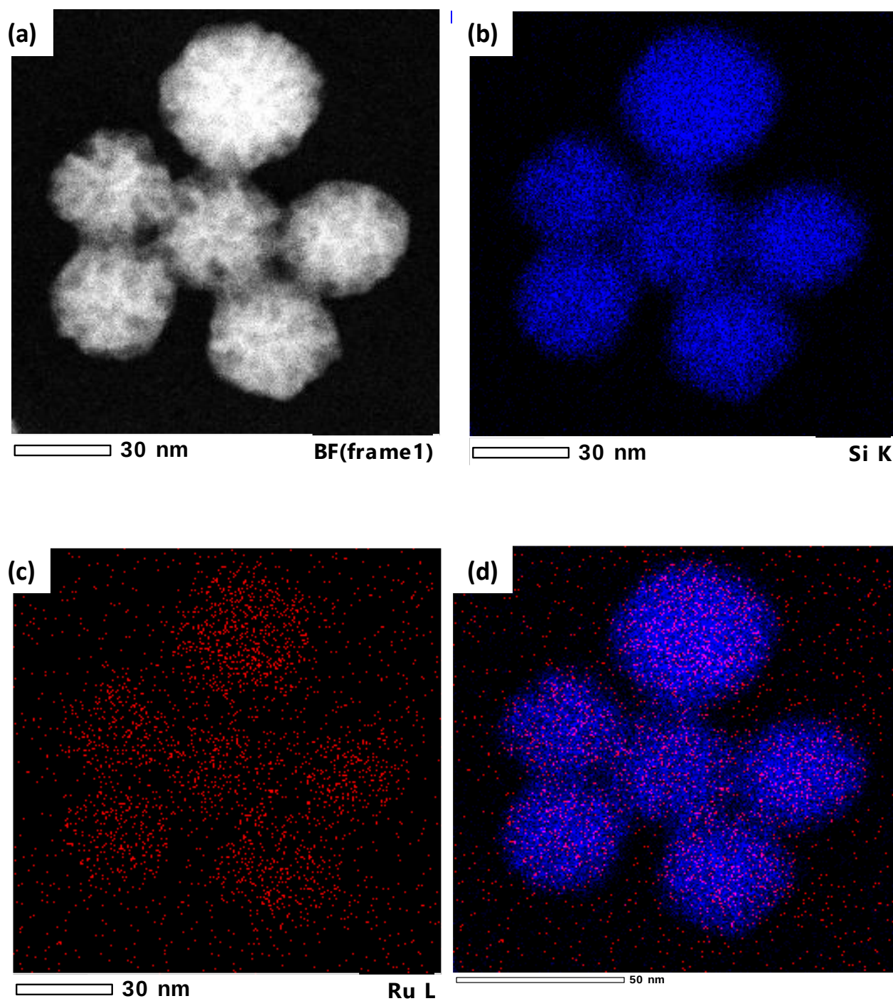
Figure 76. Electron microscope images and elemental cartography of the SiO 2 -Ru : (a) STEM image, (b) Si cartography, (c) Ru cartography and (d) Si (blue color) and Ru (red color) cartographies.
