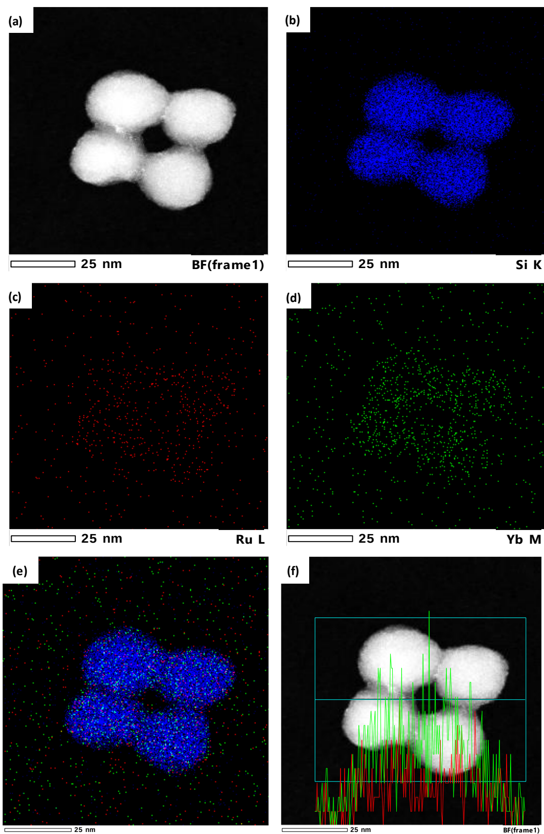
Figure 96. Electron microscope images and elemental cartography of the SiO 2 d-YbRuL : (a) STEM image, (b) Si cartography, (c) Ru cartography, (d) Yb cartography, (e) Si (blue color), Ru (red color) and Yb (green color) cartographies. (f) STEM image with a line profile of Ru (red line) and Yb (green line) atoms in the selected area (blue line).
