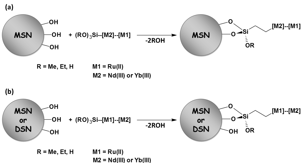
Figure 87. Representation of grafting reactions of (a) Ru—LnL3 complex onto MSNs and (b) Ln—RuL complexes onto MSNs and DSNs.
