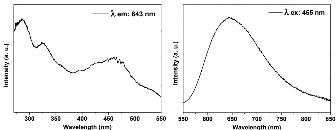
Figure 81. Room temperature excitation ( \lambda_{\text{emission}} = 643 \text{ nm} , on the left) and emission ( \lambda_{\text{excitation}} = 455 \text{ nm} , on the right) spectra from the SiO 2 -Ru complex in solid state.
