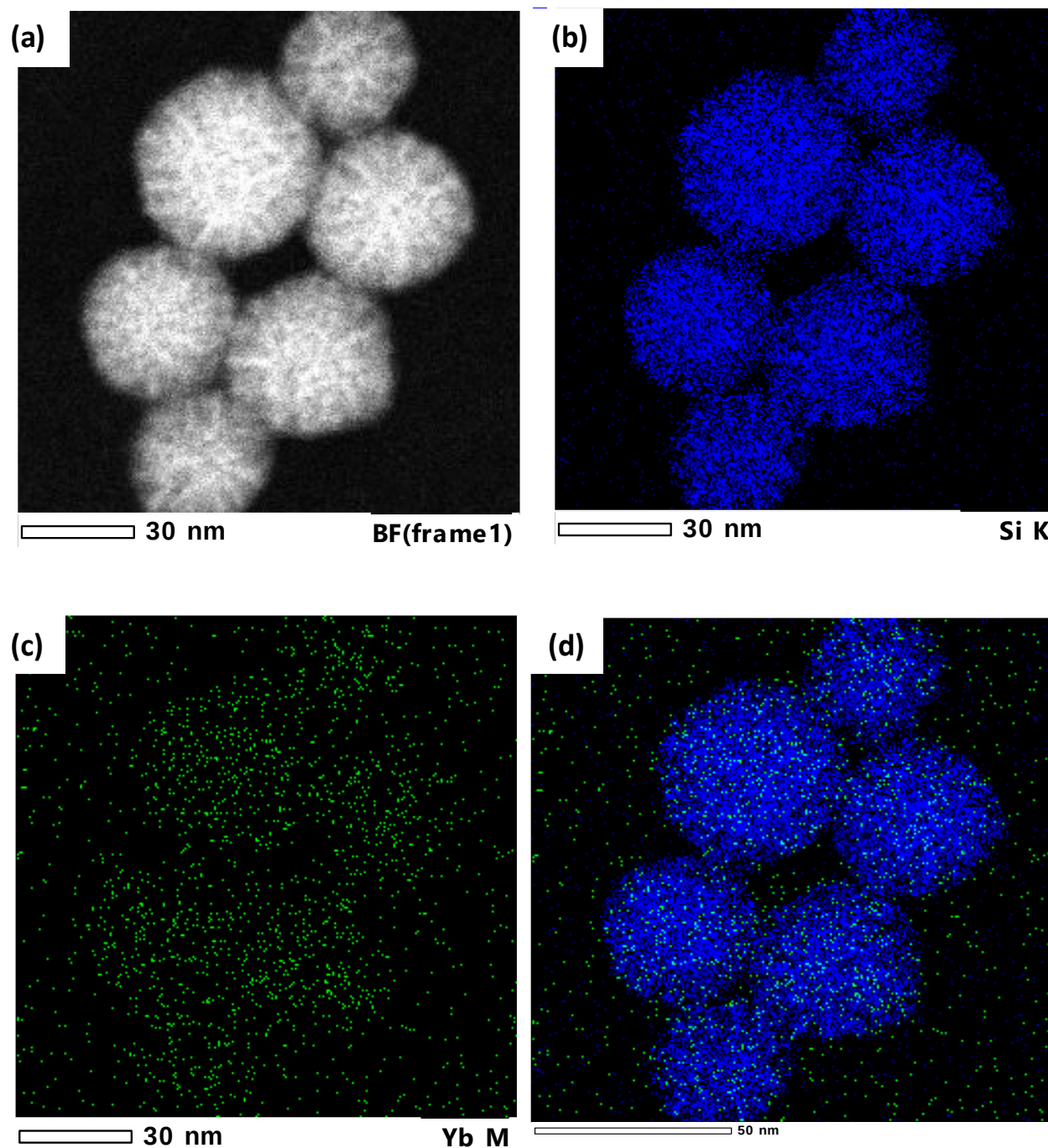
Figure 78. Electron microscope images and elemental cartography of the SiO 2 -Yb : (a) STEM image, (b) Si cartography, (c) Yb cartography and (d) Si (blue color) and Yb (green color) cartographies.
