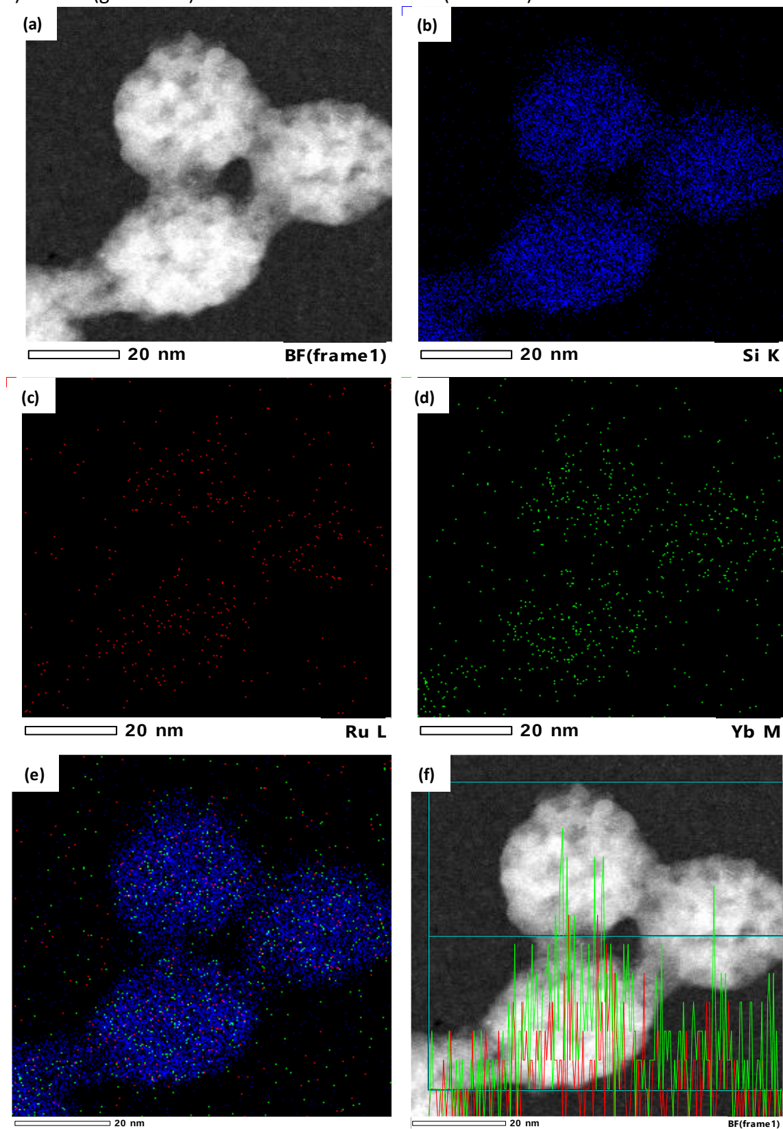
Figure 93. Electron microscope images and elemental cartography of the SiO 2 -RuYbL3 : (a) STEM image, (b) Si cartography, (c) Ru cartography, (d) Yb cartography, (e) Si (blue color), Ru (red color) and Yb (green color) cartographies. (f) STEM image with a line profile of Ru (red line) and Yb (green line) atoms in the selected area (blue line).
