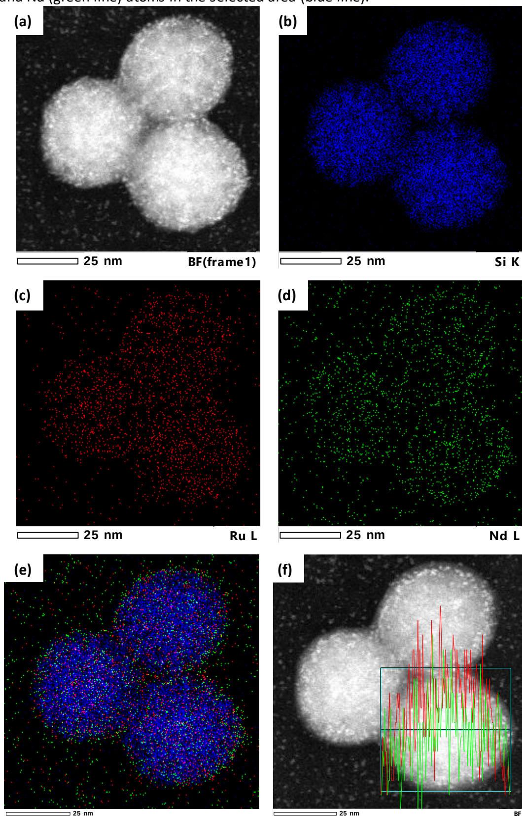
Figure 80. Electron microscope images and elemental cartography of the SiO 2 -RuNd : (a) STEM image, (b) Si cartography, (c) Ru cartography, (d) Nd cartography and (e) Si (blue color), Ru (red color) and Nd (green color) cartographies. (f) STEM image with a line profile of Ru (red line) and Nd (green line) atoms in the selected area (blue line).
