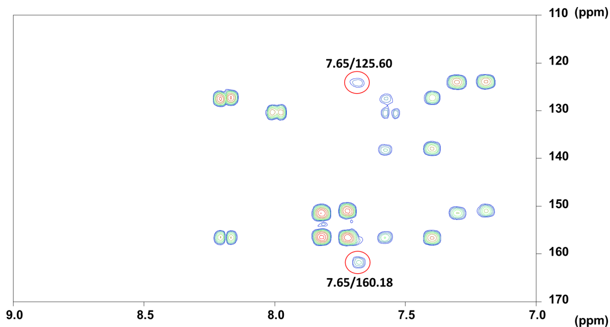
Figure 41. ^1\text{H}\{^{13}\text{C}\} -HMBC NMR spectrum of the Ru—NdL3 complex in the aromatic region (MeOD- d_4 , 600 MHz).
