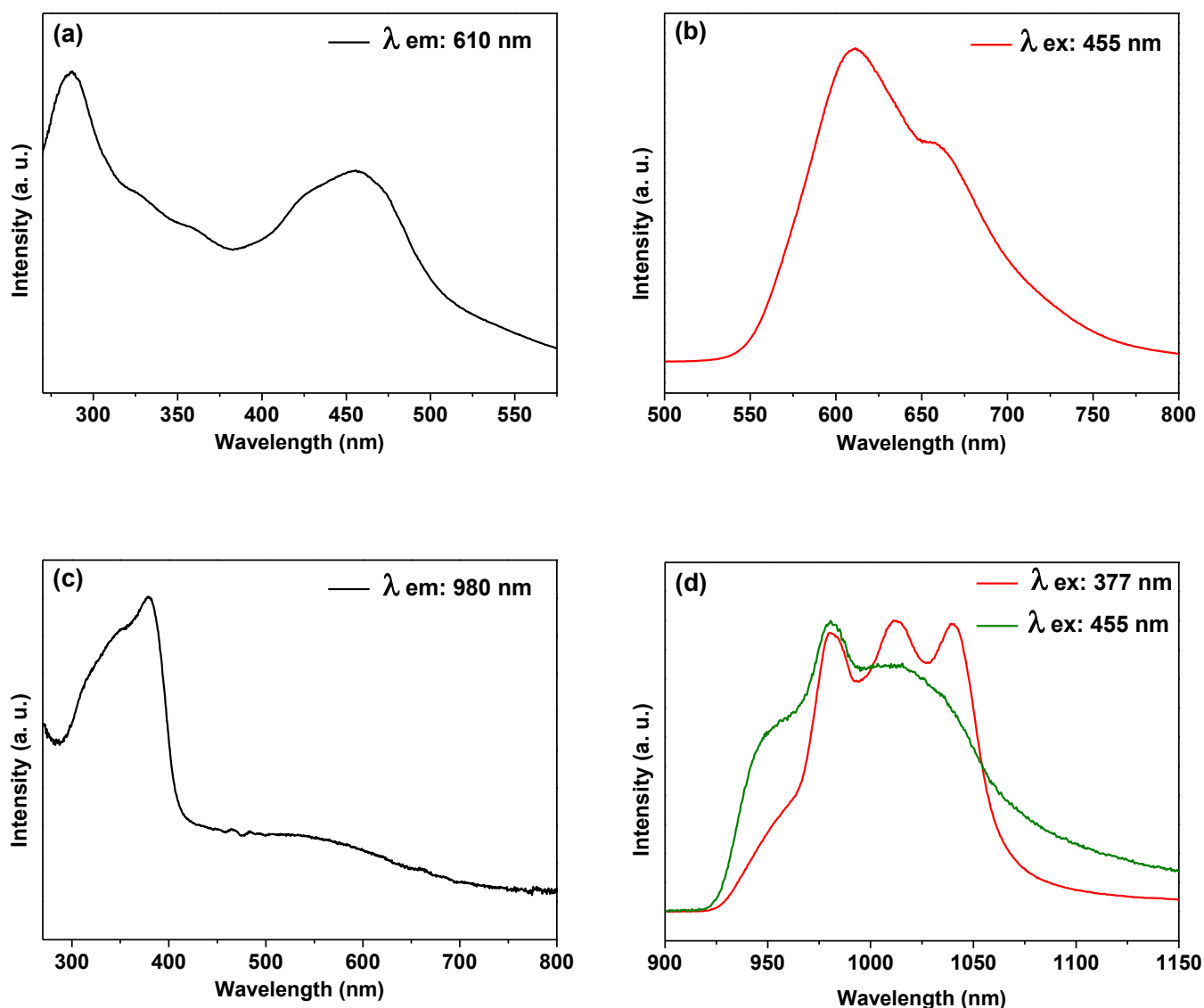
Figure 99. Room temperature excitation ((a), \lambda_{\text{emission}} : 610 nm and (c), \lambda_{\text{emission}} : 980 nm) and emission ((b), \lambda_{\text{excitation}} : 455 nm; and (d), \lambda_{\text{excitation}} : 377 and 455 nm) spectra from the SiO 2 -YbRuL in solid state.
