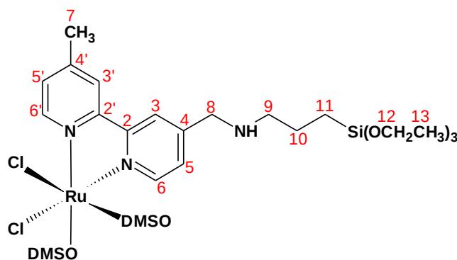
Figure 9. Structural representation of RuCl 2 DMSO 2 (bpy-Si) silylated complex.
