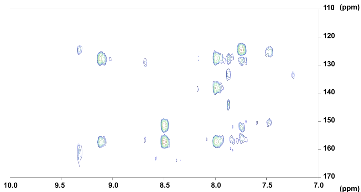
Figure 45. ^1H\{^{13}C\} -HMBC NMR spectrum of the Yb—RuL complex in the aromatic region (MeOD- d_4 , 600 MHz).
