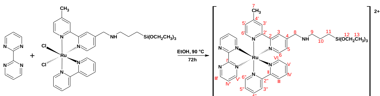
Figure 11. Synthetic route of the [Ru(bpy)(bpy-Si)(bpm d)]Cl_2 silylated complex ( RuL ).
