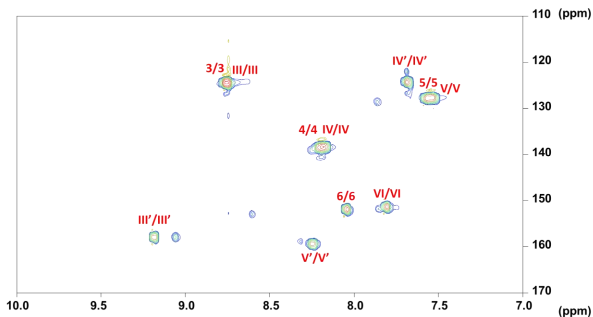
Figure 33. ^1\text{H}\{^{13}\text{C}\} HSQC NMR spectra of the Ru complex (MeOD- d_4 , 600 MHz) in the aromatic region. The numbering of C and H atoms is given for the complex and present in both spectra.
