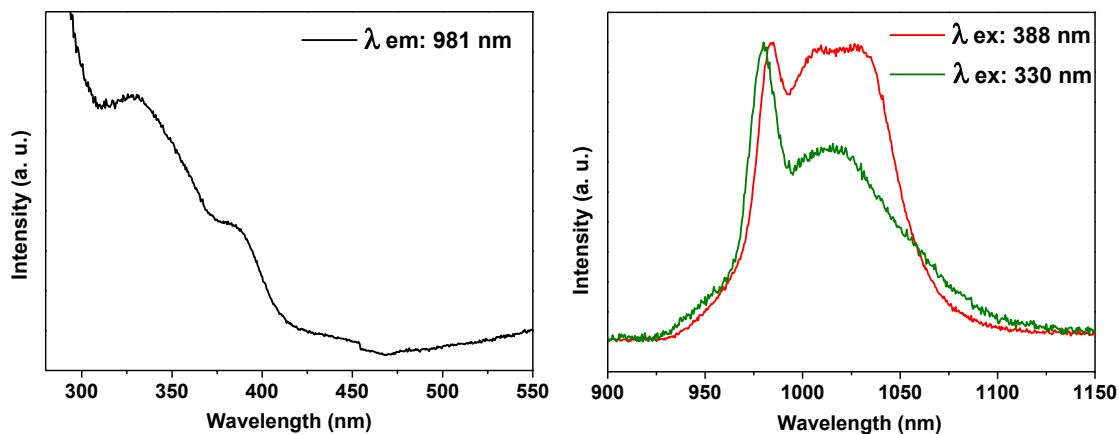
Figure 83. Room temperature excitation (on the left; \lambda_{\text{emission}} = 981 nm) and emission (on the right; \lambda_{\text{excitation}} = 330 and 388 nm; green and red lines, respectively) spectra from the SiO 2 -Yb complex in solid state.
