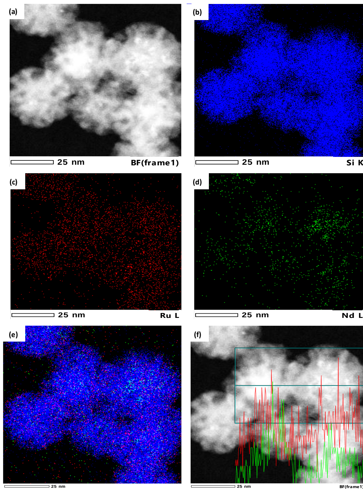
Figure 94. Electron microscope images and elemental cartography of the SiO 2 -NdRuL : (a) STEM image, (b) Si cartography, (c) Ru cartography, (d) Nd cartography, (e) Si (blue color), Ru (red color) and Nd (green color) cartographies. (f) STEM image with a line profile of Ru (red line) and Nd (green line) atoms in the selected area (blue line).
