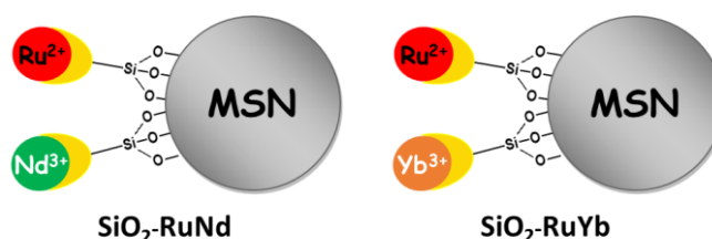
Figure 20. Representation of \text{SiO}_2\text{-RuNd} and \text{SiO}_2\text{-RuYb} nanohybrids.
