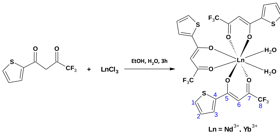
Figure 14. Synthetic route of the \text{Ln}(\text{TTA})_3\text{2H}_2\text{O} complex (Ln).
