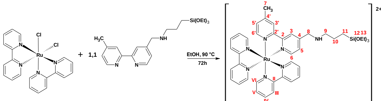
Figure 12. Synthetic route of the [\text{Ru}(\text{bpy})_2(\text{bpy-Si})]\text{Cl}_2 silylated complex ( RuL1 ).
