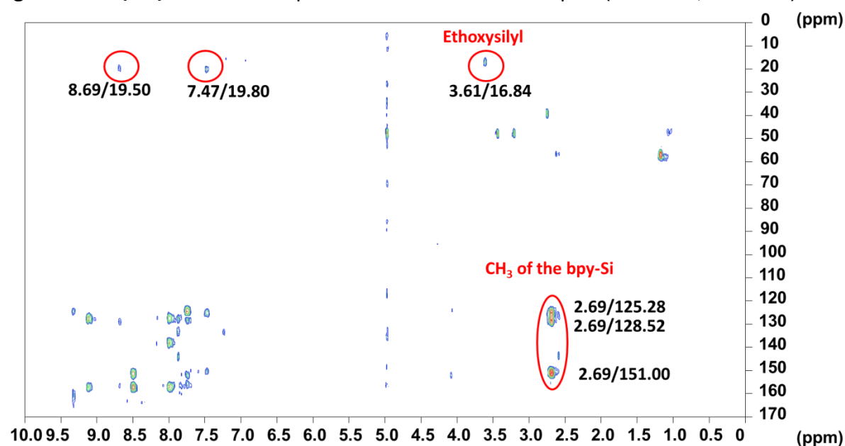
Figure 46. ^1H\{^{13}C\} -HMBC NMR spectrum of the Yb—RuL complex (MeOD- d_4 , 600 MHz).
