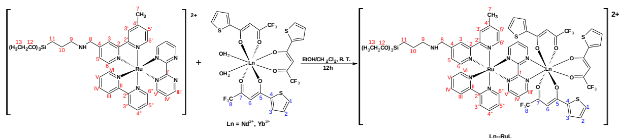
Figure 17. Synthetic route of the [Ru(bpy)(bpy-Si)(bpmd)Ln(TTA) 3 Cl 2 ] complex (Ln—RuL).
