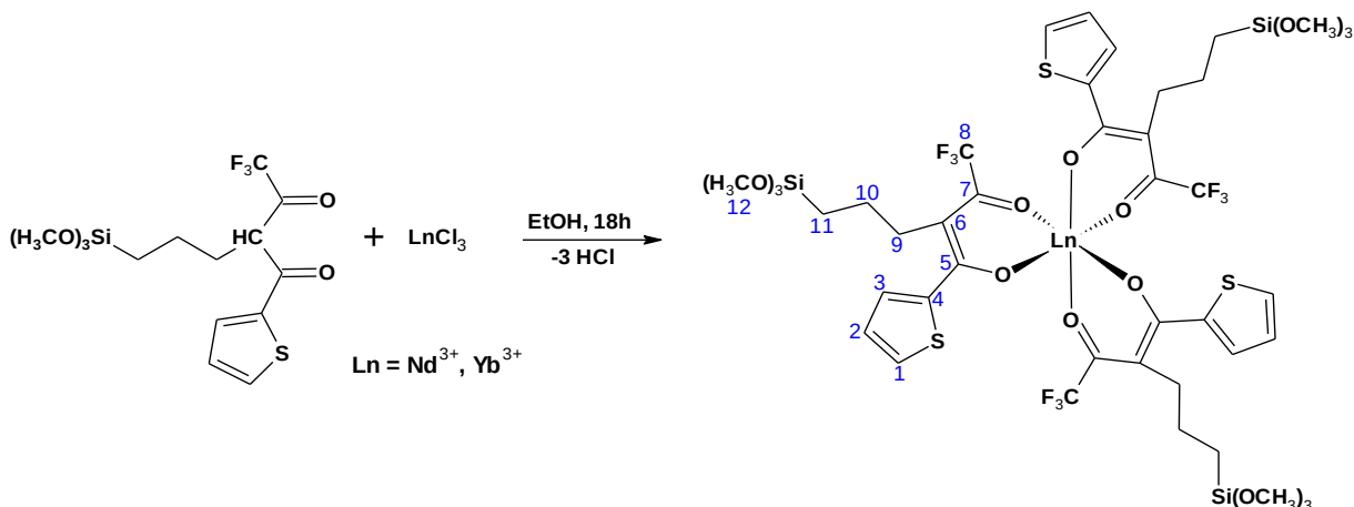
Figure 15. Synthetic route of the [\text{Ln}(\text{TTA-Si}(\text{OCH}_3)_3)] silylated complex ( LnL3 ).
