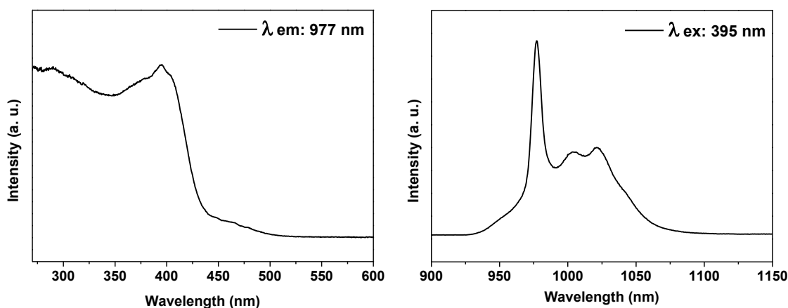
Figure 54. Room temperature excitation (on the left, monitoring at \lambda_{\text{emission}} = 977 nm) and emission (on the right, monitoring at \lambda_{\text{excitation}} = 395 nm) spectra from the Yb complex in solid state.
