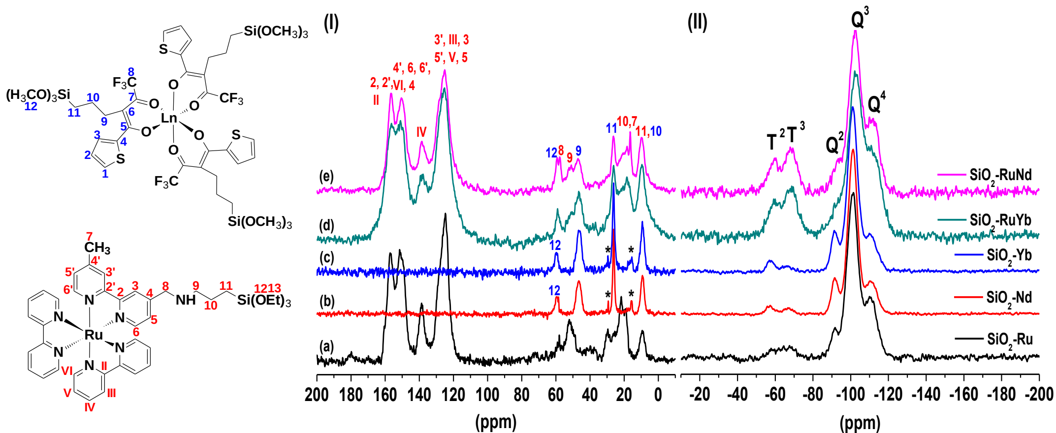
Figure 73. ^{13}\text{C}\{^1\text{H}\} CP-MAS NMR spectra (I) and ^{29}\text{Si}\{^1\text{H}\} CP-MAS NMR spectra (II) of (a) \text{SiO}_2\text{-Ru} , (b) \text{SiO}_2\text{-Nd} , (c) \text{SiO}_2\text{-Yb} , (d) \text{SiO}_2\text{-RuYb} and (e) \text{SiO}_2\text{-RuNd} . *: carbon atoms in residual ethanol groups. +: carbon atoms in methoxysilyl groups not grafted. The numbering of carbon atoms is given on the left side with Roman figures for the bipyridine ligands; Arabic numerals for the alkoxyisilane groups (methoxysilyl and ethoxysilyl).
