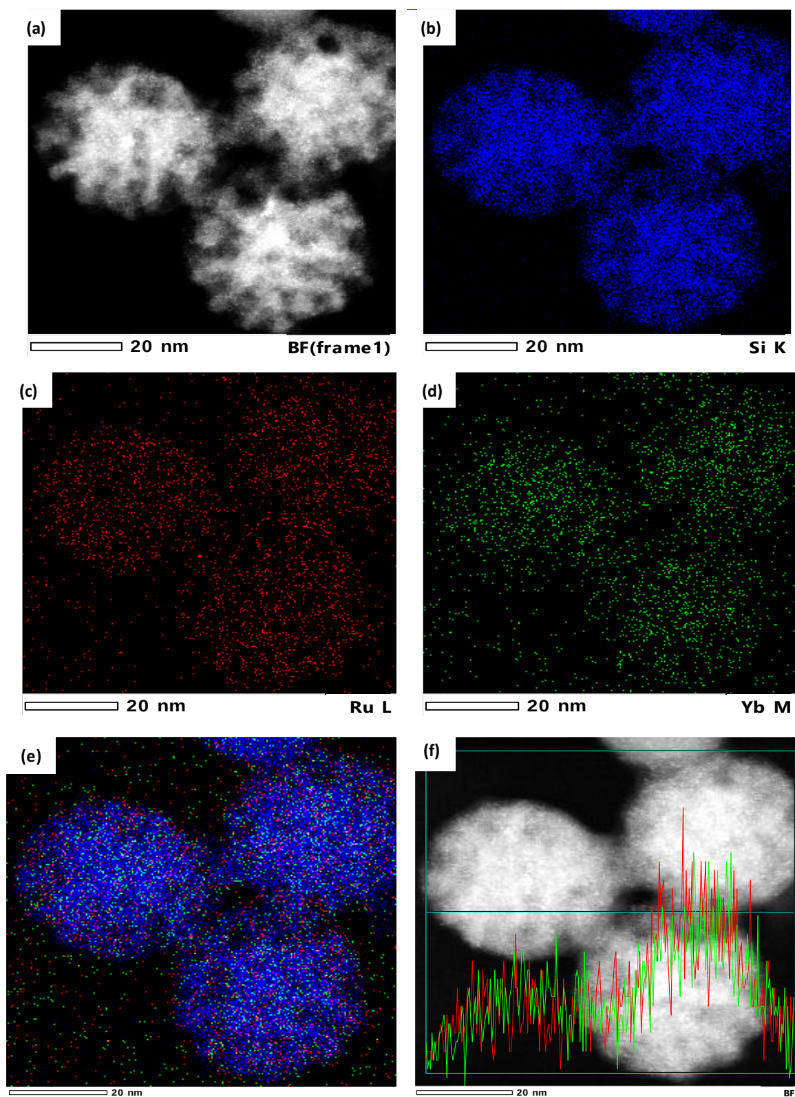
Figure 95. Electron microscope images and elemental cartography of the SiO 2 -YbRuL : (a) STEM image, (b) Si cartography, (c) Ru cartography, (d) Yb cartography, (e) Si (blue color), Ru (red color) and Yb (green color) cartographies. (f) STEM image with a line profile of Ru (red line) and Yb (green line) atoms in the selected area (blue line).
