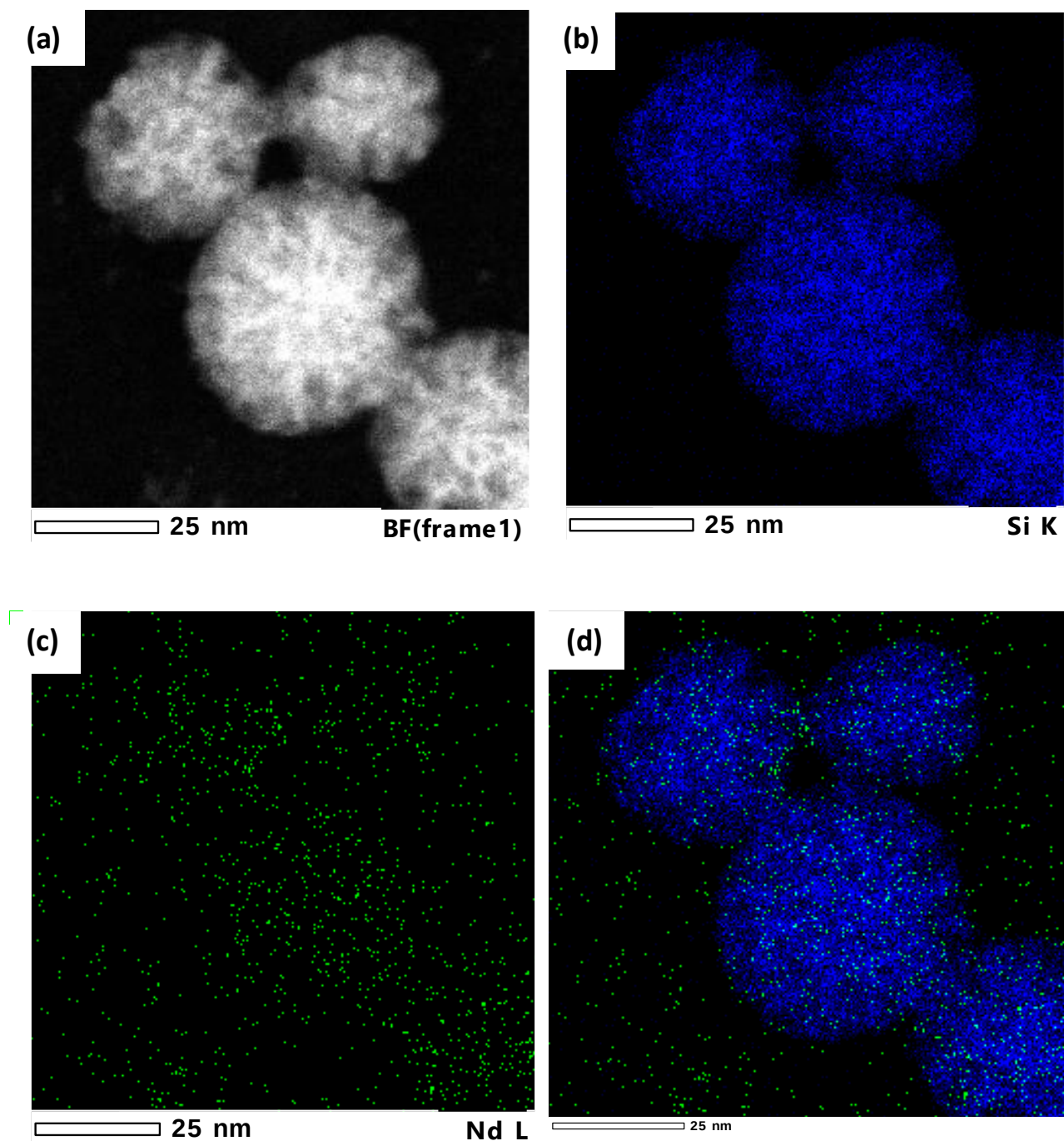
Figure 77. Electron microscope images and elemental cartography of the SiO 2 -Nd : (a) STEM image, (b) Si cartography, (c) Nd cartography and (d) Si (blue color) and Nd (green color) cartographies.
