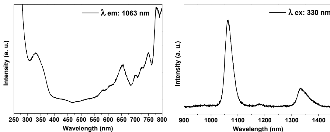
Figure 82. Room temperature excitation ( \lambda_{\text{emission}} = 1063 nm; on the left) and emission ( \lambda_{\text{excitation}} = 330 nm; on the right) spectra from the SiO 2 -Nd complex in solid state.
