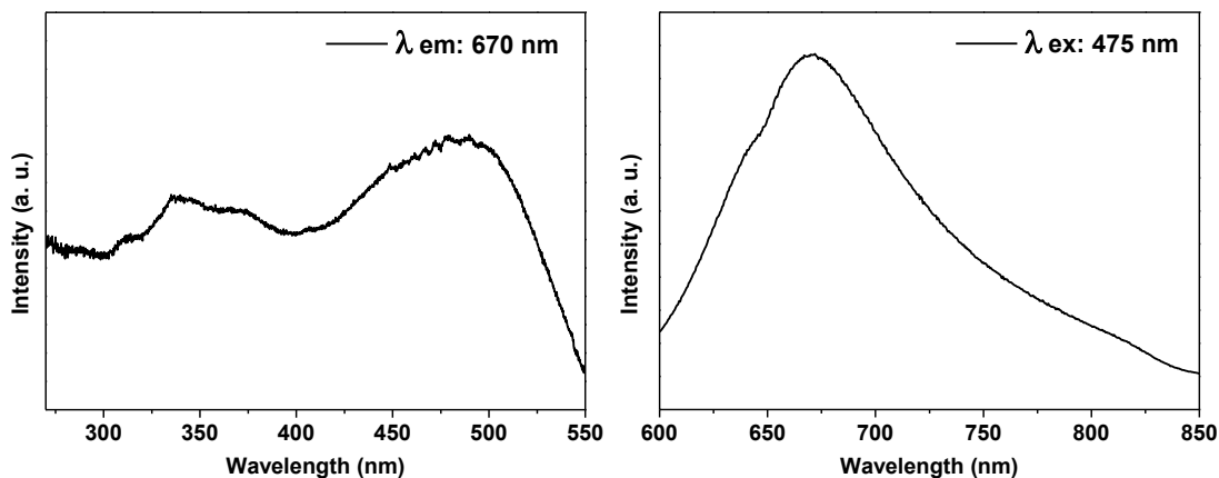
Figure 51. Room temperature excitation (on the left, monitoring at \lambda_{\text{emission}} = 670 \text{ nm} ) and emission (on the right, monitoring at \lambda_{\text{excitation}} = 475 \text{ nm} ) spectra from the Ru complex in solid state.
