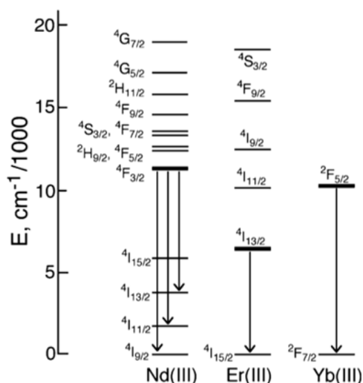
Figure 2. Representation of the diagram of the f–f energy levels of Nd(III), Er(III) and Yb(III) up to ca. 20,000 \text{cm}^{-1} . The energy levels from which NIR luminescence originates are marked in bold, and the main NIR emissions showed as descending arrows. Adapted from 25 .
