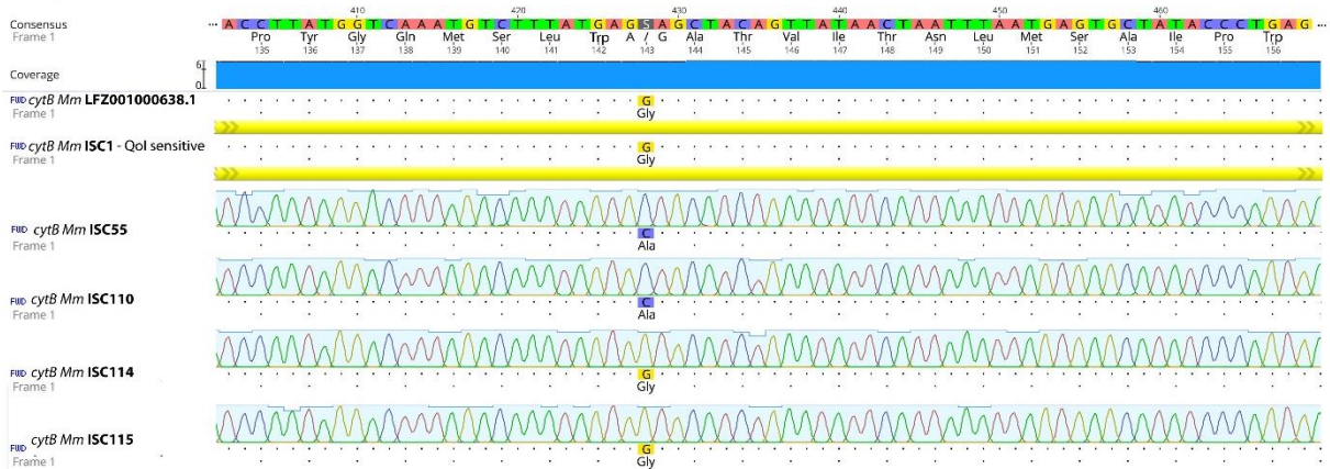
Figure 6. Graphical representation of the part of the cyt b gene from Mycosphaerella musicola (A), M. fijiensis (B) and M. thailandica (C) isolates containing the G428C mutation or not, resulting in the Gly143Ala amino acid substitution that confers resistance to Qol fungicides a, b, c .
