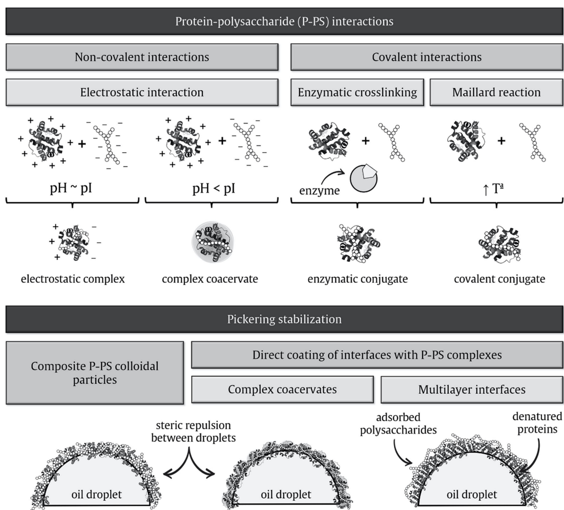
Figure 4.1.1 Schematic representation of both protein-polysaccharide non-covalent and covalent interactions and the different processes of Pickering stabilisation of these complexes and conjugates.
