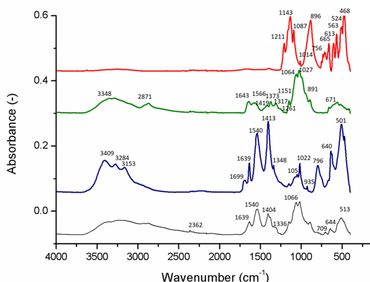
Figure 4.3.2 FT-IR spectra of sodium tripolyphosphate powder (TPP) ( — ), pure chitosan powder ( — ), chitosan nanoparticle at pH 6.7 (CN) ( — ) and chitosan-sodium tripolyphosphate nanoparticle (CN-TPP) ( — ) at CS:TPP mass ratio of 3:1.
