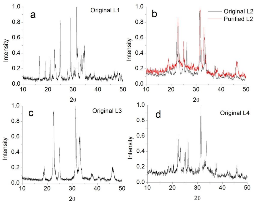
Fig. 3. XRD spectra of lignin ash
