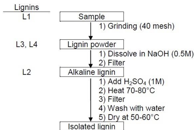
Fig. 1. Lignin isolation process
