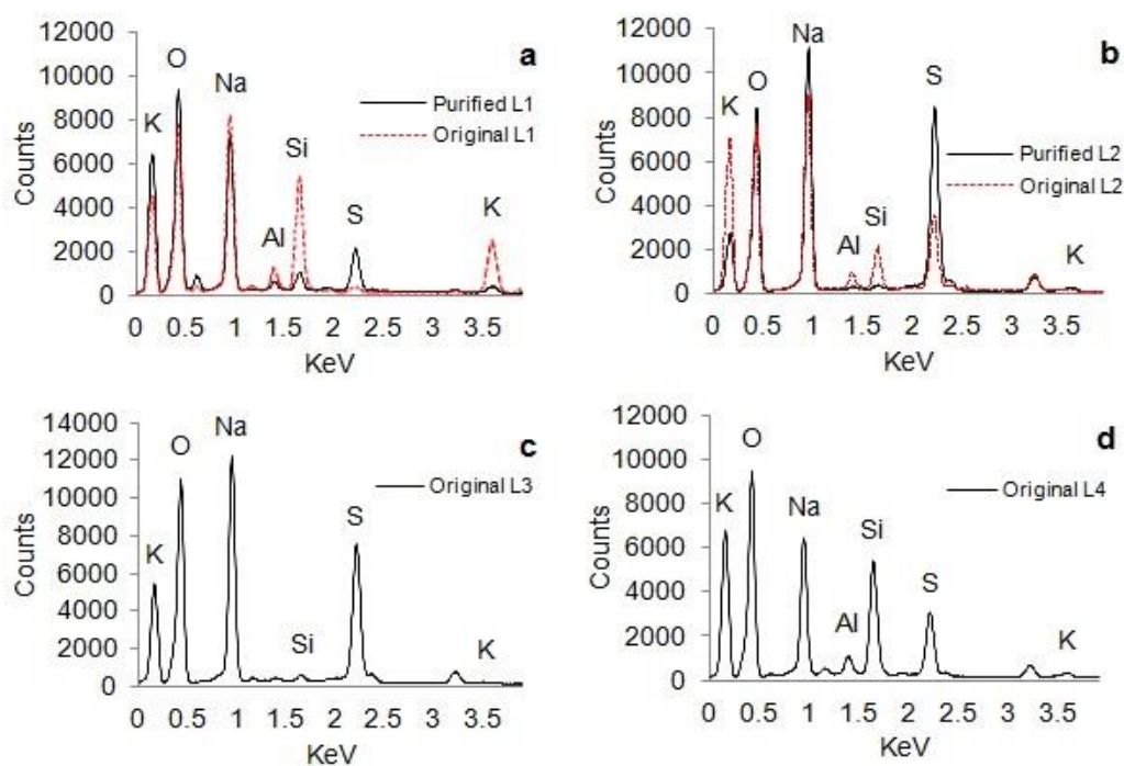
Fig. 2. EDS analysis of lignin ash
