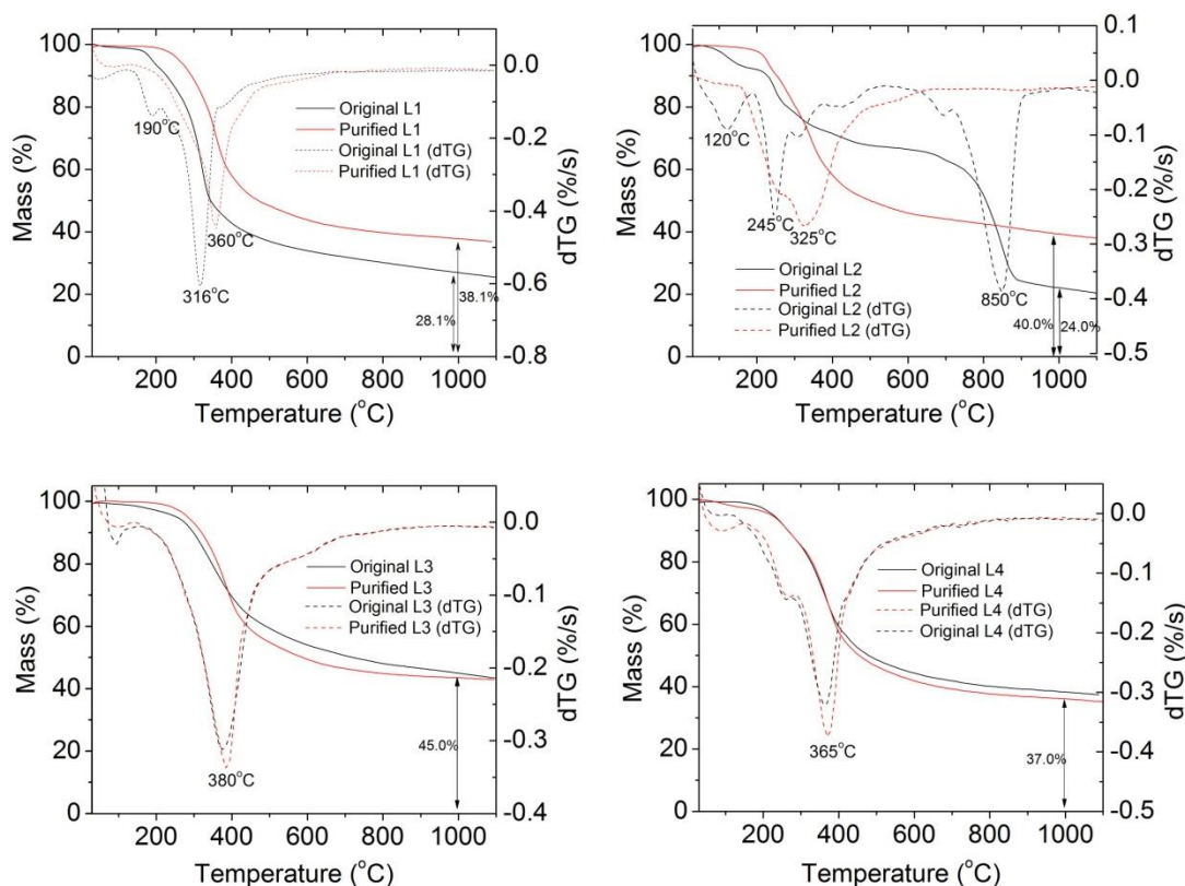
Fig. 4. TGA thermogram of original and purified lignin samples
