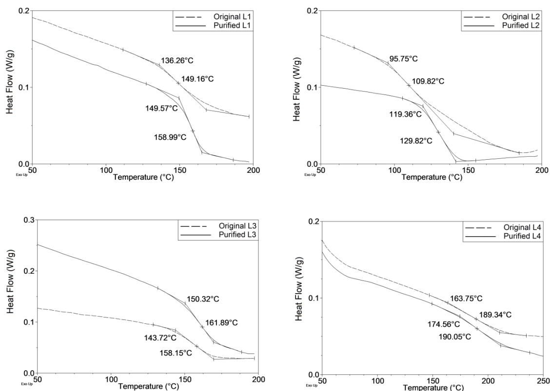
Fig. 5. DSC curves of lignin samples
