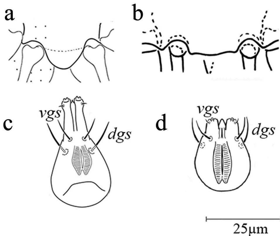
Figure 9. (a,b): Tegula of D. annonae and D. maryae , respectively; (c,d): Gnathosoma of D. esalqi and D. oliveirai , respectively.
