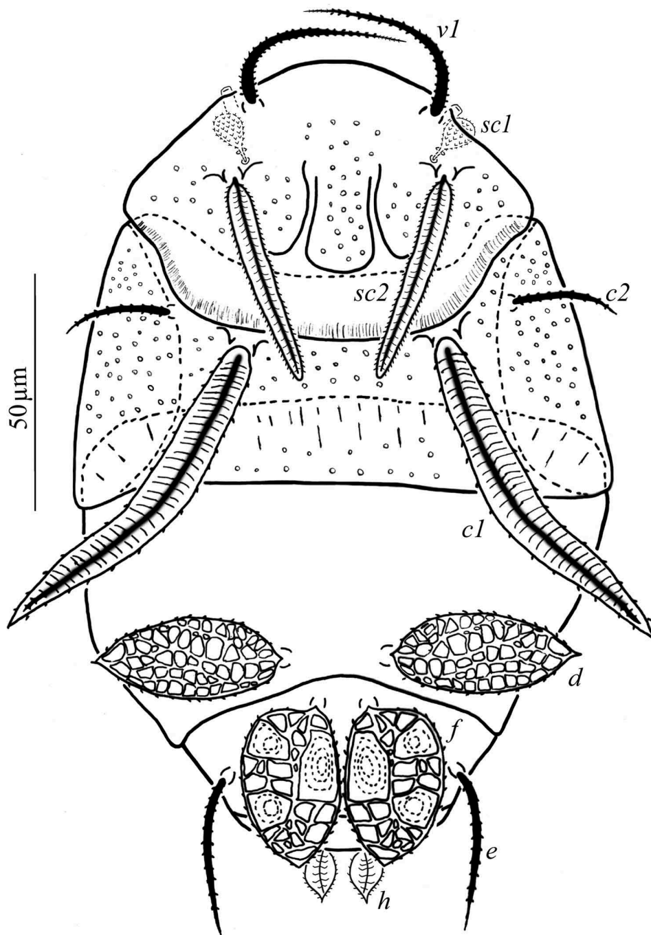
Figure 1. Excelsotarsonemus cabrucae sp. n. (female). Dorsal surface.
