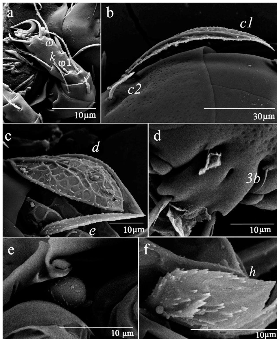
Figure 6. Excelsotarsonemus cabrucae sp. n. (female): (a) sensorial cluster of tibia I, (b) lateral view of the setae c1 and c2 , (c) lateral view of the setae d and e , (d) details of the tegula, (e) bothridial seta and stigma, and (f) details of the setae h .
