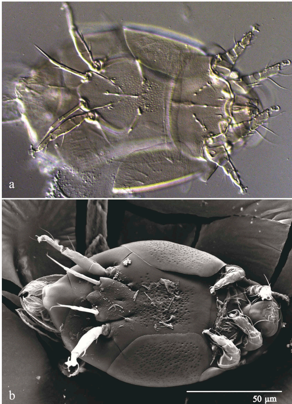
Figure 4. Excelsotarsonemus cabrucae sp. n. (female). Ventral micrographs: (a) differential interference contrast and (b) scanning electron microscopy.
