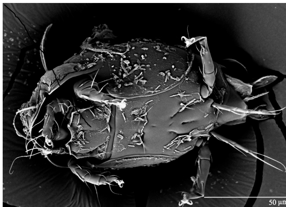
Figure 7. Presence of fungi and bacteria on part of lateral and ventral surface of the Excelsotarsonemus cabrucae sp. n.
