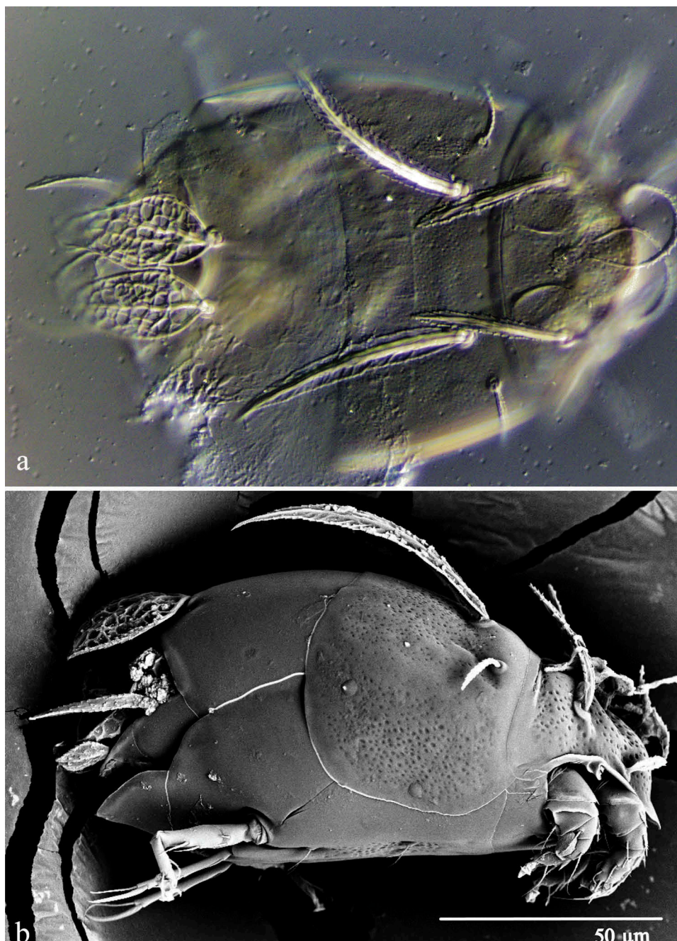
Figure 2. Excelsotarsonemus cabrucae sp. n. (female). Dorsal and lateral micrographs: (a) differential interference contrast and (b) scanning electron microscopy.
