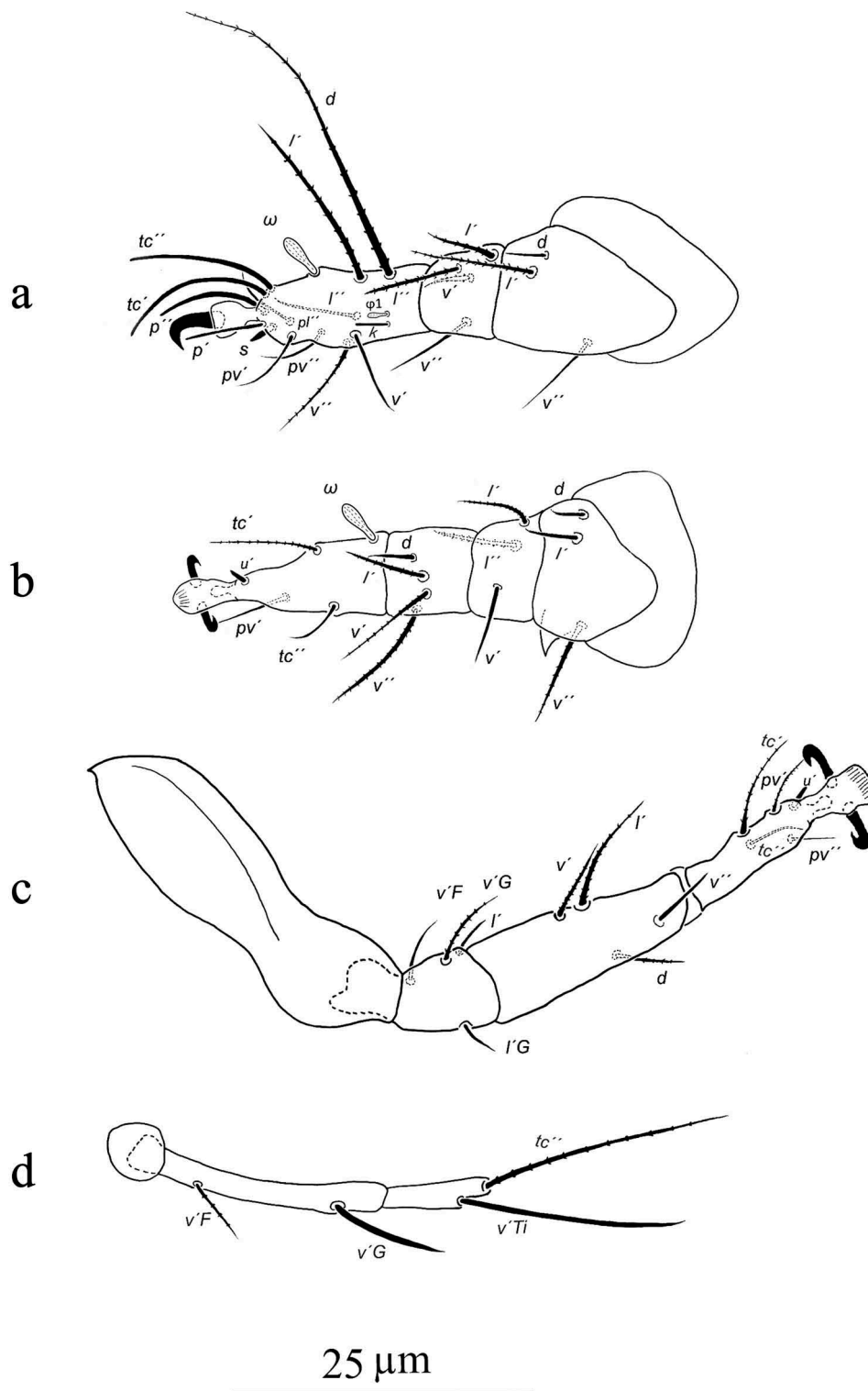
Figure 5. Excelsotarsonemus cabrucae sp. n. (female): (a) leg I, (b) leg II, (c) leg III, and (d) leg IV.
