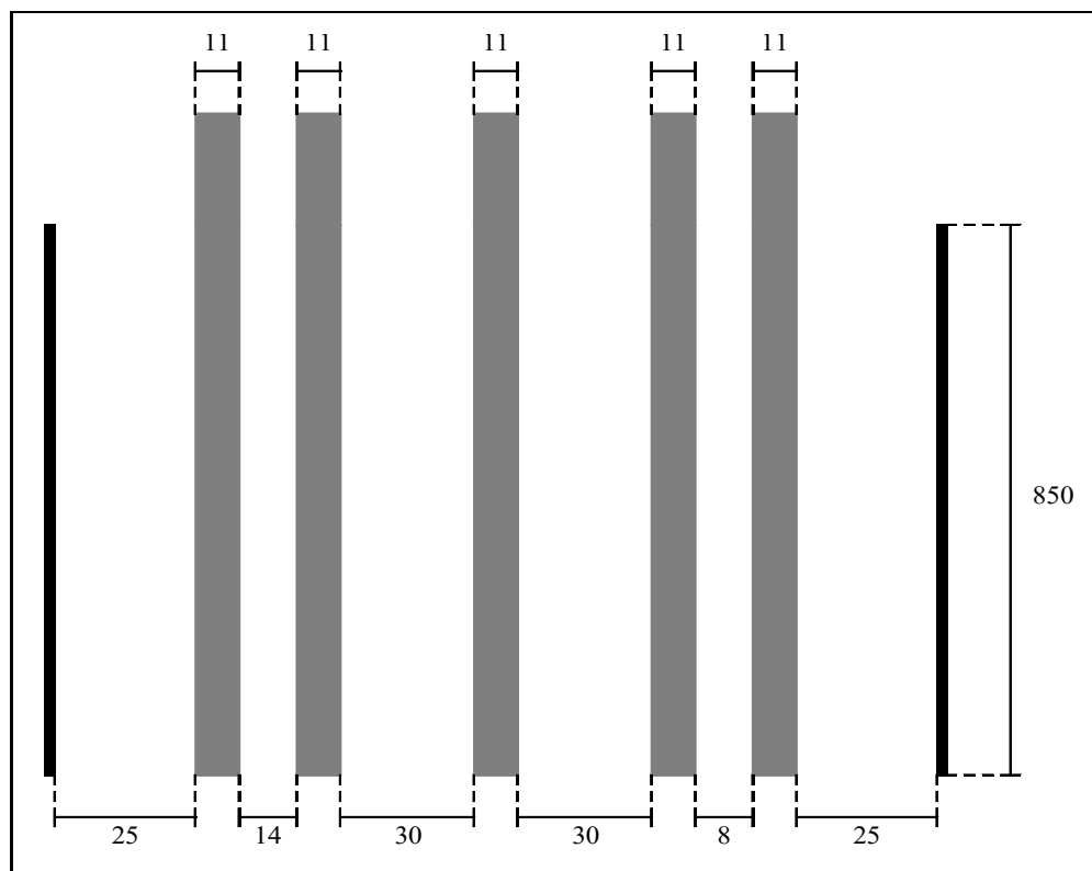
Figure 14 – Internal dimensions, in top view, of the hardening furnace (centimeters). Source: Author.
