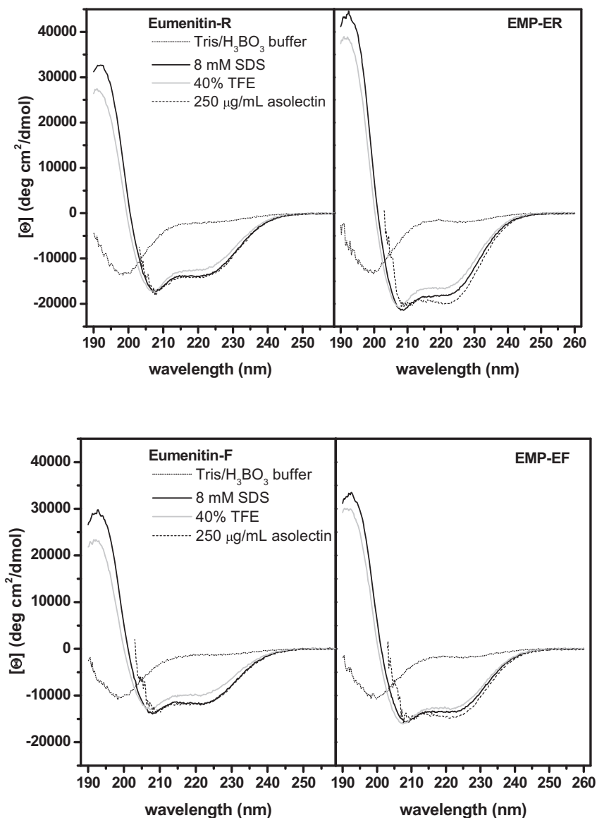
Fig. 4. CD spectra of the four peptides, eumenitin-R, EMP-ER, eumenitin-F and EMP-EF, obtained at 20 \mu M peptide concentration, at 25 °C in different environments. Peptides assume an \alpha -helical conformation in 40% TFE, 8 mM SDS and in the presence of asolectin vesicles, showing modest preference for the anionic environments of SDS micelles and asolectin vesicles.
